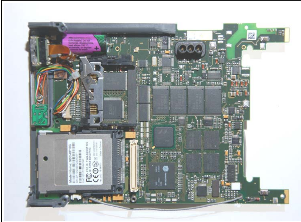
EUT PCB 1, Front
