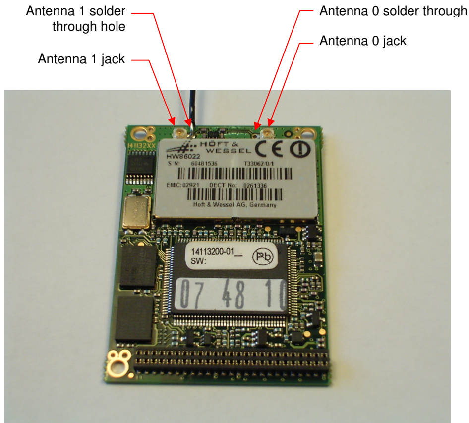
Figure 9: Antenna Ports
