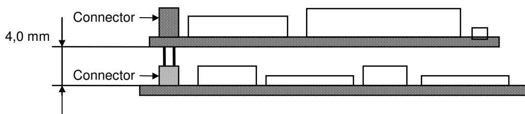
Figure 5: Components fitted on target PCB below HW 86022. Distance between PCBs depend on component heights (here: 4,0 mm)
