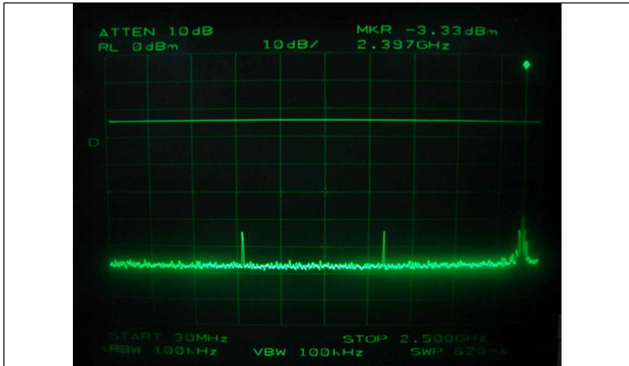
Low Channel
