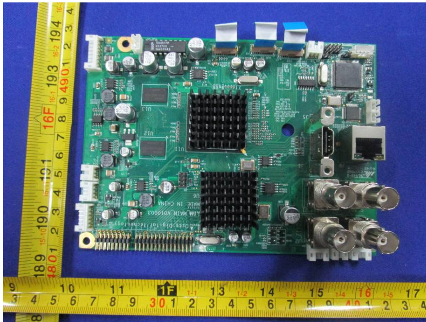
EUT –Port Board 2 Top View
