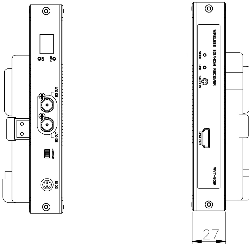
Figure 4.2-7 Side View(Unit: mm)
