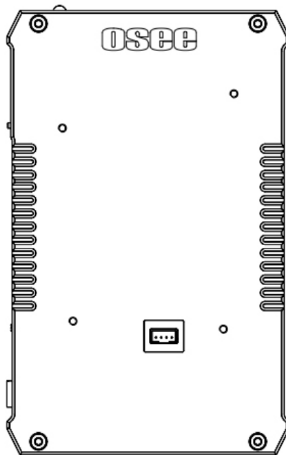
Figure 4.2-6 Back View(Unit: mm)
