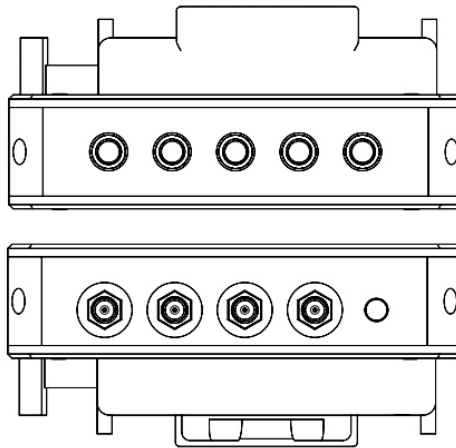
Figure 4.2-8 Top View (Unit: mm)
