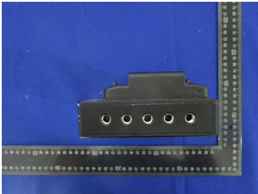
EUT – RX Side View
