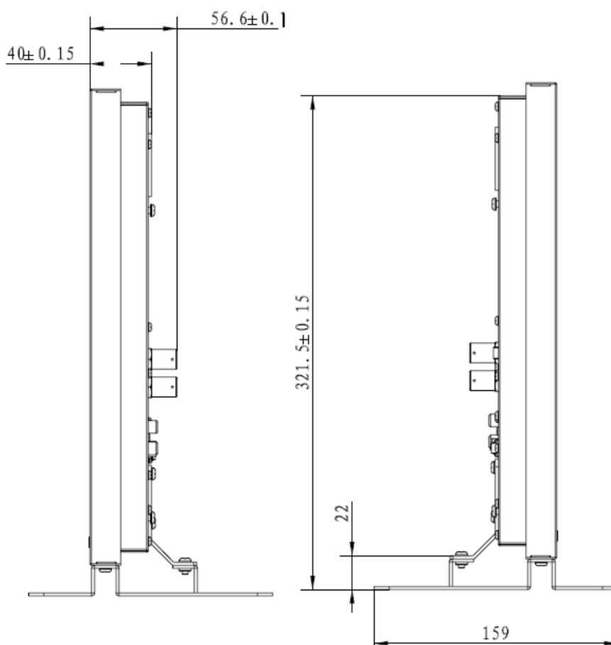
Top Side View (Unit: mm)
