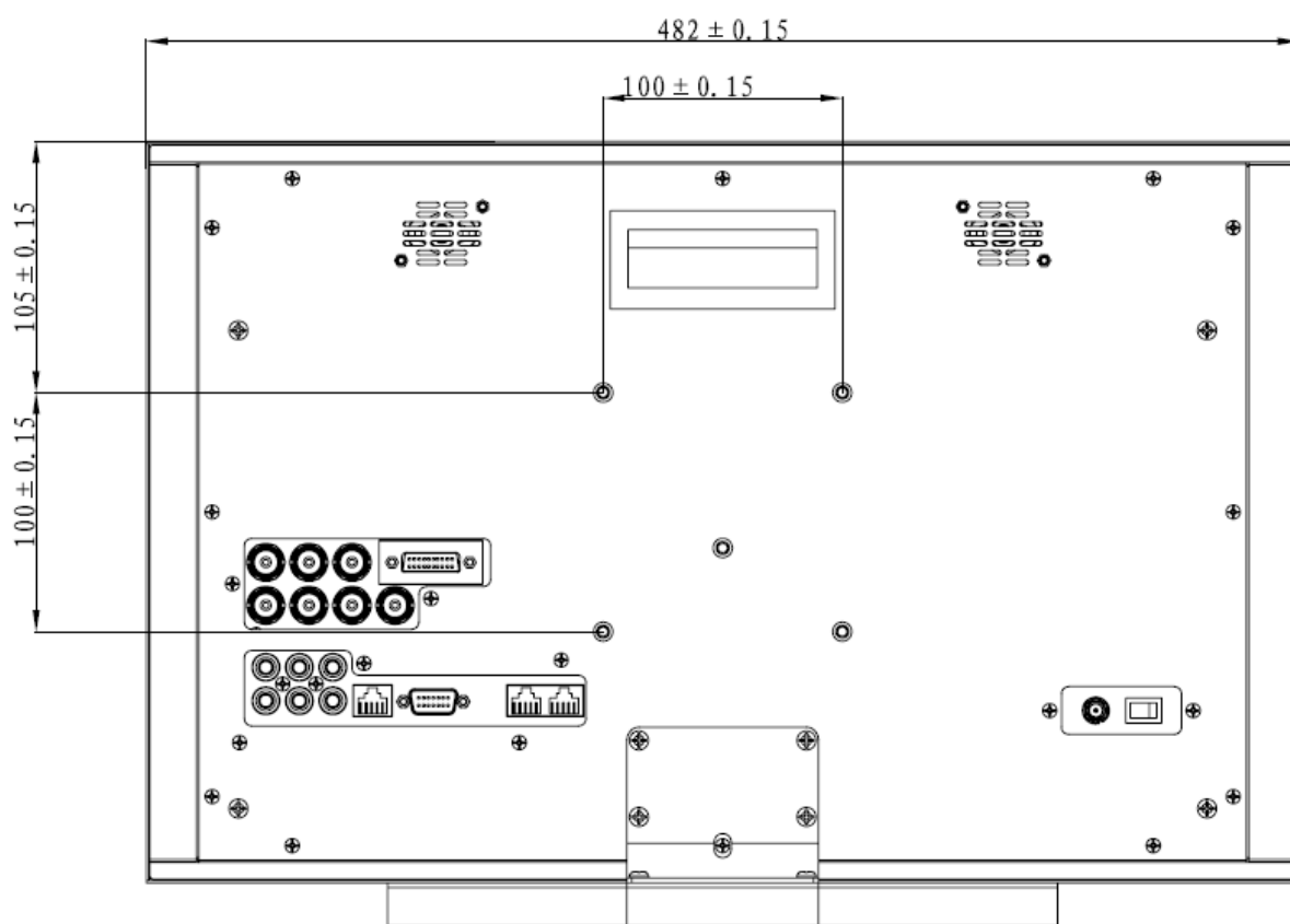
Rear View (Unit: mm)
