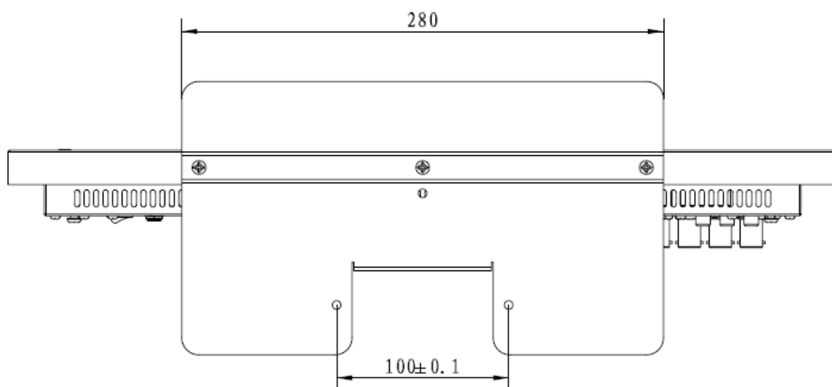
Top Side View (Unit: mm)
