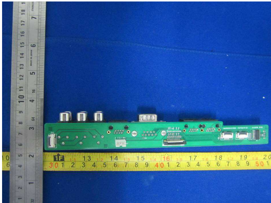
EUT –Signal Out/Input Board Bottom View
