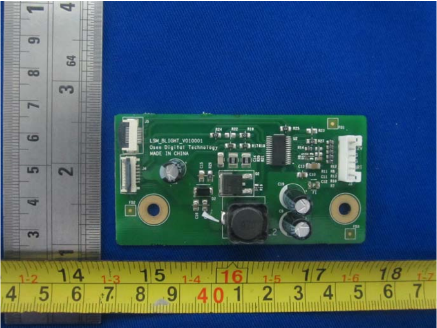
EUT- Blight Board Top View
