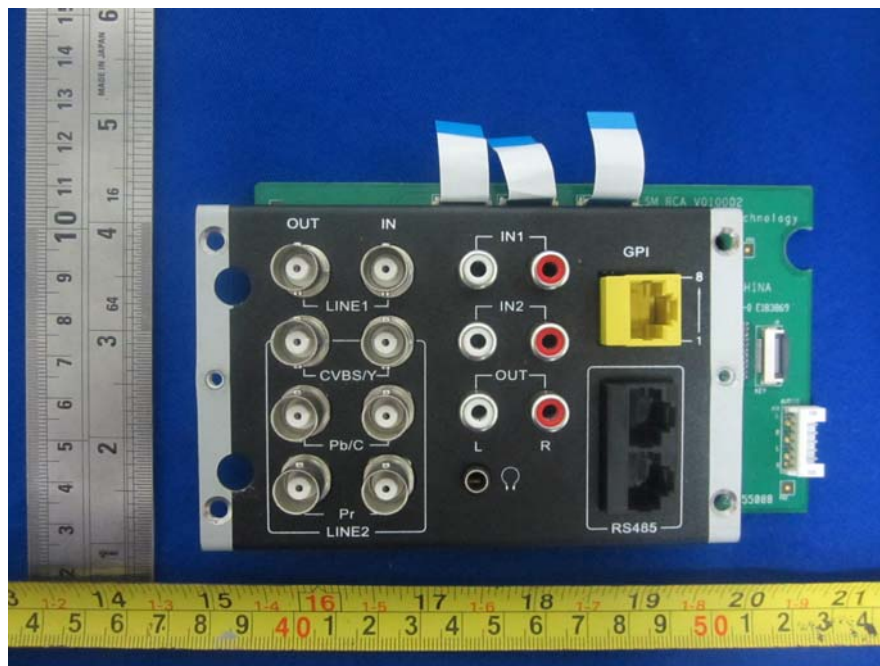
EUT- RCA Board Bottom View
