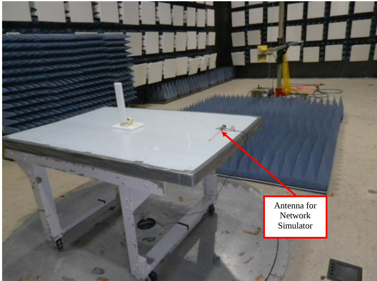
Figure 4: Typical Radiated Emissions – Above 1 GHz shown, rear view
