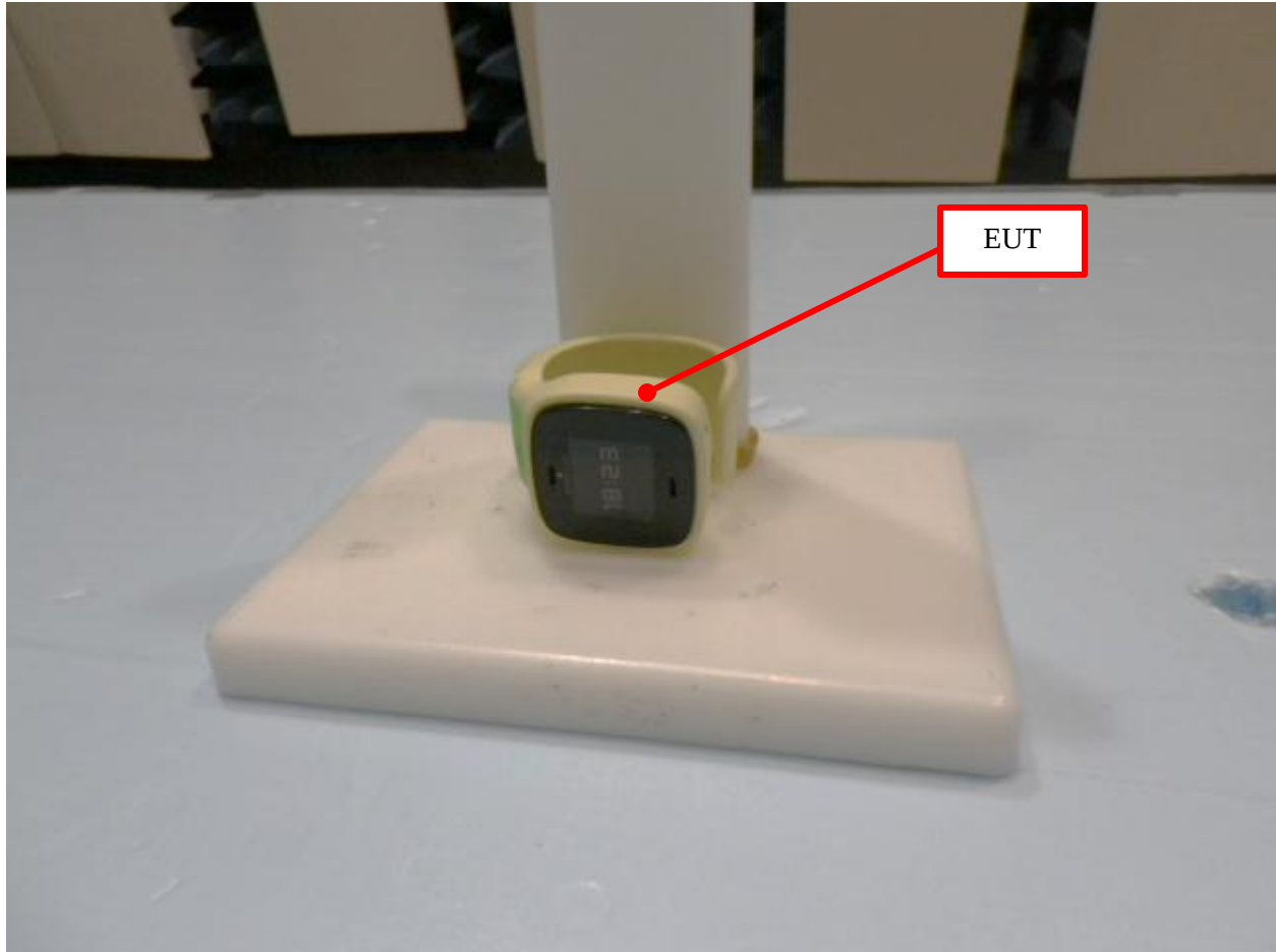
Figure 6: Radiated Emissions – Orientation A
