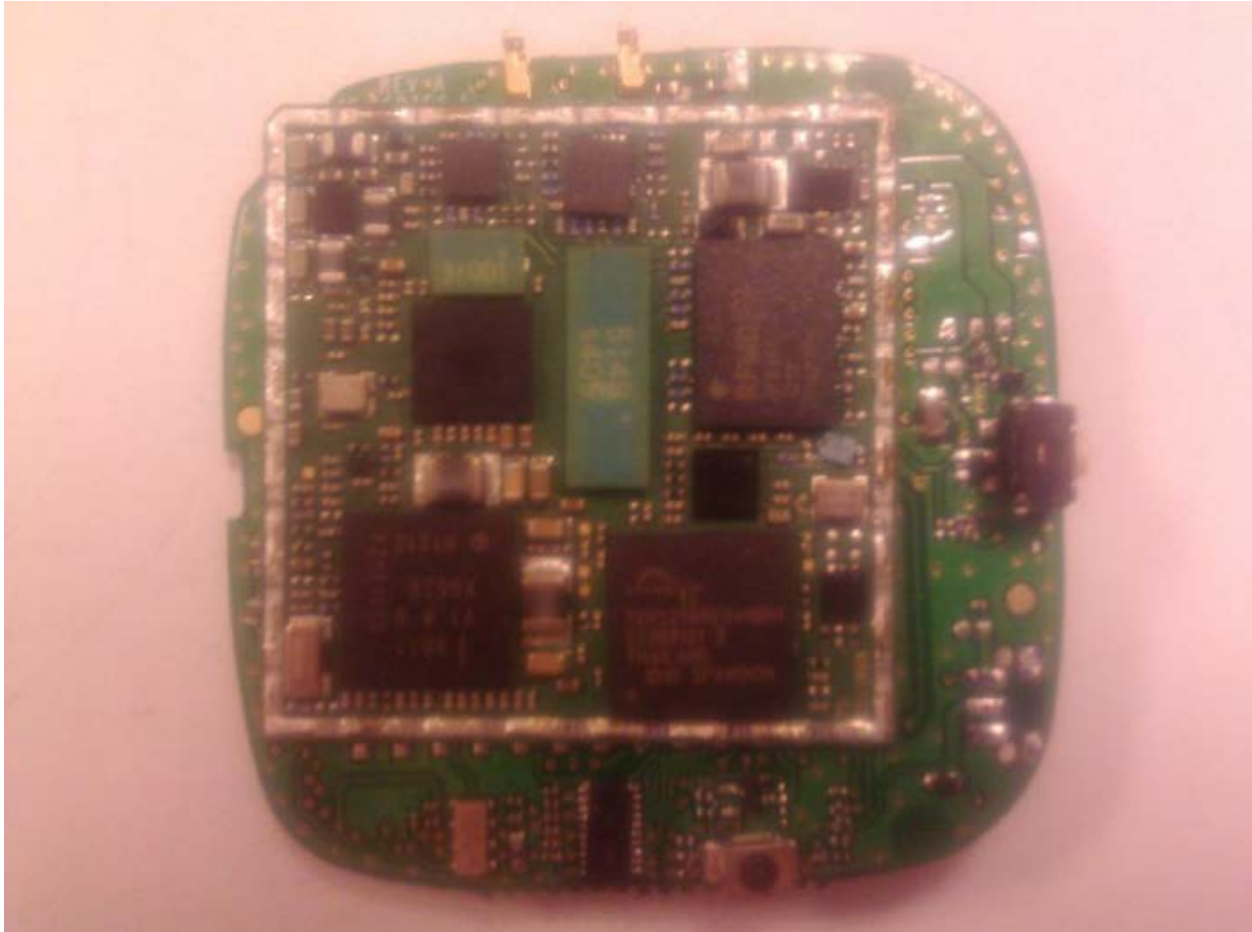
Figure 3: Internal View of circuit board w/ shield removed.
