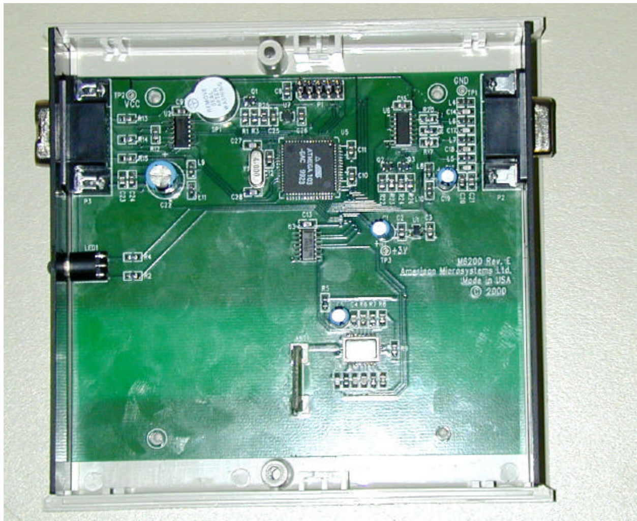
M6200 Internal photo: Component side of PCB
