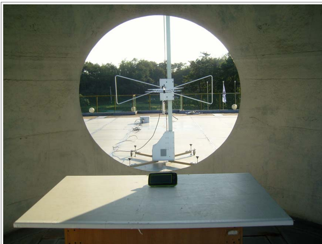
Radiated emission Test(13.56MHz)
