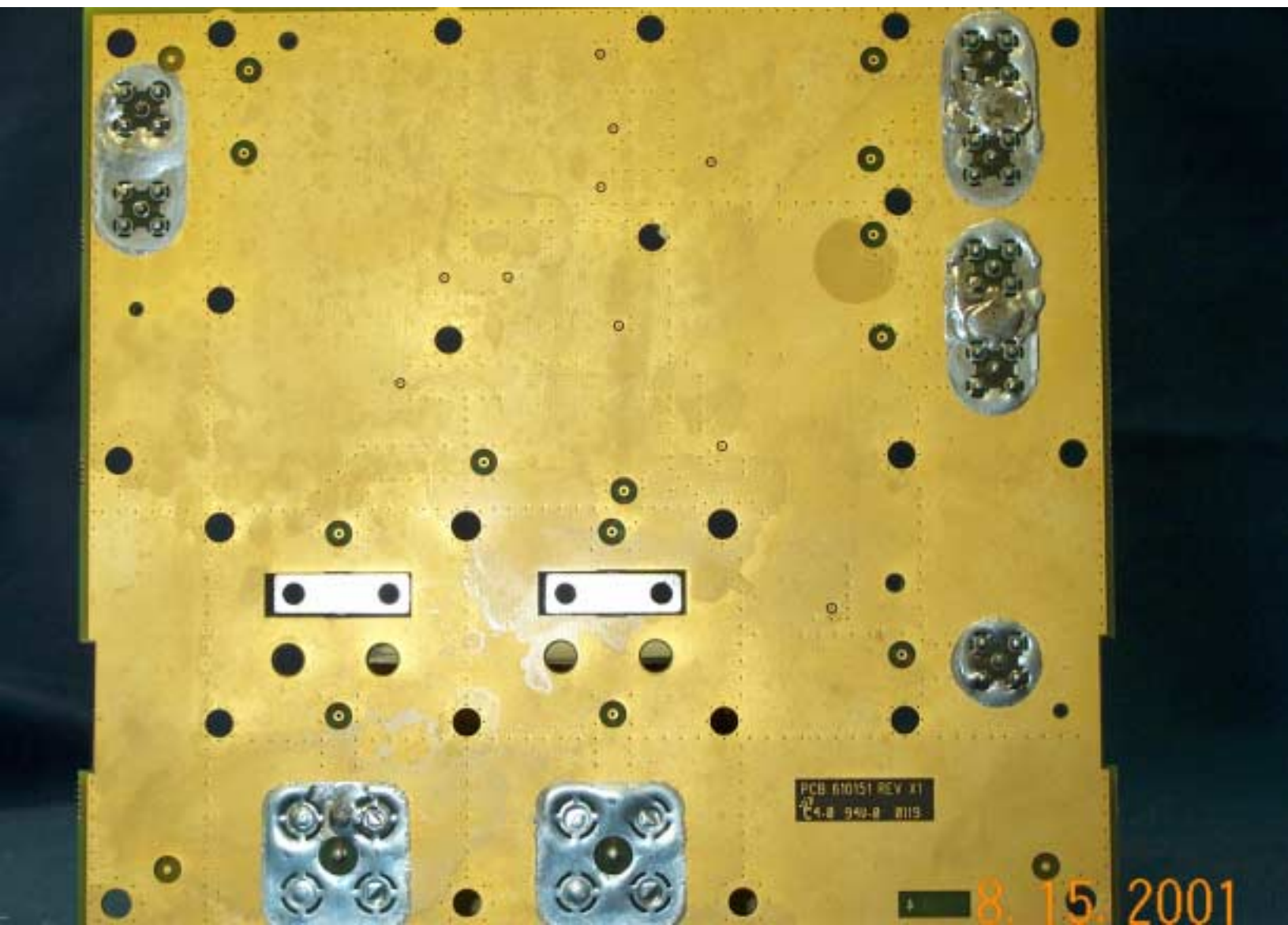
BTS INTR PWA, BACK
