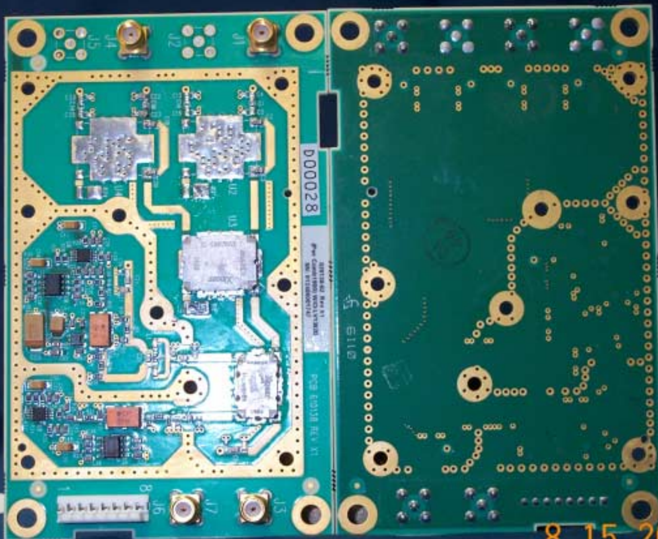
PWR COMBINER PWA FRONT/BACK
