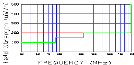
Figure 24. Restricted band harmonics and spurious limits.
