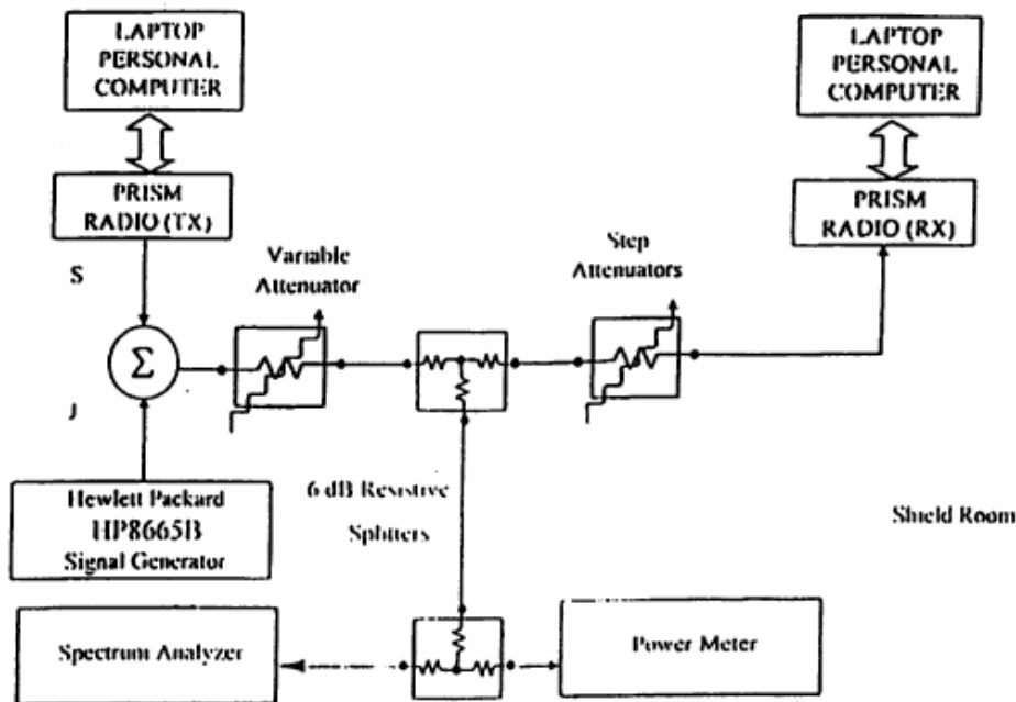
Basic Test Block Diagram
