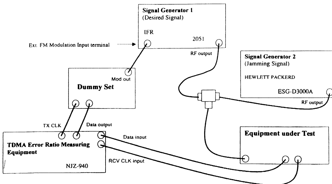
Figure 1: Processing Gain Test Setup
