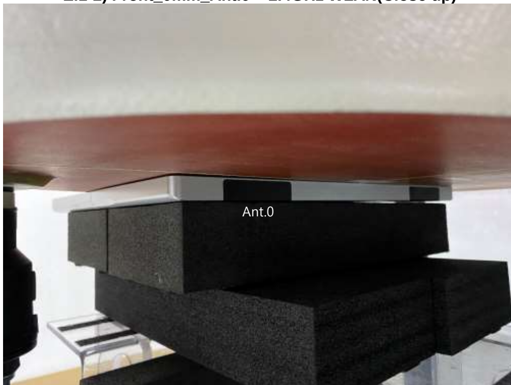
E.1-2) Front_0mm_Ant.0 – 2.4GHz WLAN(Close up)
