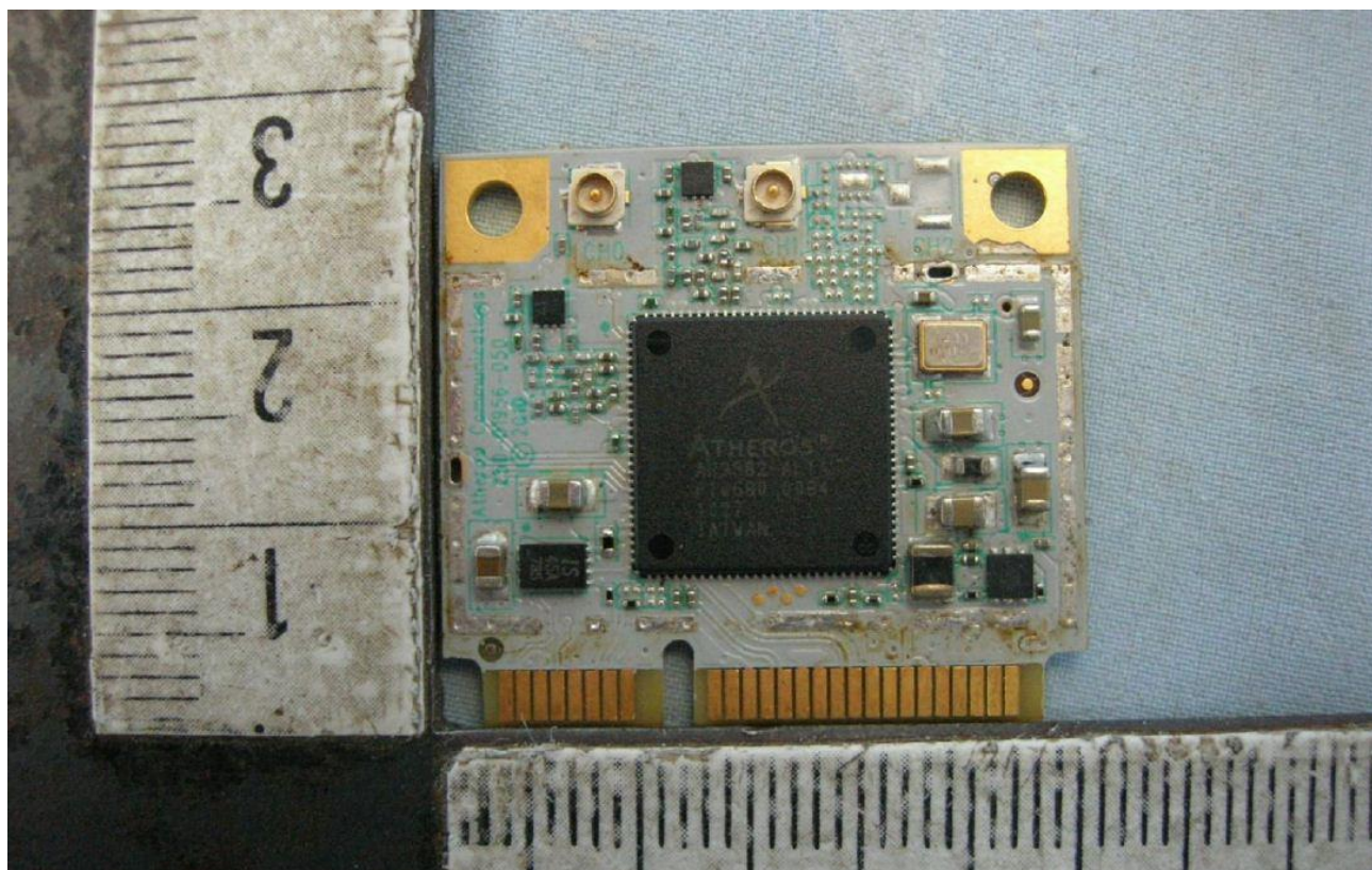
FRONT
