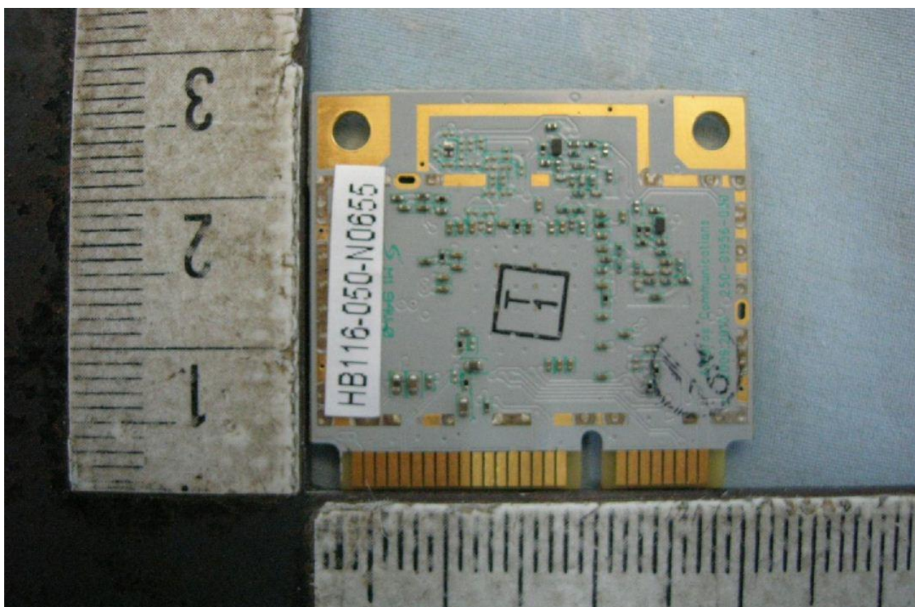
REAR
