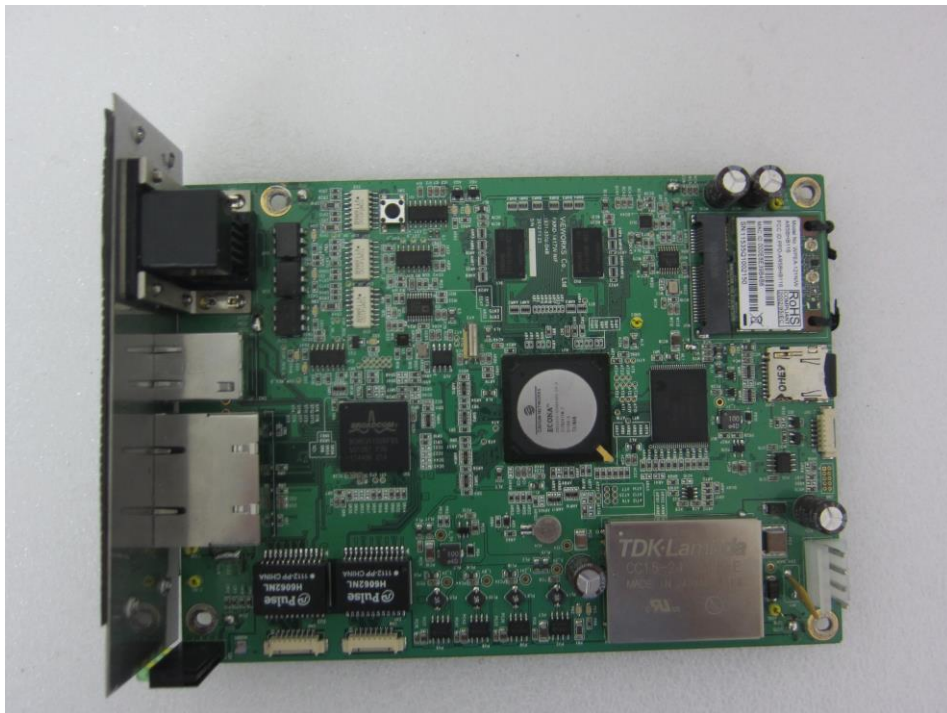
Main board_front
