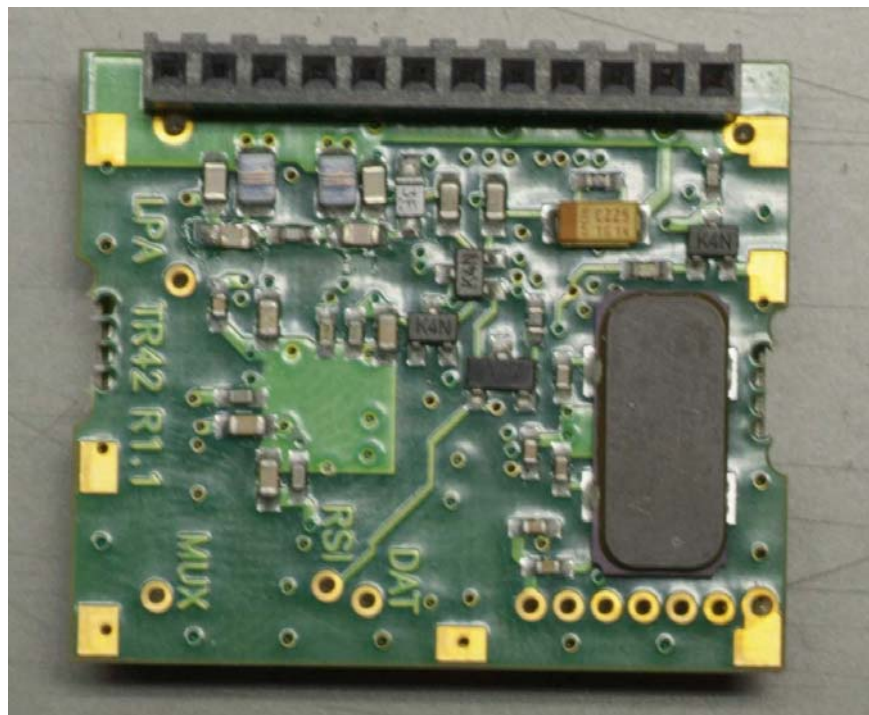
RF Module PCB Bottom View
