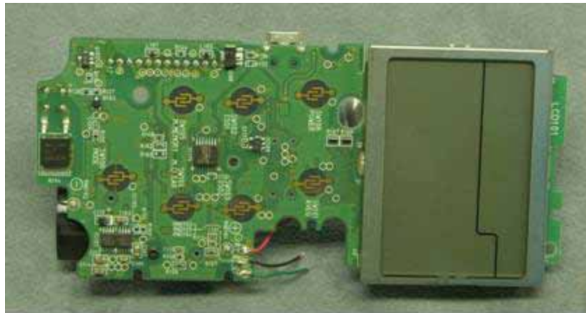
PCB 1 Top View
