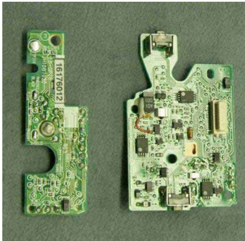
PCB 2&3 Top view
