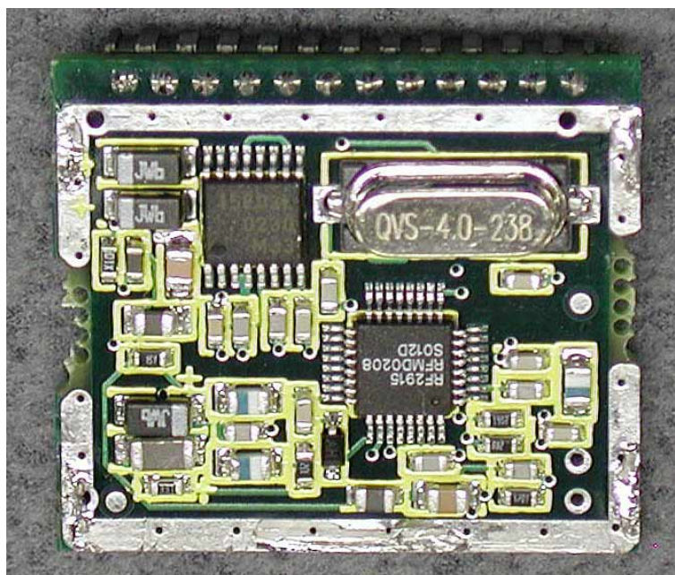
RF Module PCB Top View
