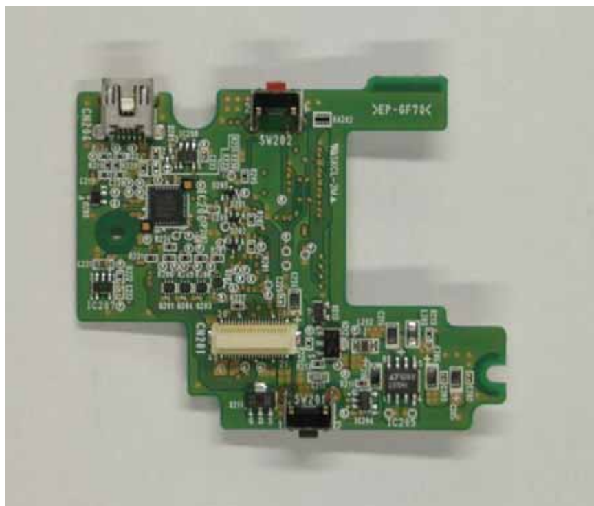
PCB 2 Bottom View
