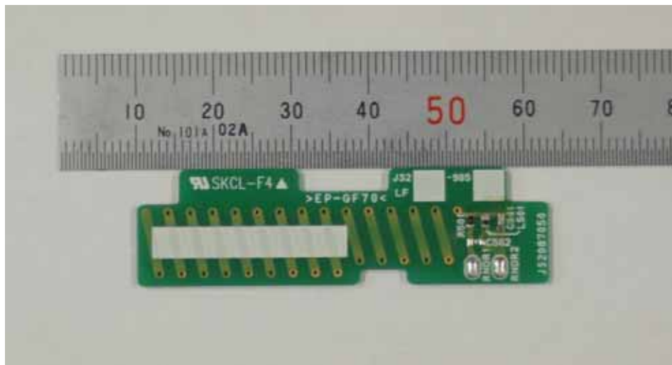
PCB 5 Top View
