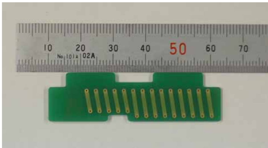
PCB 5 Bottom View
