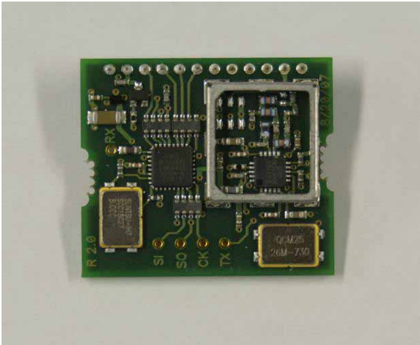
RF Module PCB Top View
