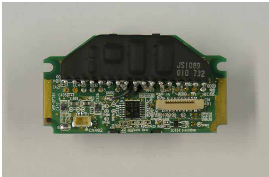
PCB 4 Top View
