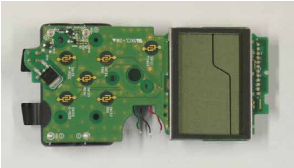
PCB 1 Top View
