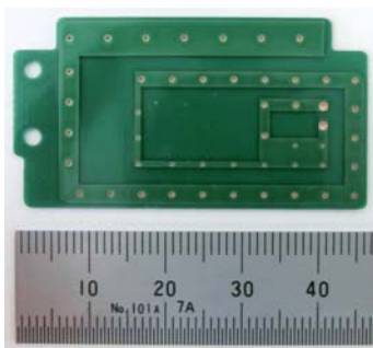
PCB 4 (Antenna) Bottom View
