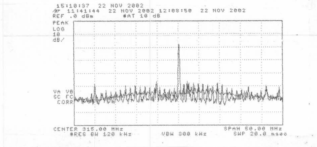
Figure 6.1. Relative receiver emissions in stand-by and "locked-in" modes. The final emission measurements were made with the receiver in "locked-in" mode.
