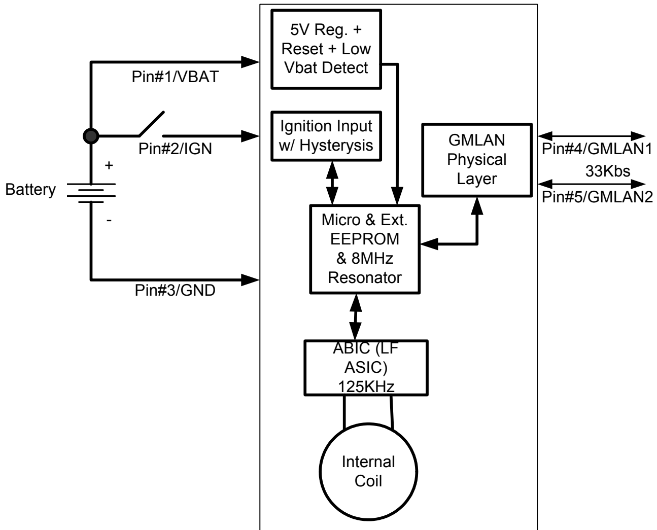
PK3+ Block & Detailed Functional Diagram
