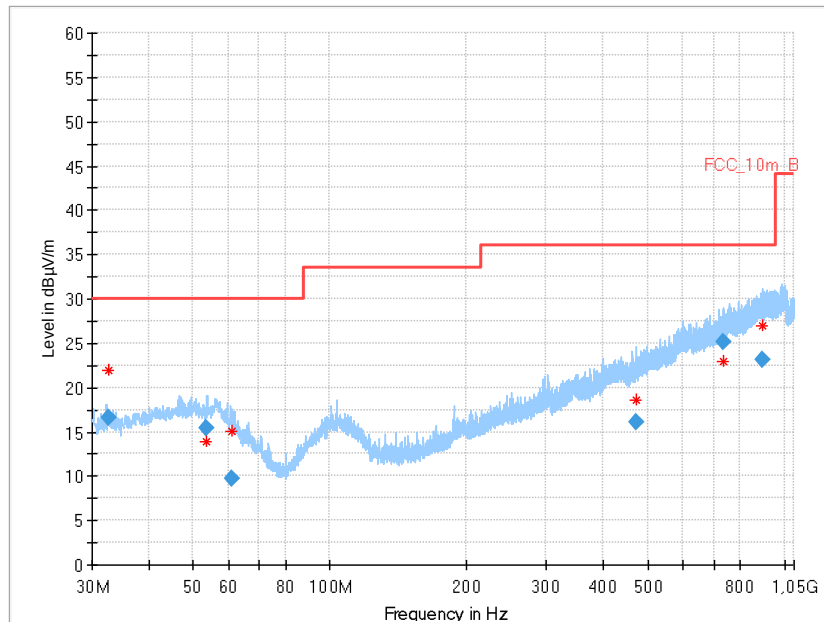
Plot 10: 30 MHz to 1 GHz, CH 9
