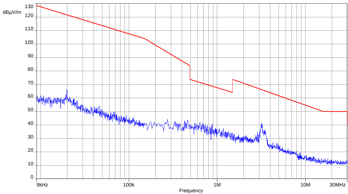
Plot 8: 9 kHz to 30 MHz, CH 9
