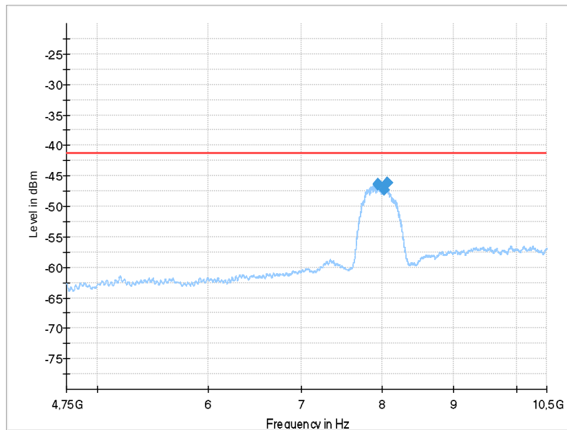
Plot 6: Peak fundamental emission, CH 9
