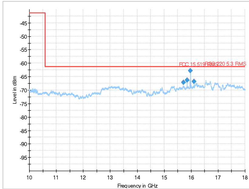
Plot 16: 10 GHz to 18 GHz, CH 9
