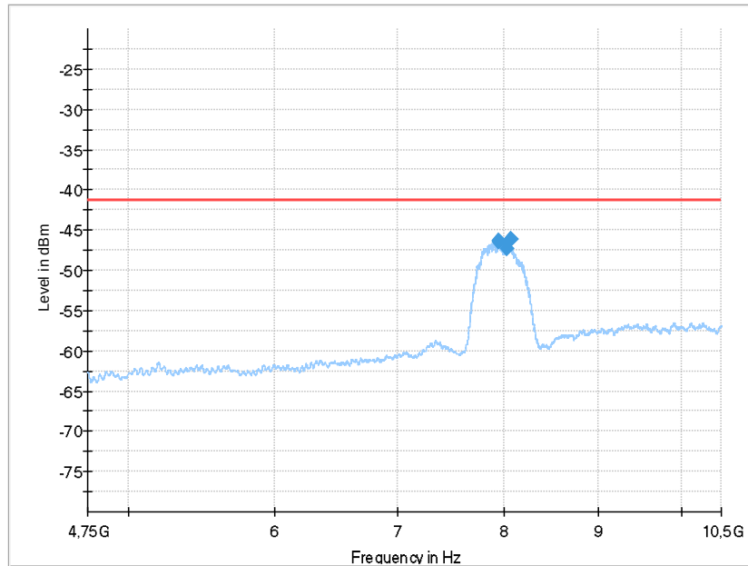
Plot 14: 4.75 GHz to 10.5 GHz, CH 9
