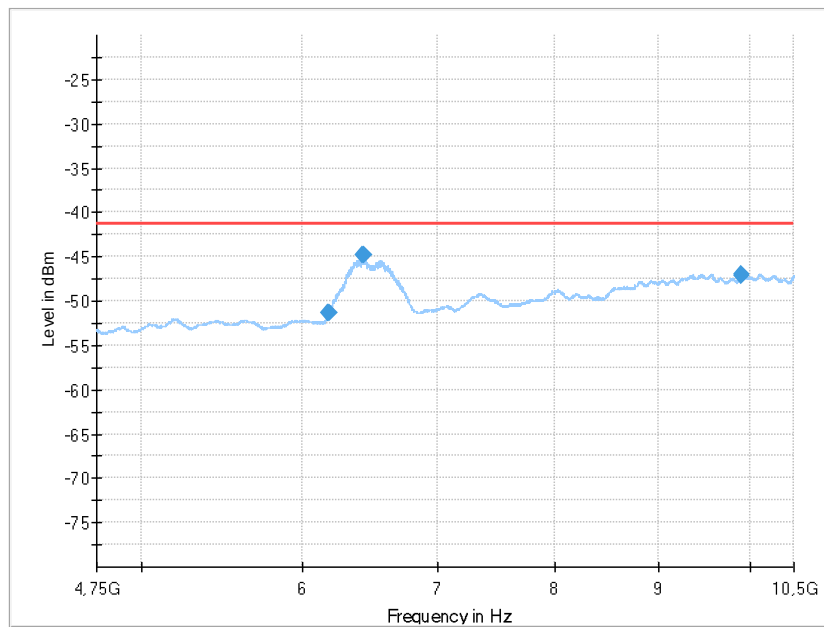
Plot 13: 4.75 GHz to 10.5 GHz, CH 5
