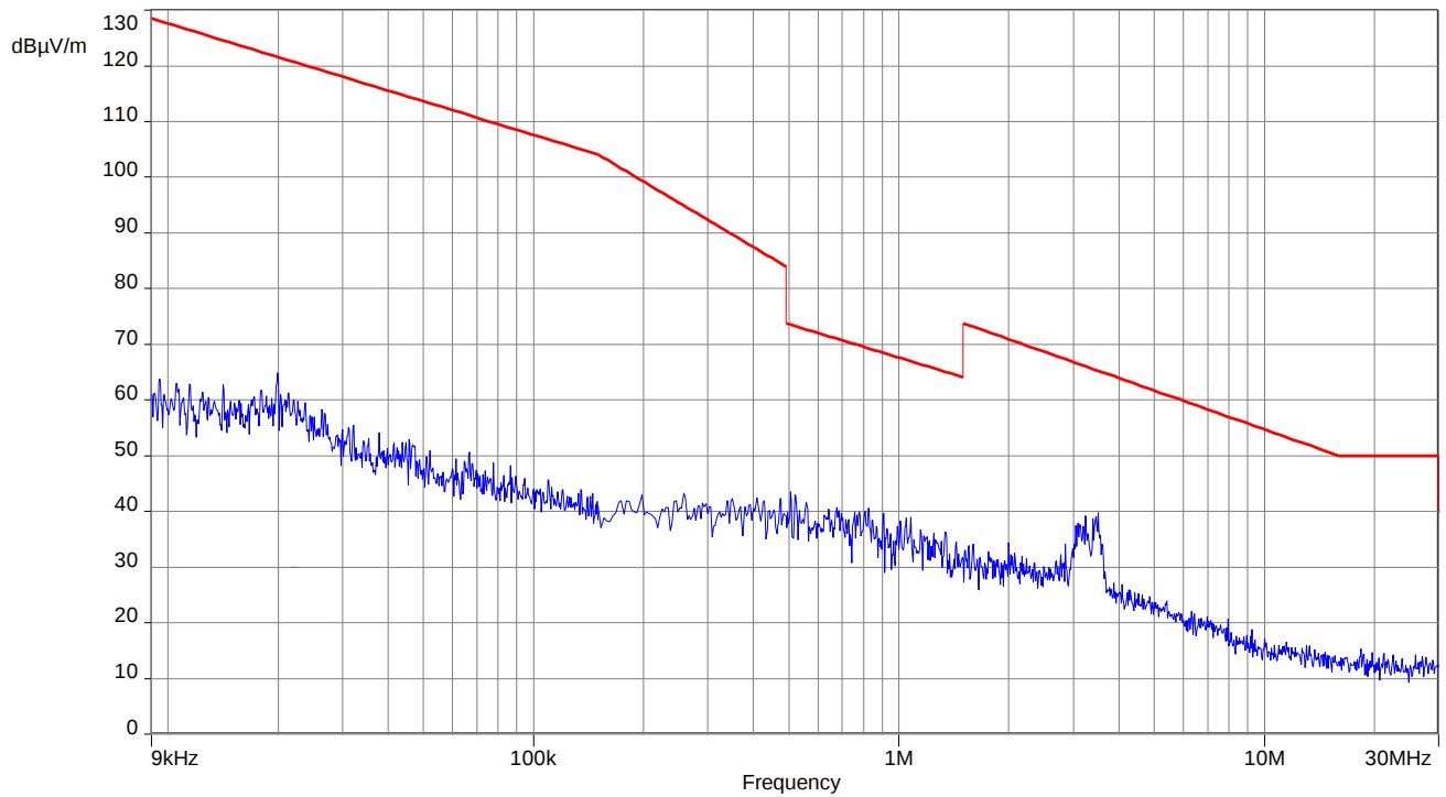
Plot 8: 9 kHz to 30 MHz, CH 9
