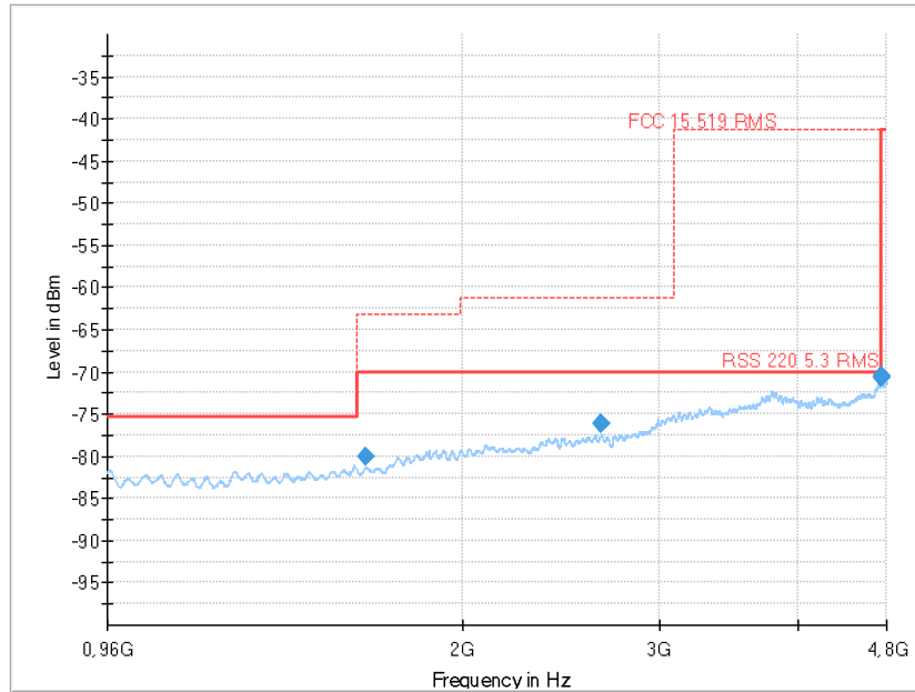
Plot 11: 960 MHz to 4.8 GHz, CH 5
