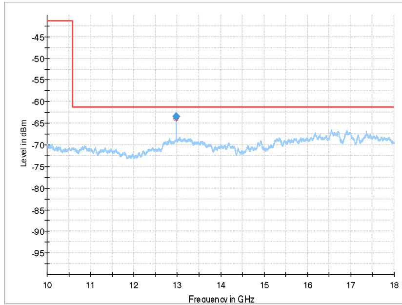
Plot 15: 10 GHz to 18 GHz, CH 5
