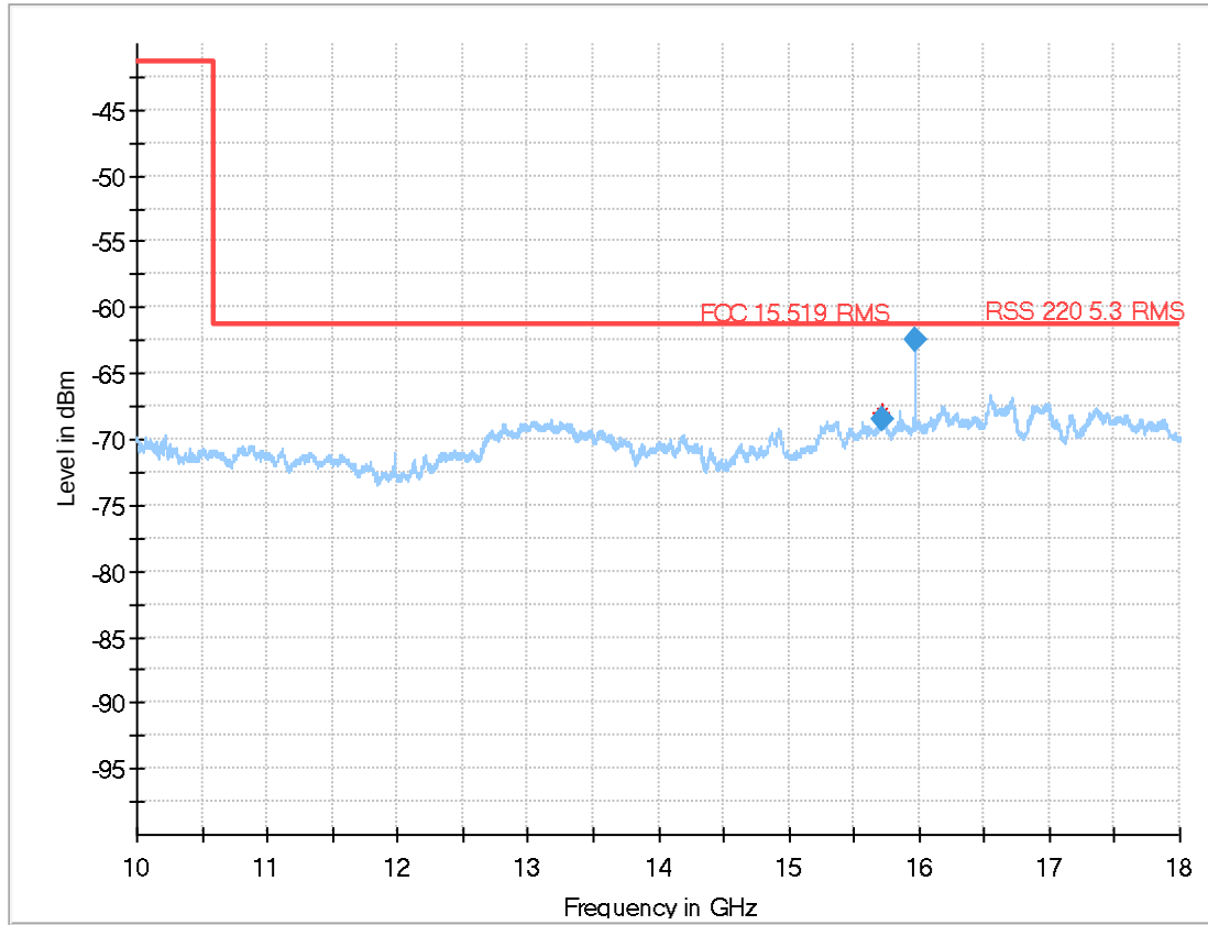
Plot 16: 10 GHz to 18 GHz, CH 9
