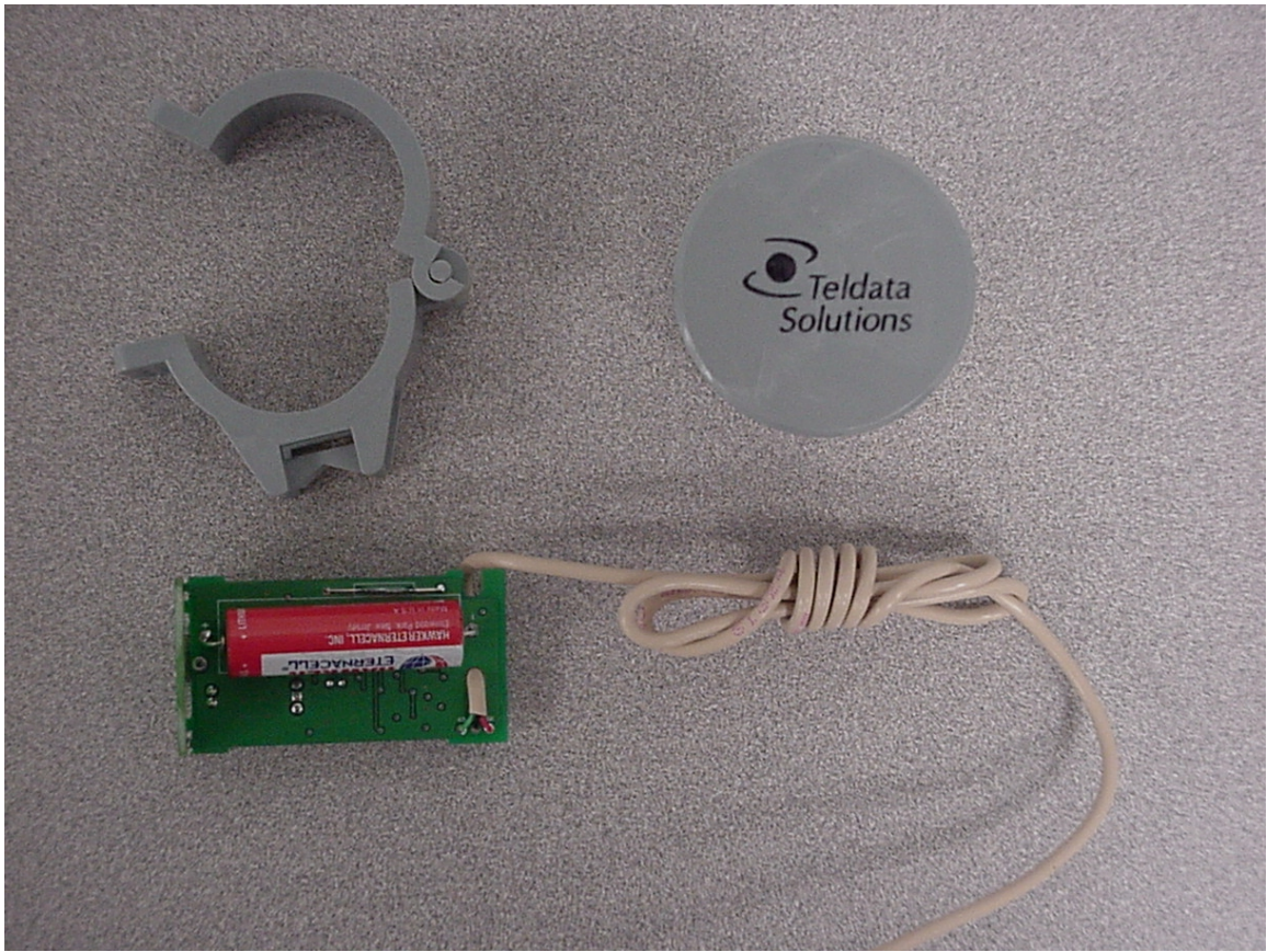
Transmitter, battery side with top view of enclosure and clamp.
