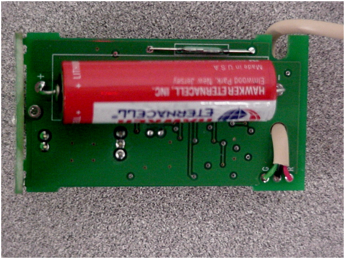
Transmitter, Close-up Battery side.
