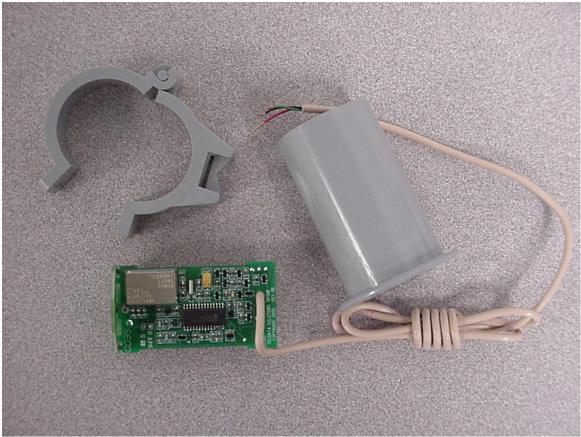
Transmitter, component side with side view of enclosure and clamp.
