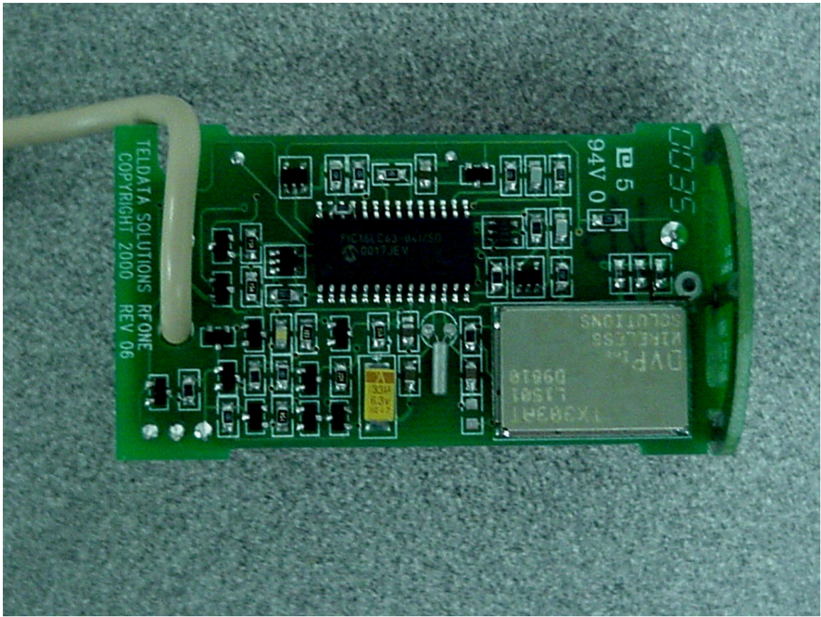
Transmitter, Close-up of component side.
