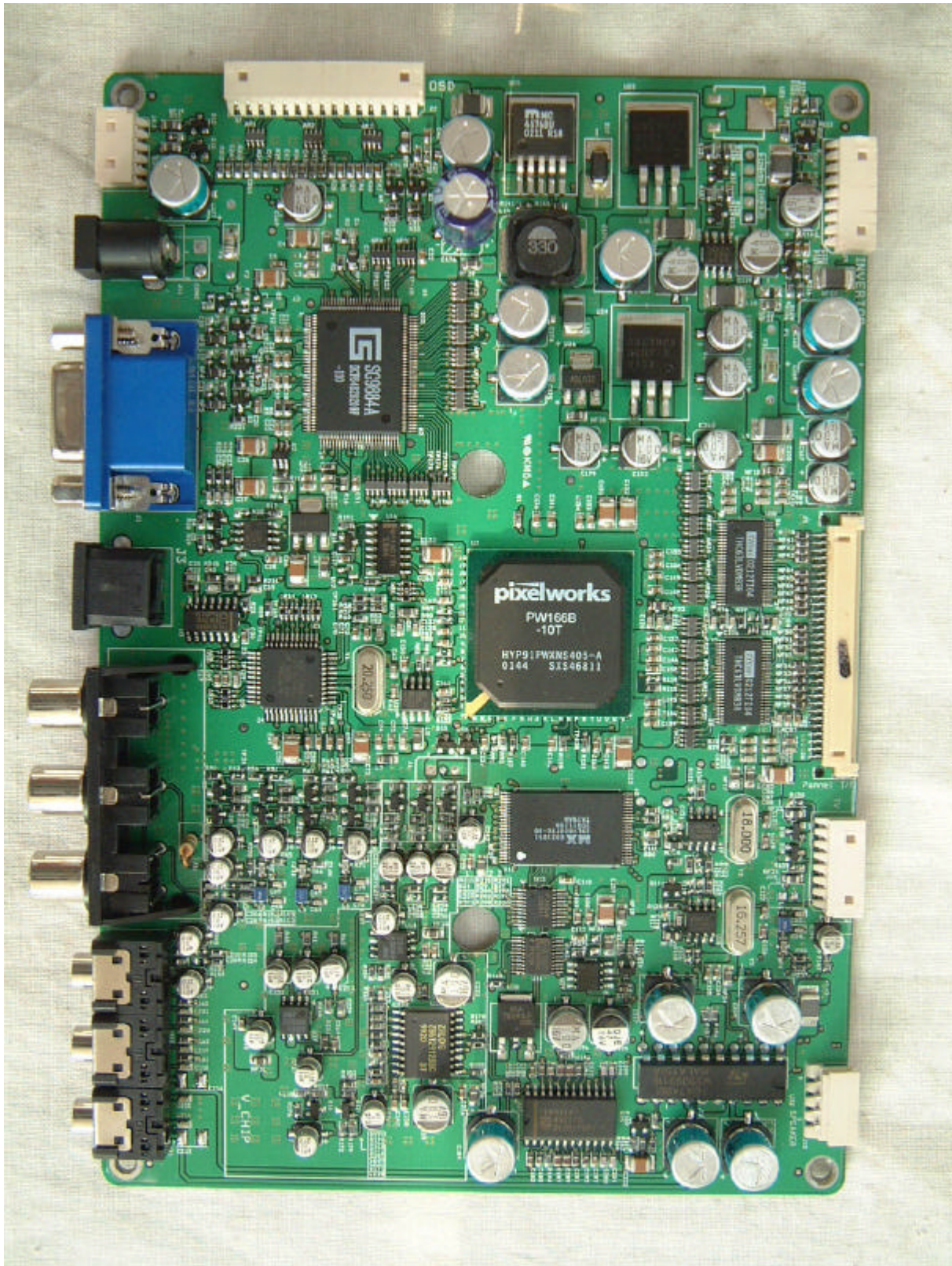
<FRONT VIEW OF MAIN BOARD>
