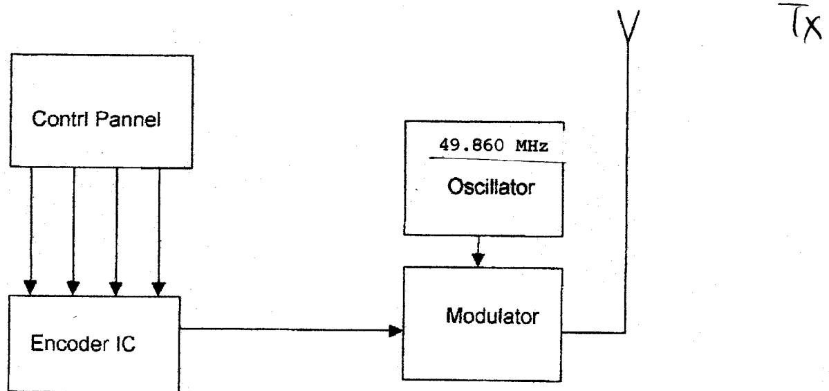
Block Diagram : Remote Control.
