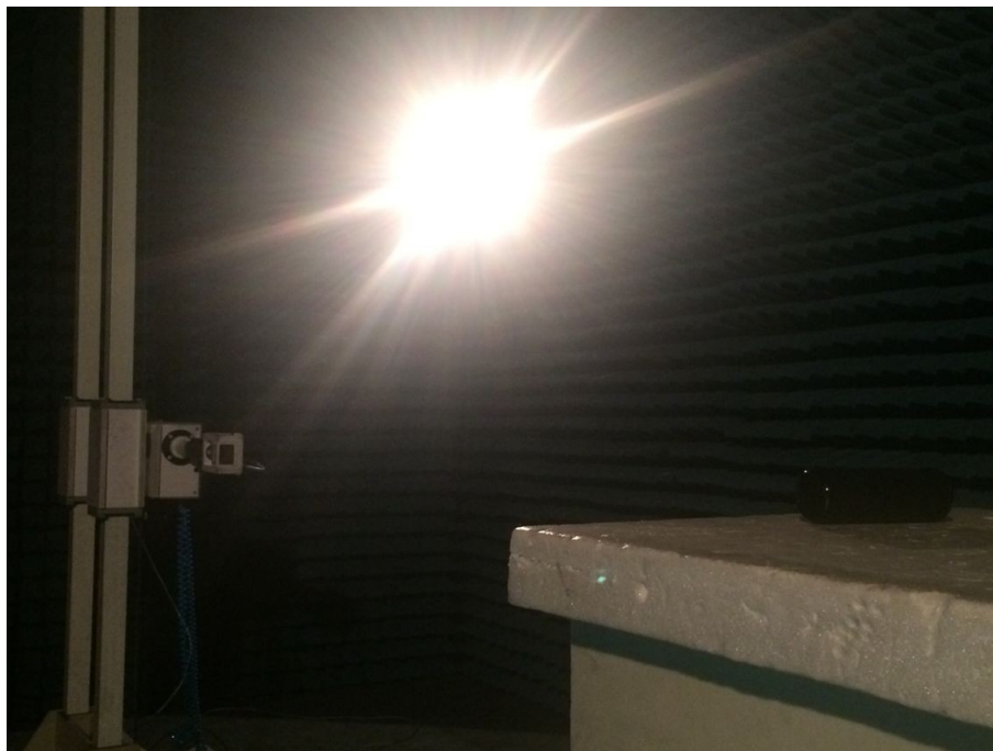
Radiated Emission test view (18GHz to 26.5GHz)
