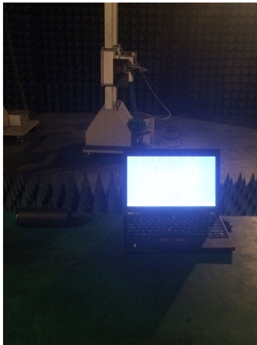
Radiated Emission test view (Frequency above 1GHz)
