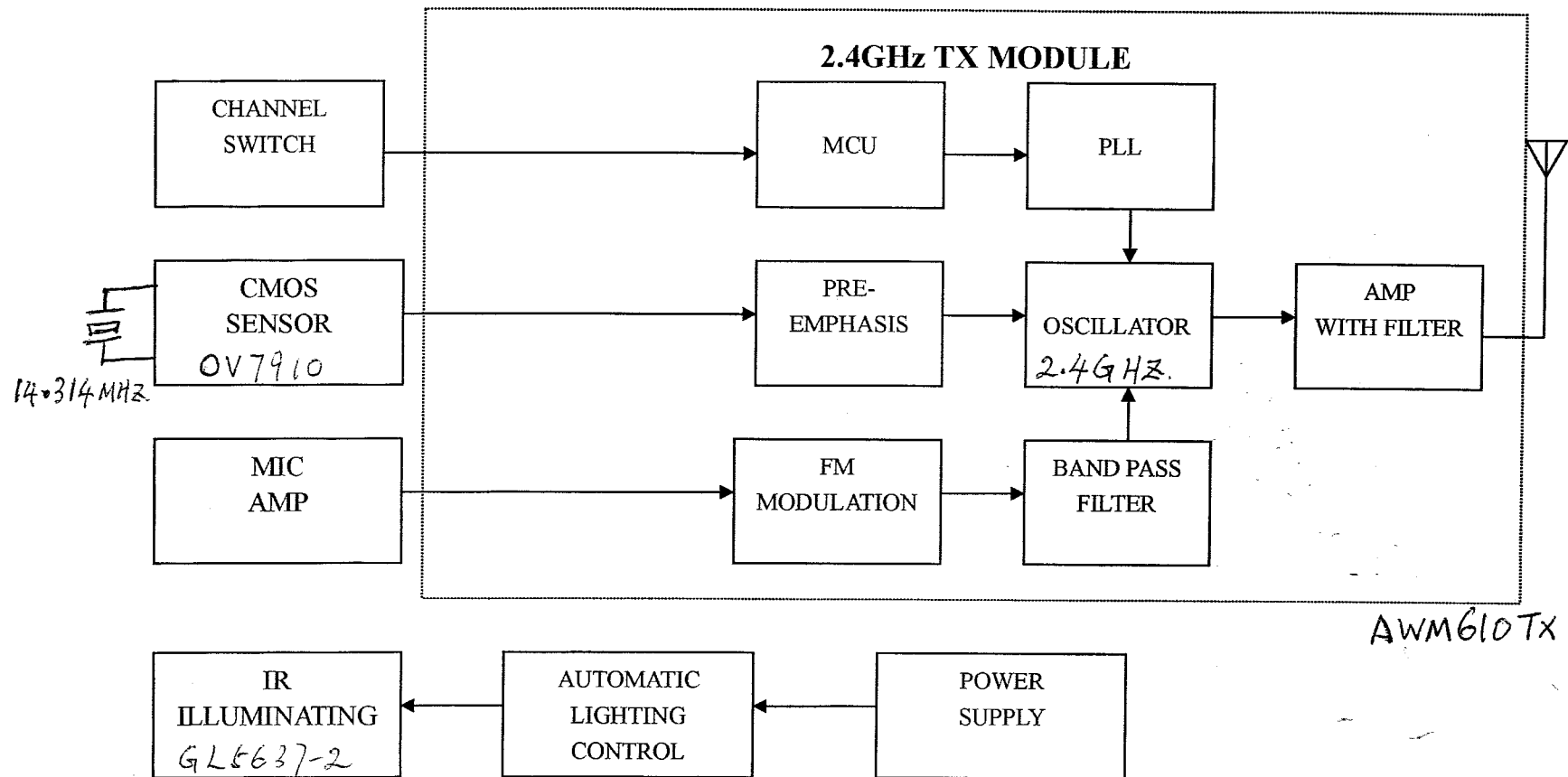
BM242 TX BLOCK DIAGRAM
