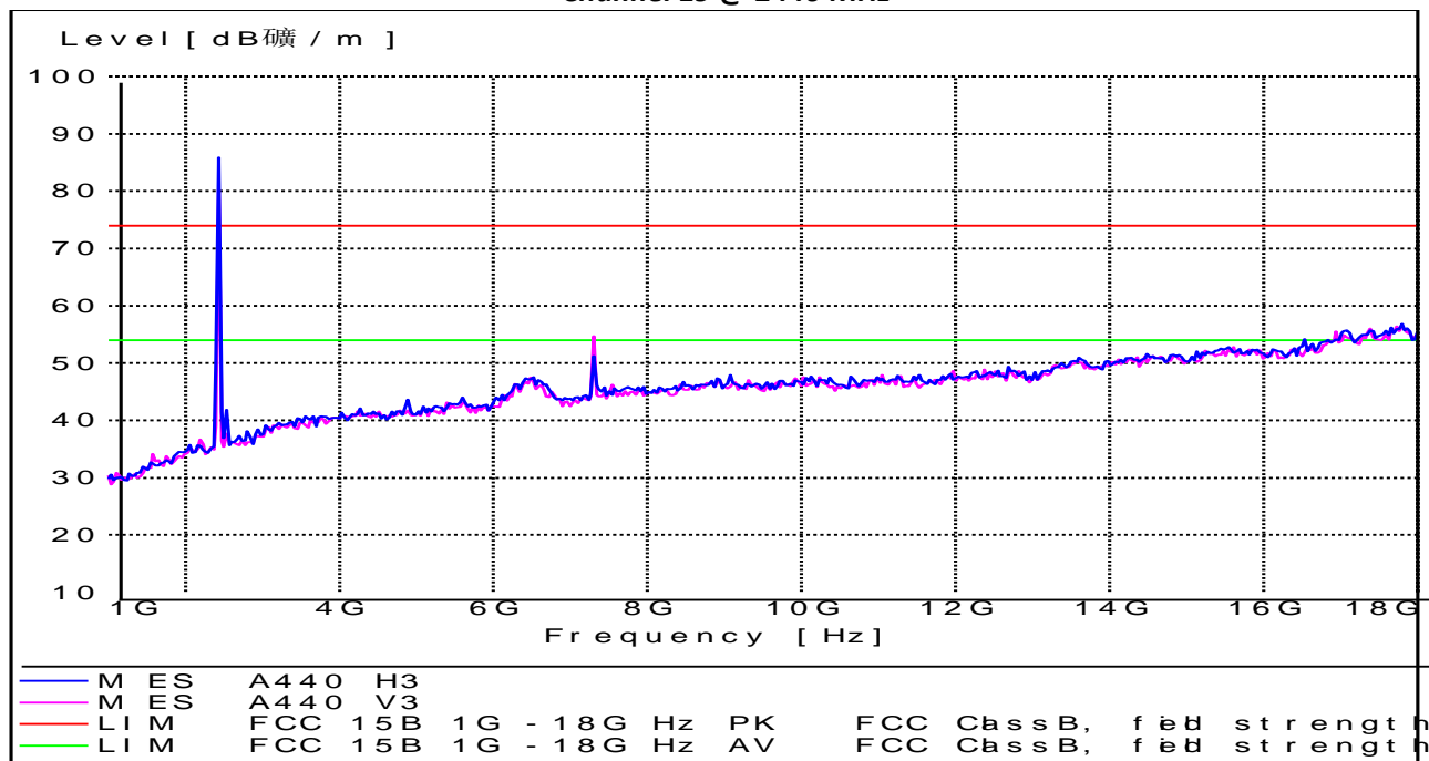
Channel 19 @ 2440 MHz
