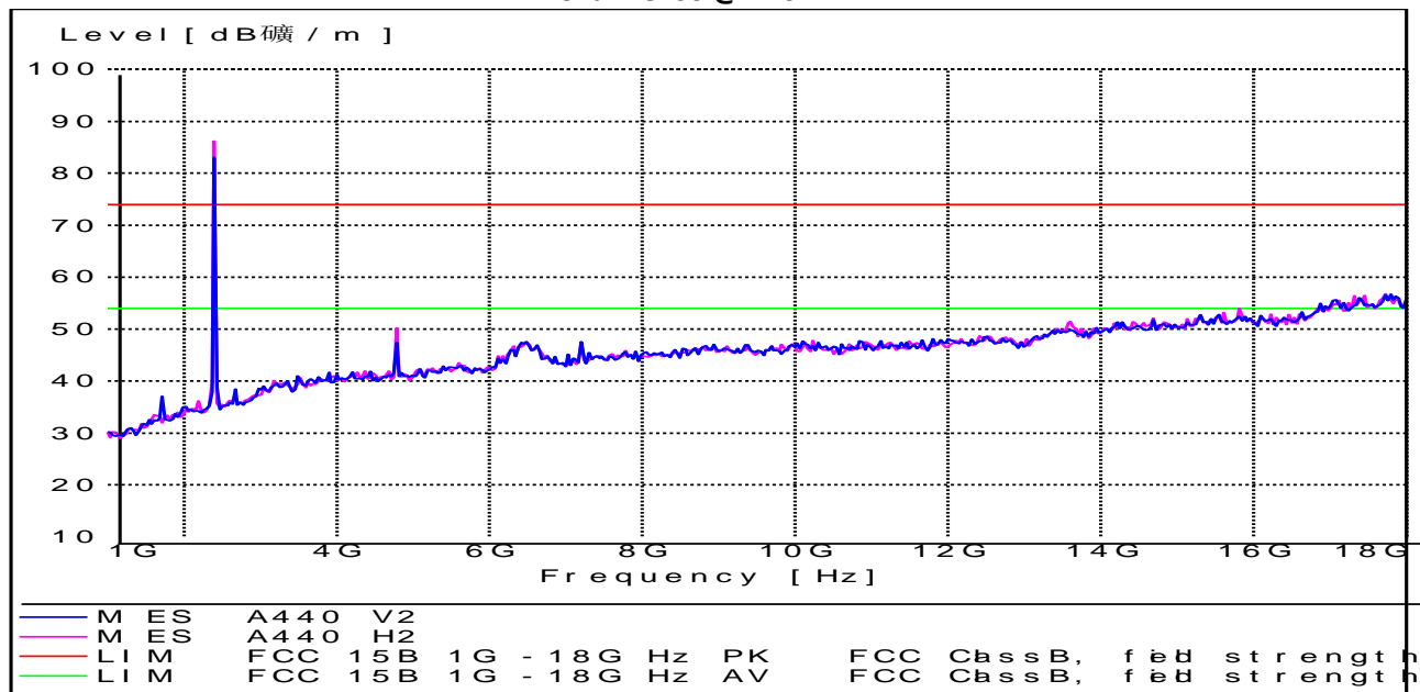
Channel 00 @ 2402 MHz
