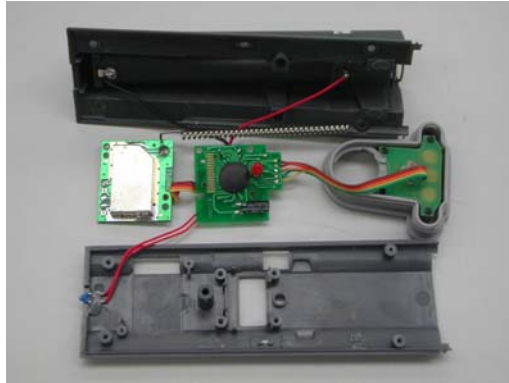
Internal Photo - 2
