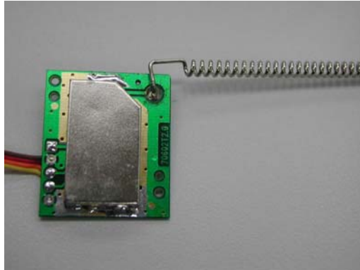
Internal Photo – 6
