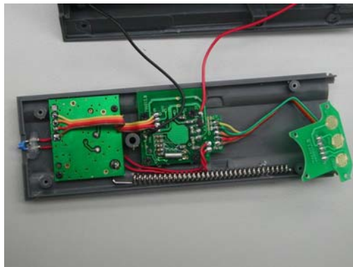
Internal Photo - 2
