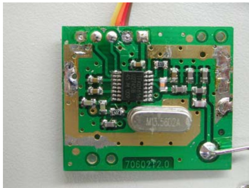
Internal Photo – 6
