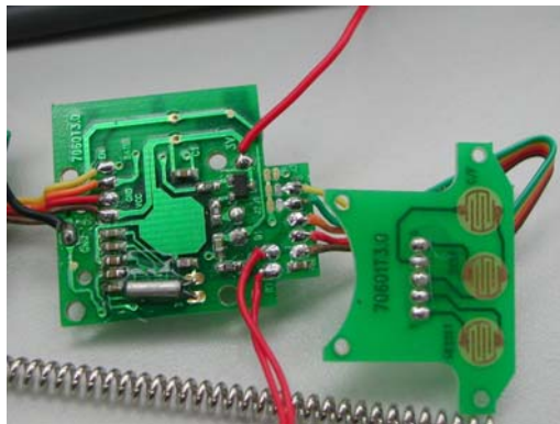
Internal Photo – 4
