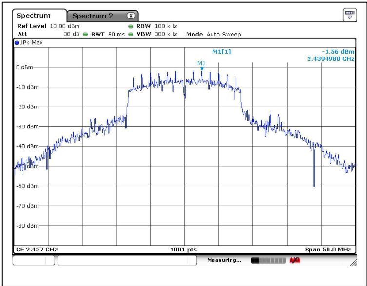
802.11g CH6
