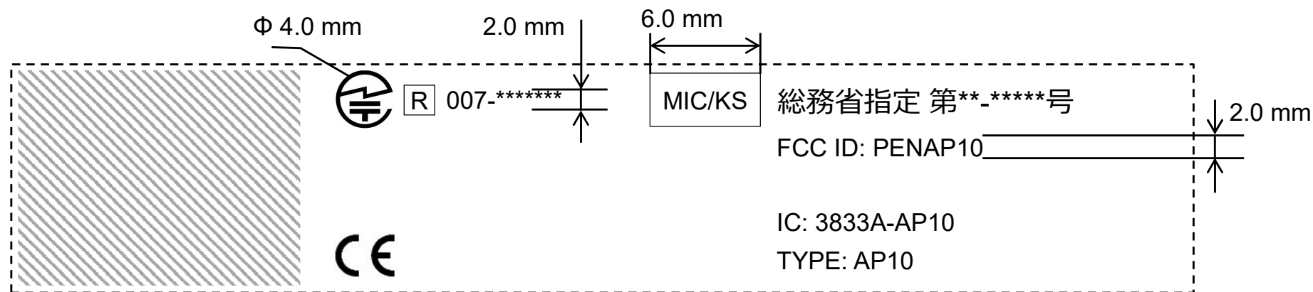
Figure 11 Marking information
