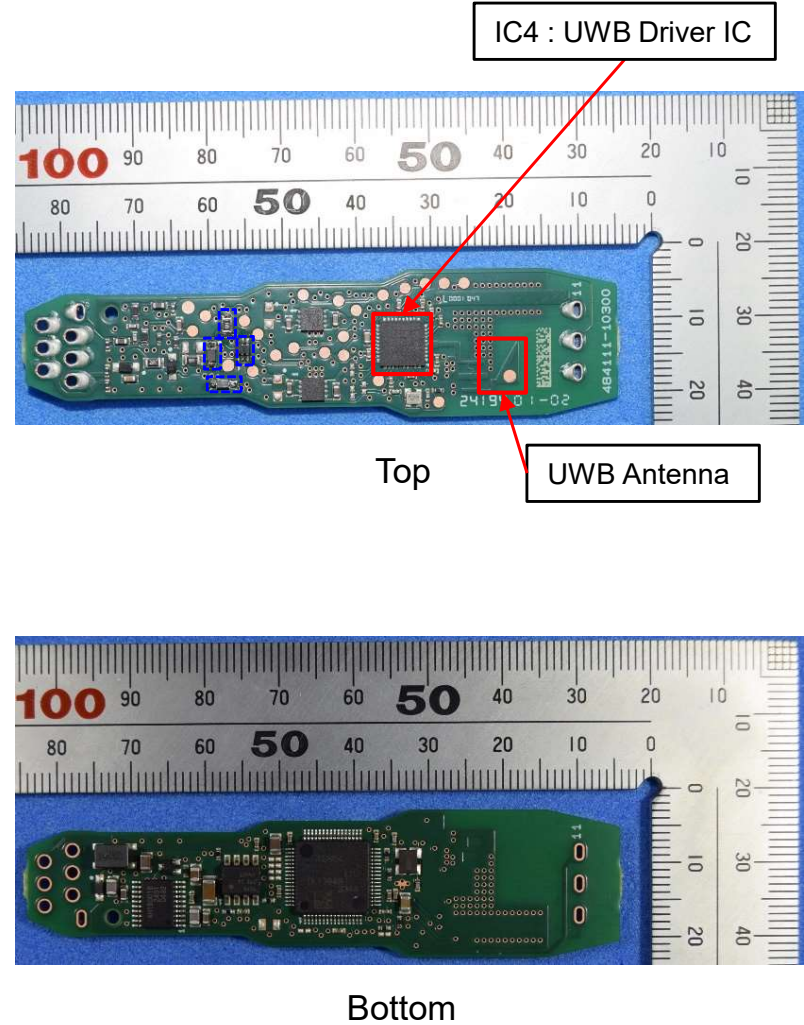
Figure 9 PCB (with SW)
