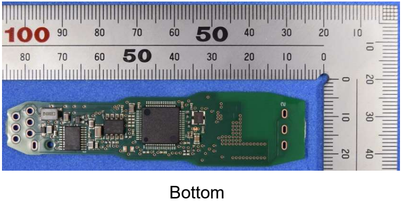
Figure 10 PCB (without SW)
