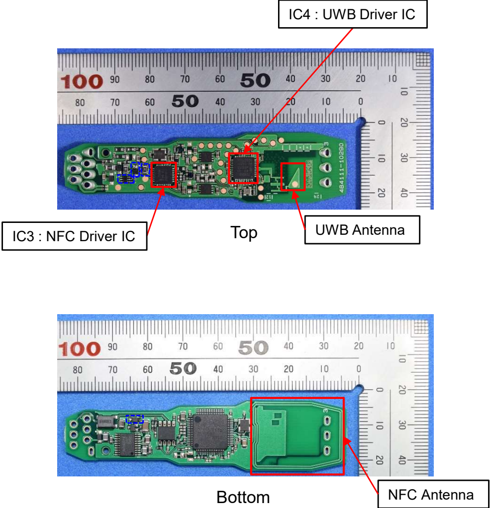
Figure 9 PCB (with SW)
