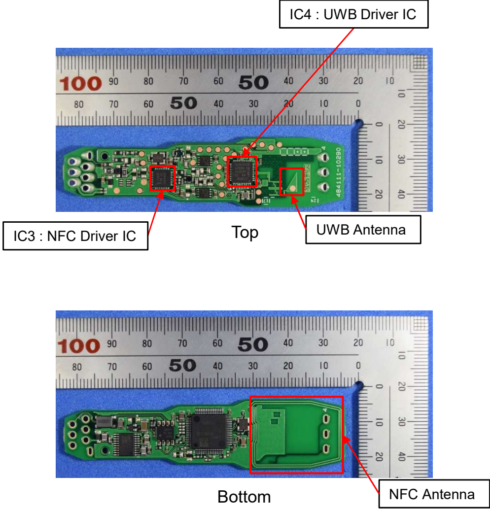
Figure 10 PCB (without SW)
