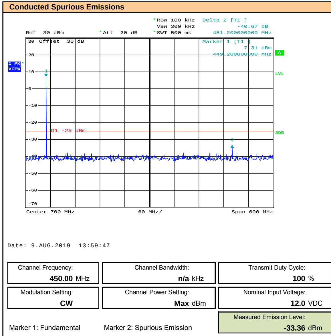
Plot 10.11 – Conducted Spurious Emission, 400MHz – 1000MHz, Channel: 450MHz
