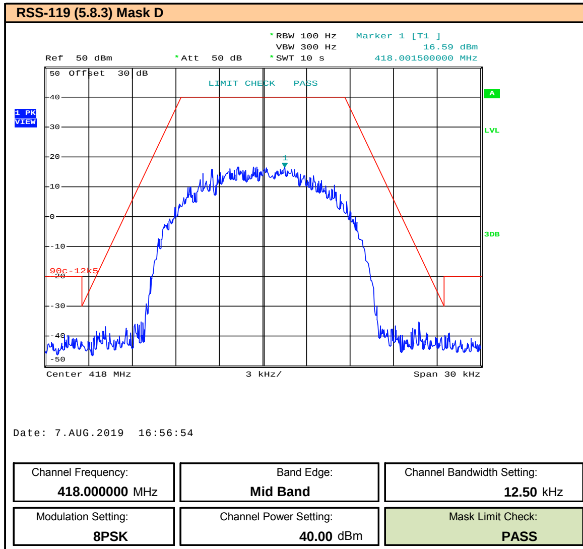
Plot 9.17 – Band Edge and Emissions Mask – 12.5kHz BW – 8PSK – 418MHz, ISED
