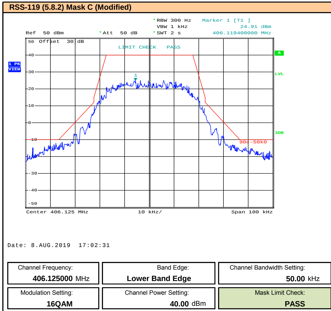
Plot 9.99 – Band Edge and Emissions Mask – 50kHz BW – 16QAM – 406.125MHz, ISED
