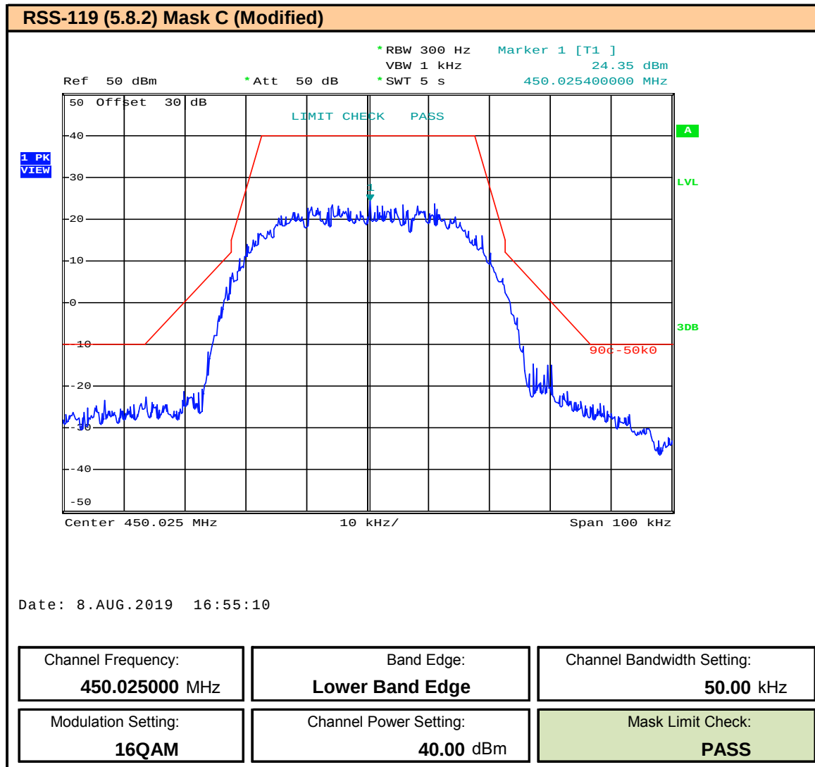
Plot 9.102 – Band Edge and Emissions Mask – 50kHz BW – 16QAM – 450.025MHz
