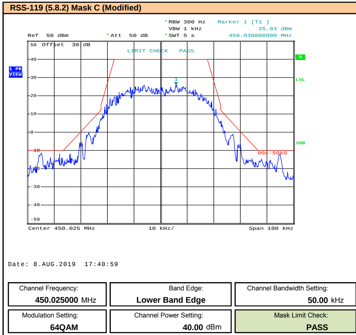
Plot 9.114 – Band Edge and Emissions Mask – 50kHz BW – 64QAM – 450.025MHz, ISED
