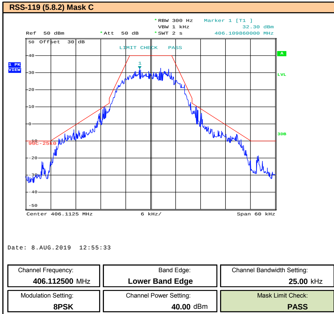
Plot 9.52 – Band Edge and Emissions Mask – 25kHz BW – 8PSK – 406.1125MHz, ISED
