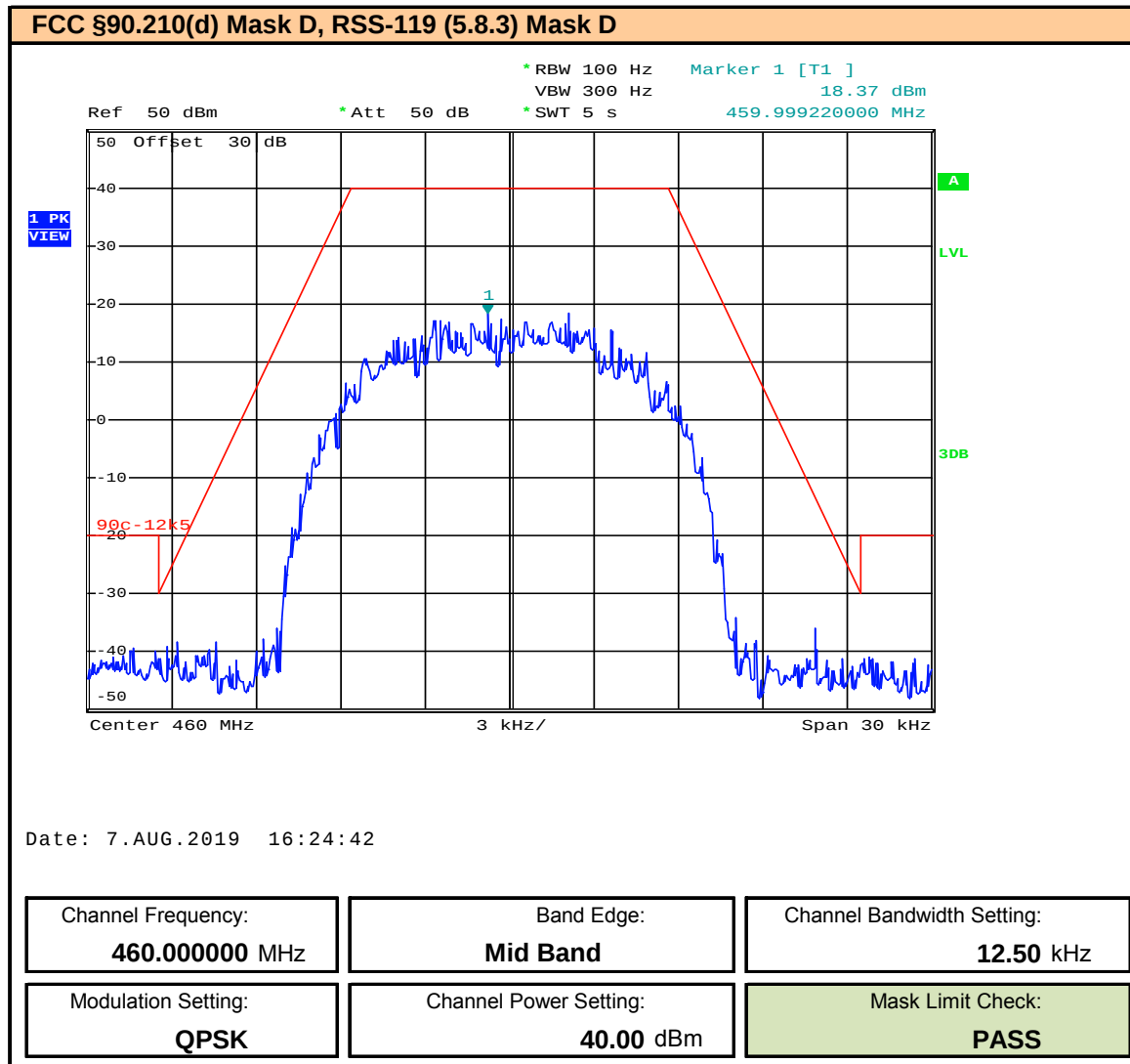
Plot 9.26 – Band Edge and Emissions Mask – 12.5kHz BW – QPSK – 460MHz
