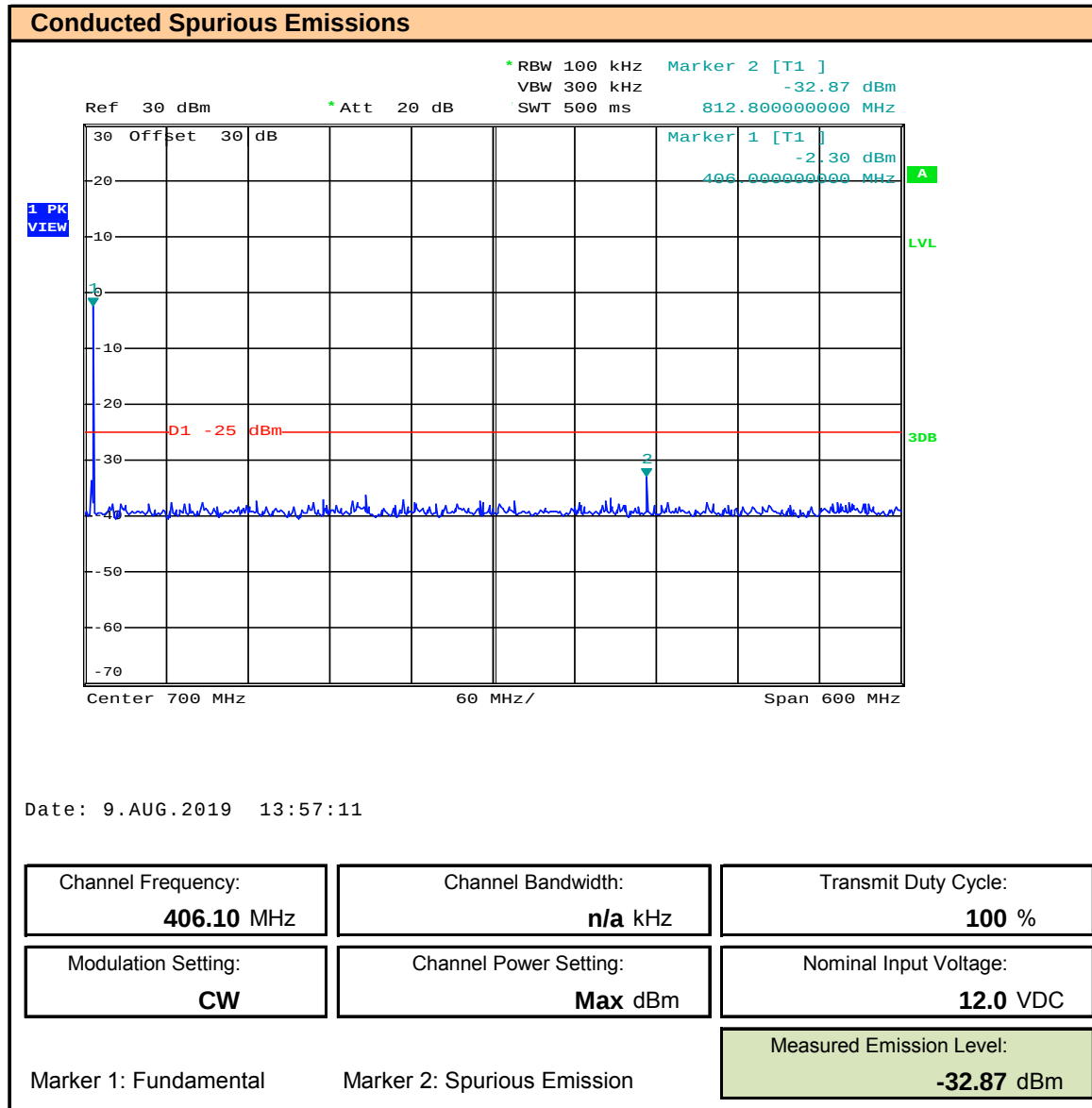
Plot 10.2 – Conducted Spurious Emission, 400MHz – 1000MHz, Channel: 406.1MHz
