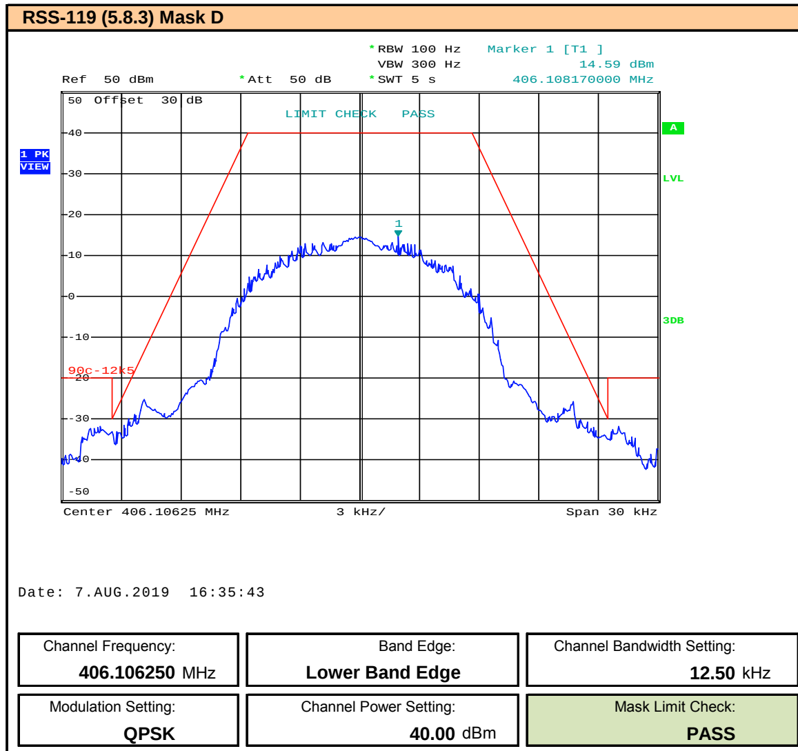
Plot 9.22 – Band Edge and Emissions Mask – 12.5kHz BW – QPSK – 406.10625MHz, ISED
