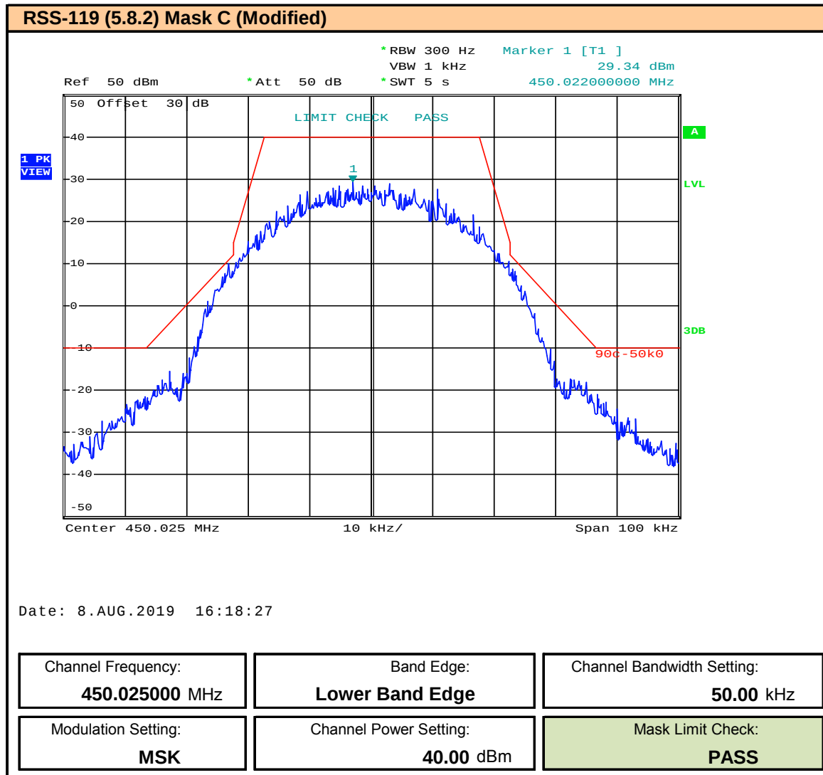
Plot 9.85 – Band Edge and Emissions Mask – 50kHz BW – MSK – 450.025MHz
