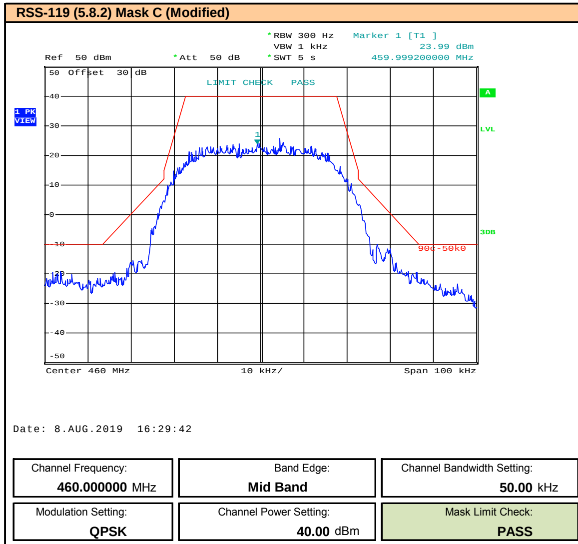
Plot 9.97 – Band Edge and Emissions Mask – 50kHz BW – QPSK – 460MHz
