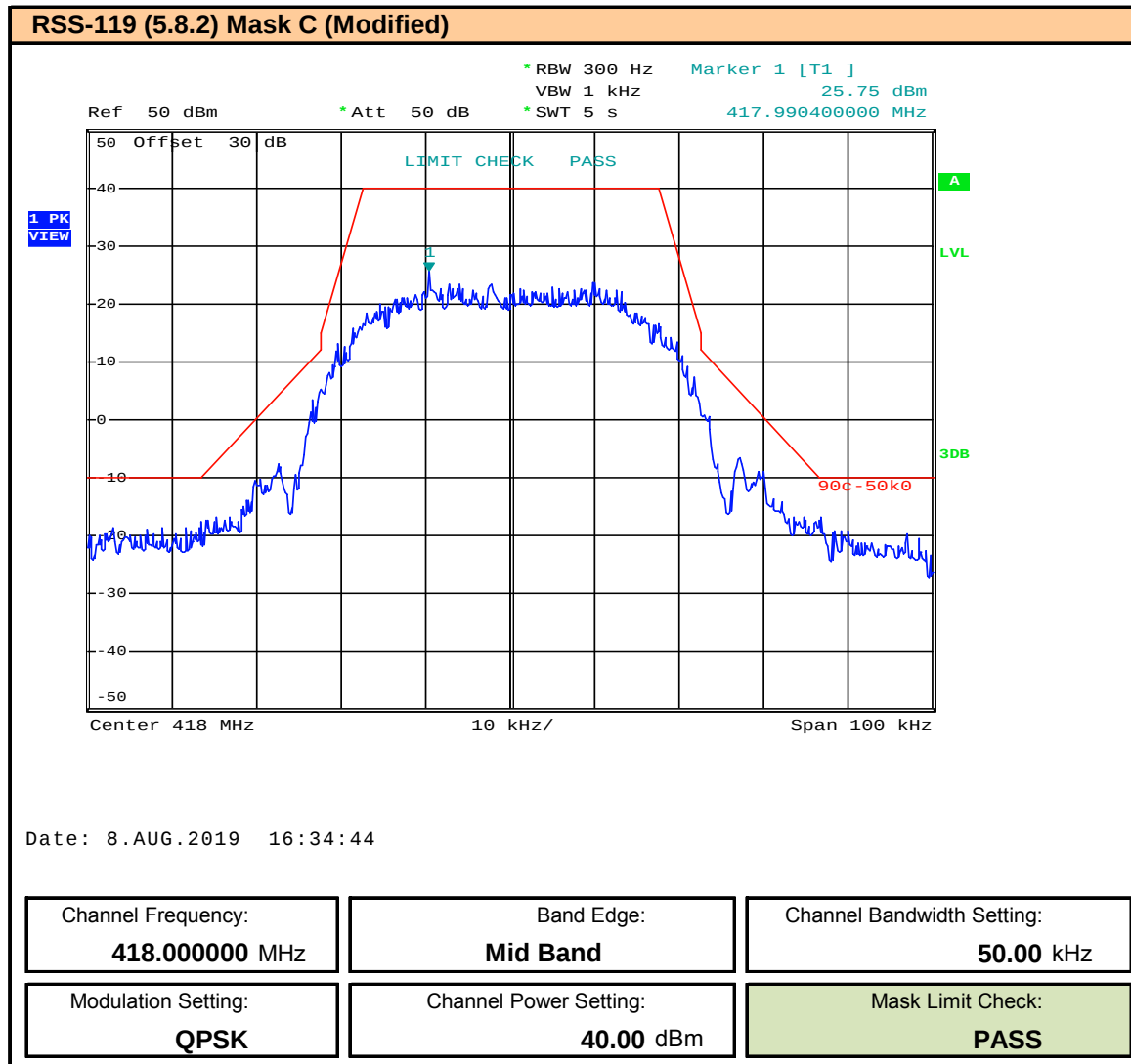
Plot 9.94 – Band Edge and Emissions Mask – 50kHz BW – QPSK – 418MHz, ISED
