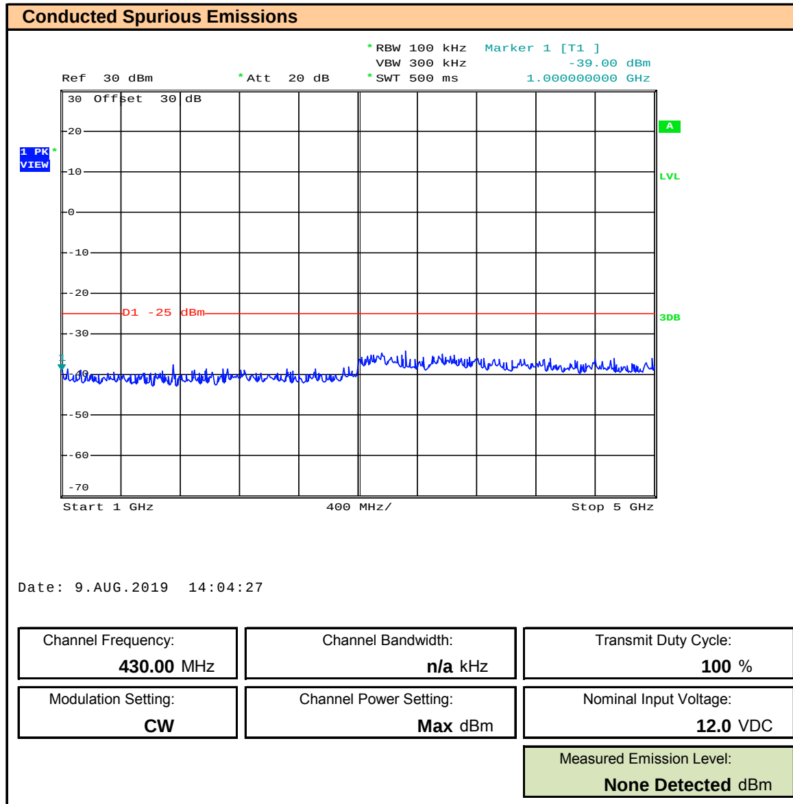
Plot 10.9 – Conducted Spurious Emission, 1 – 5GHz, Channel: 430MHz
