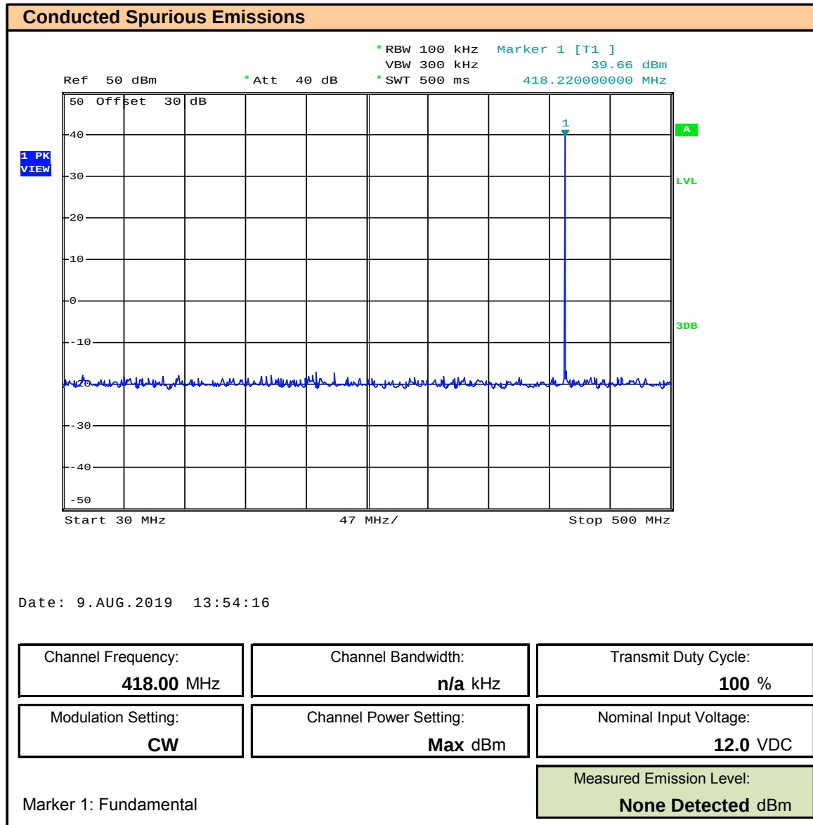
Plot 10.4 – Conducted Spurious Emission, 30MHz – 500MHz, Channel: 418MHz
