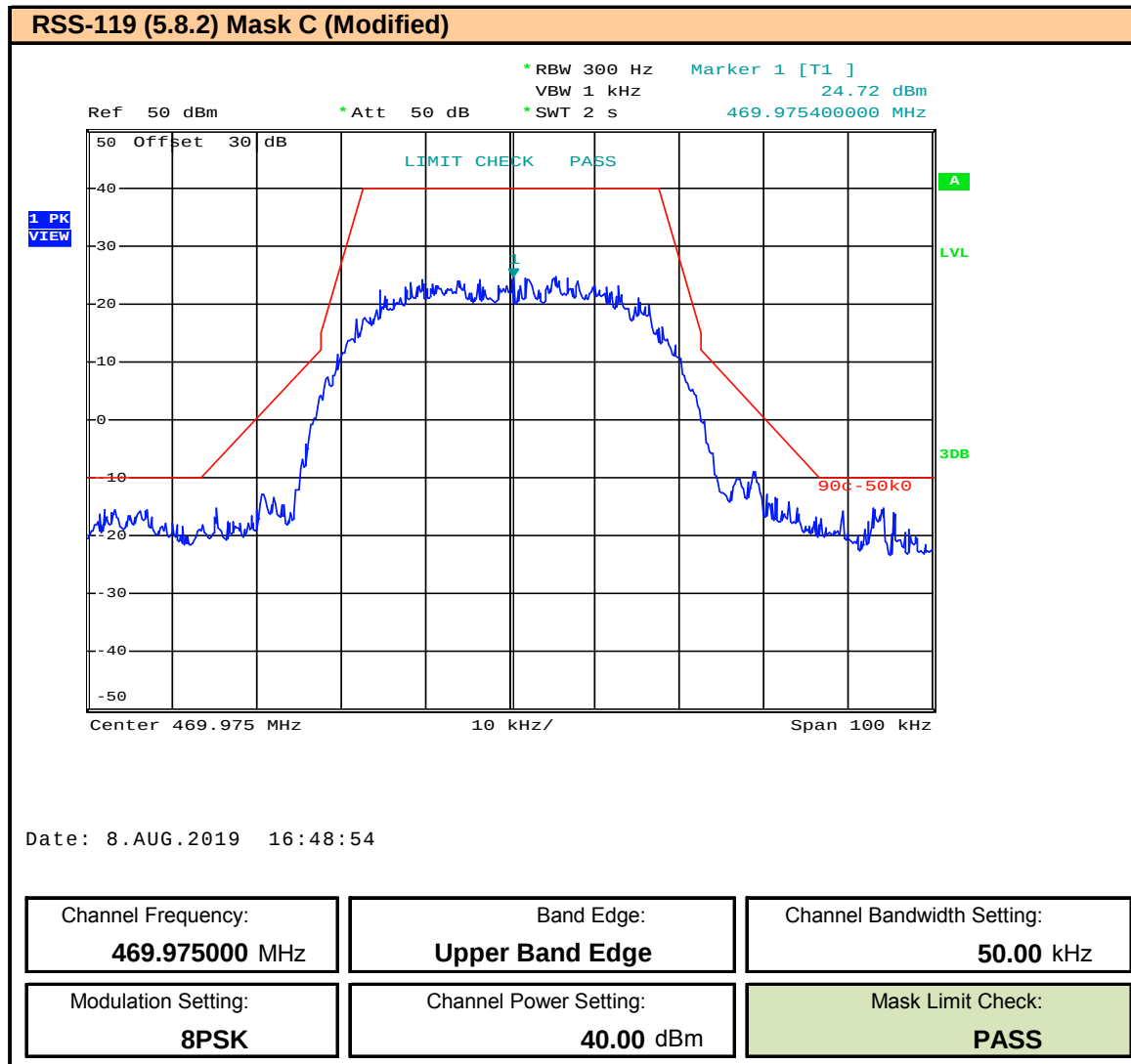
Plot 9.92 – Band Edge and Emissions Mask – 50kHz BW – 8PSK – 469.975MHz
