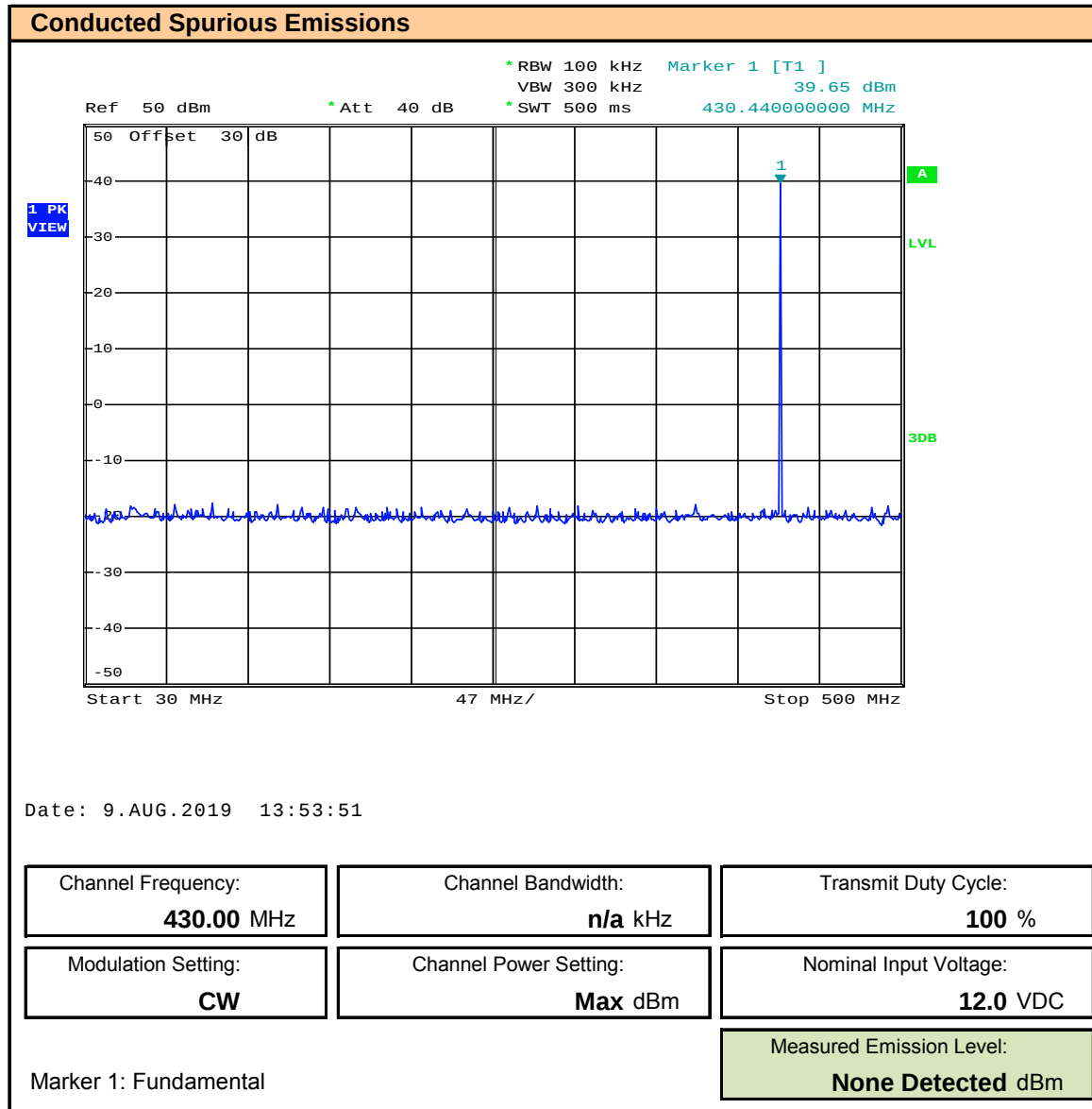
Plot 10.7 – Conducted Spurious Emission, 30MHz – 500MHz, Channel: 430MHz
