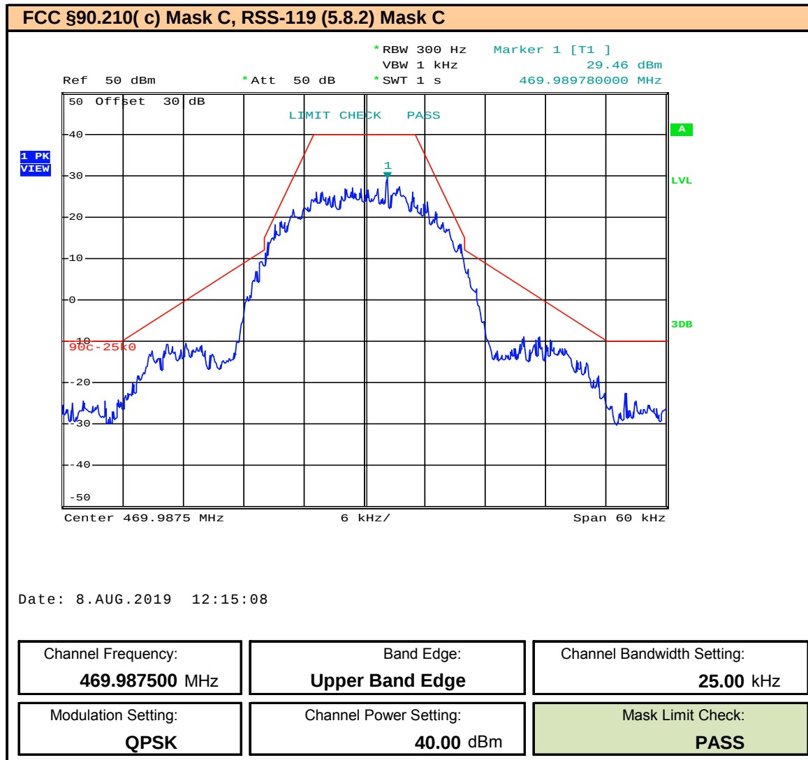
Plot 9.63 – Band Edge and Emissions Mask – 25kHz BW – QPSK – 469.9875MHz
