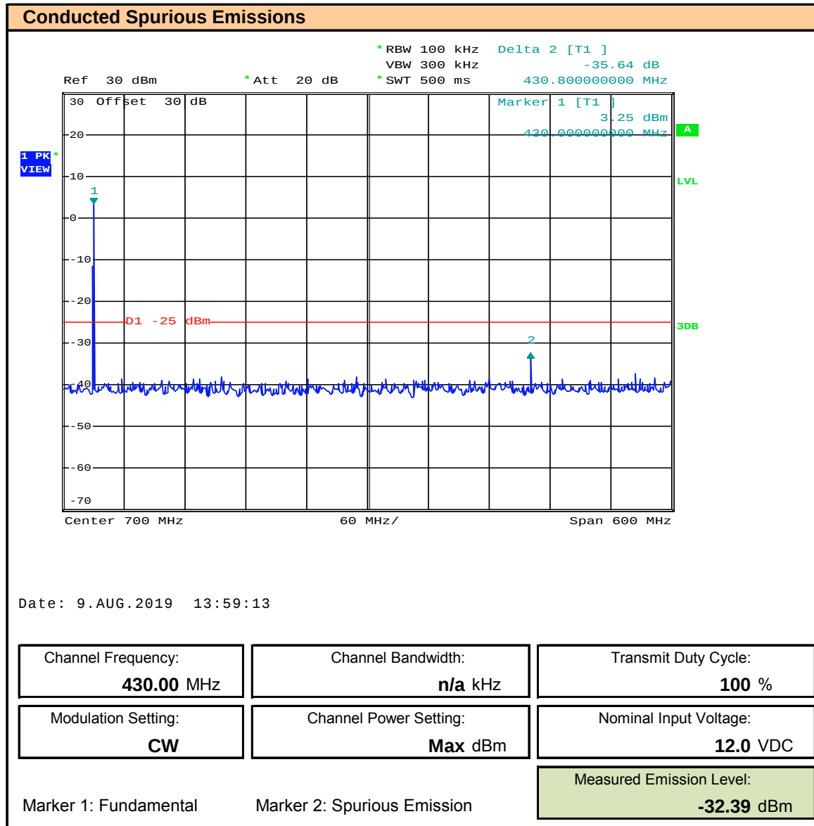
Plot 10.8 – Conducted Spurious Emission, 400MHz – 1000MHz, Channel: 430MHz
