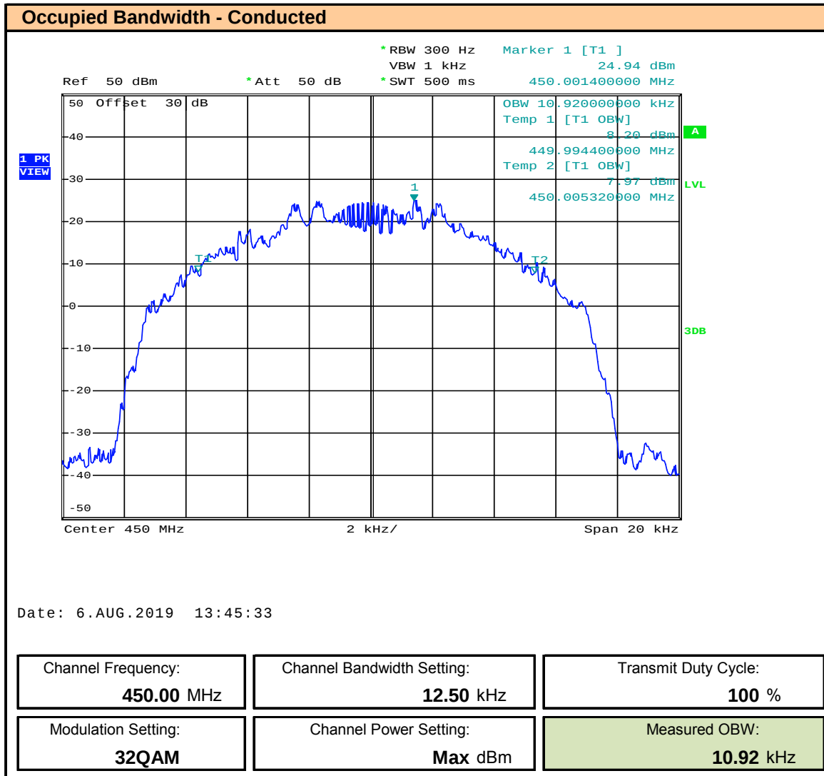
Plot 8.34 – OBW - 12.5kHz BW – 32QAM – 450MHz
