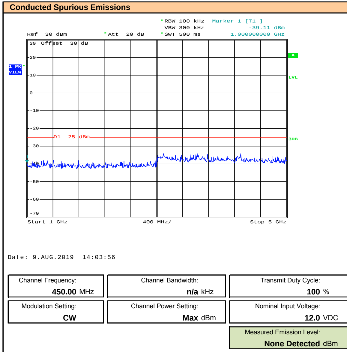
Plot 10.12 – Conducted Spurious Emission, 1 – 5GHz, Channel: 450MHz
