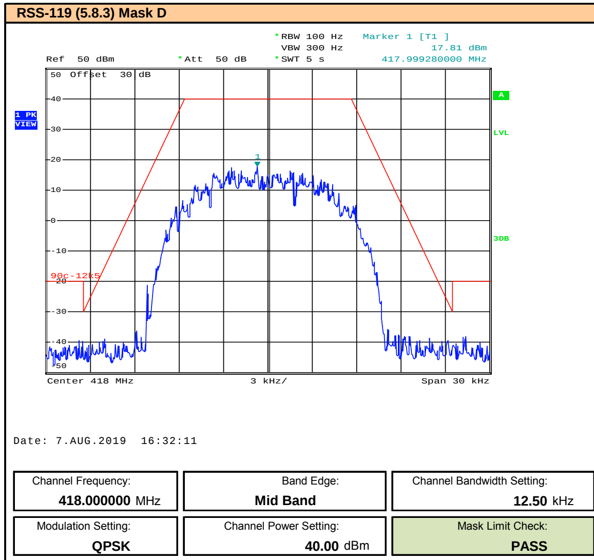
Plot 9.23 – Band Edge and Emissions Mask – 12.5kHz BW – QPSK – 418MHz, ISED
