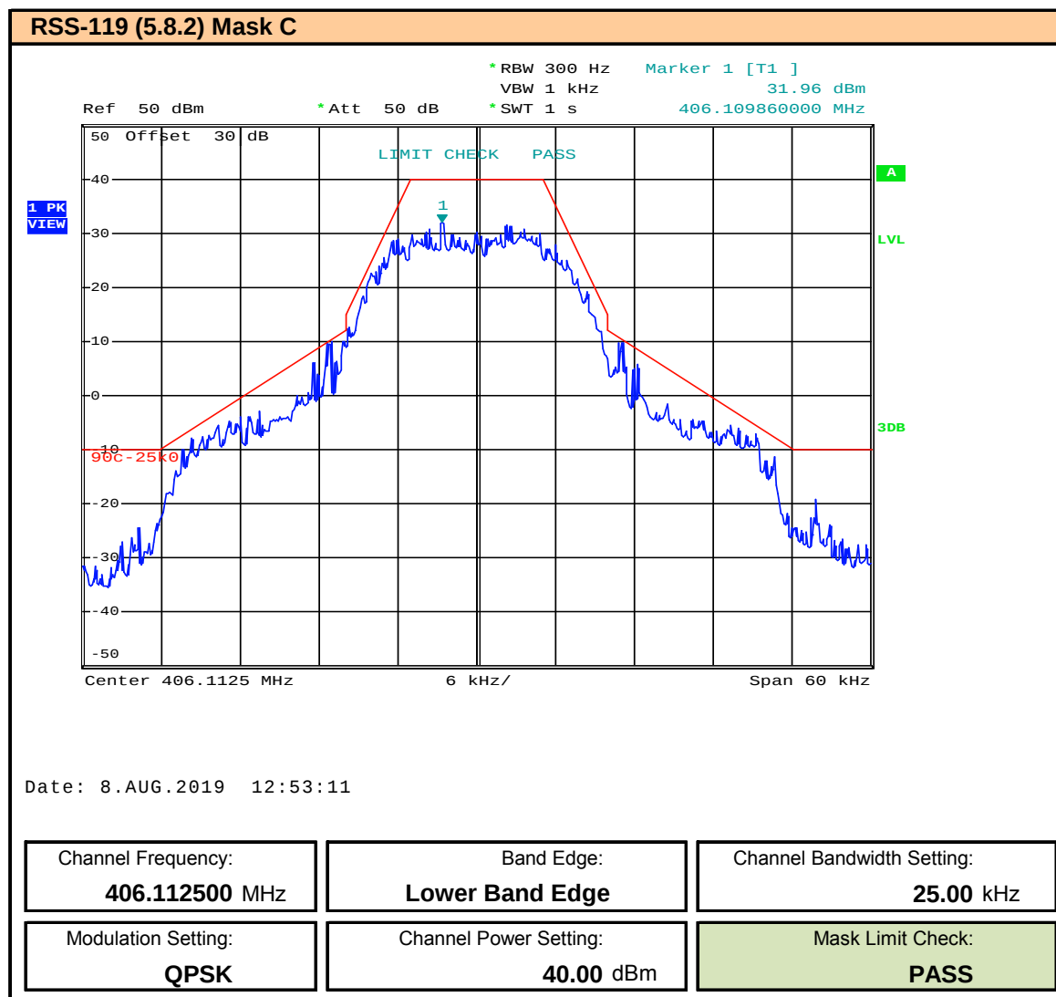
Plot 9.58 – Band Edge and Emissions Mask – 25kHz BW – QPSK – 406.1125MHz, ISED
