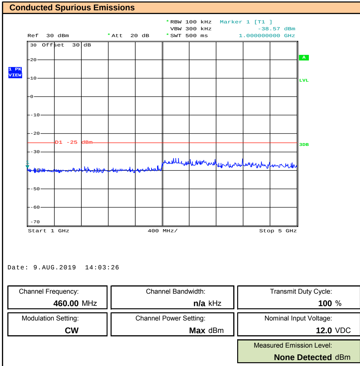
Plot 10.15 – Conducted Spurious Emission, 1 – 5GHz, Channel: 460MHz
