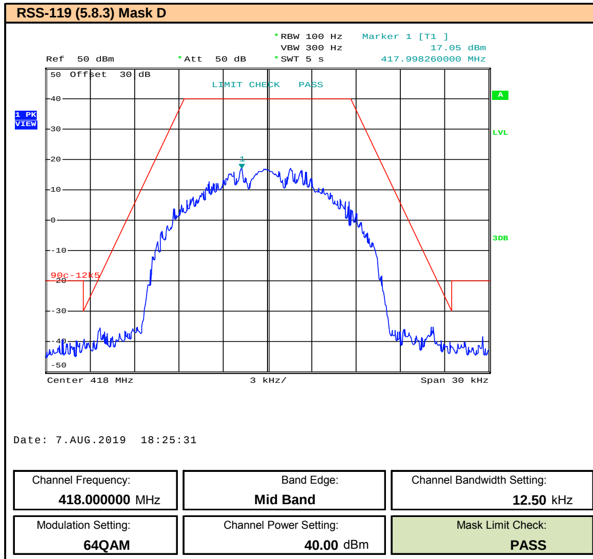
Plot 9.41 – Band Edge and Emissions Mask – 12.5kHz BW – 64QAM – 418MHz, ISED
