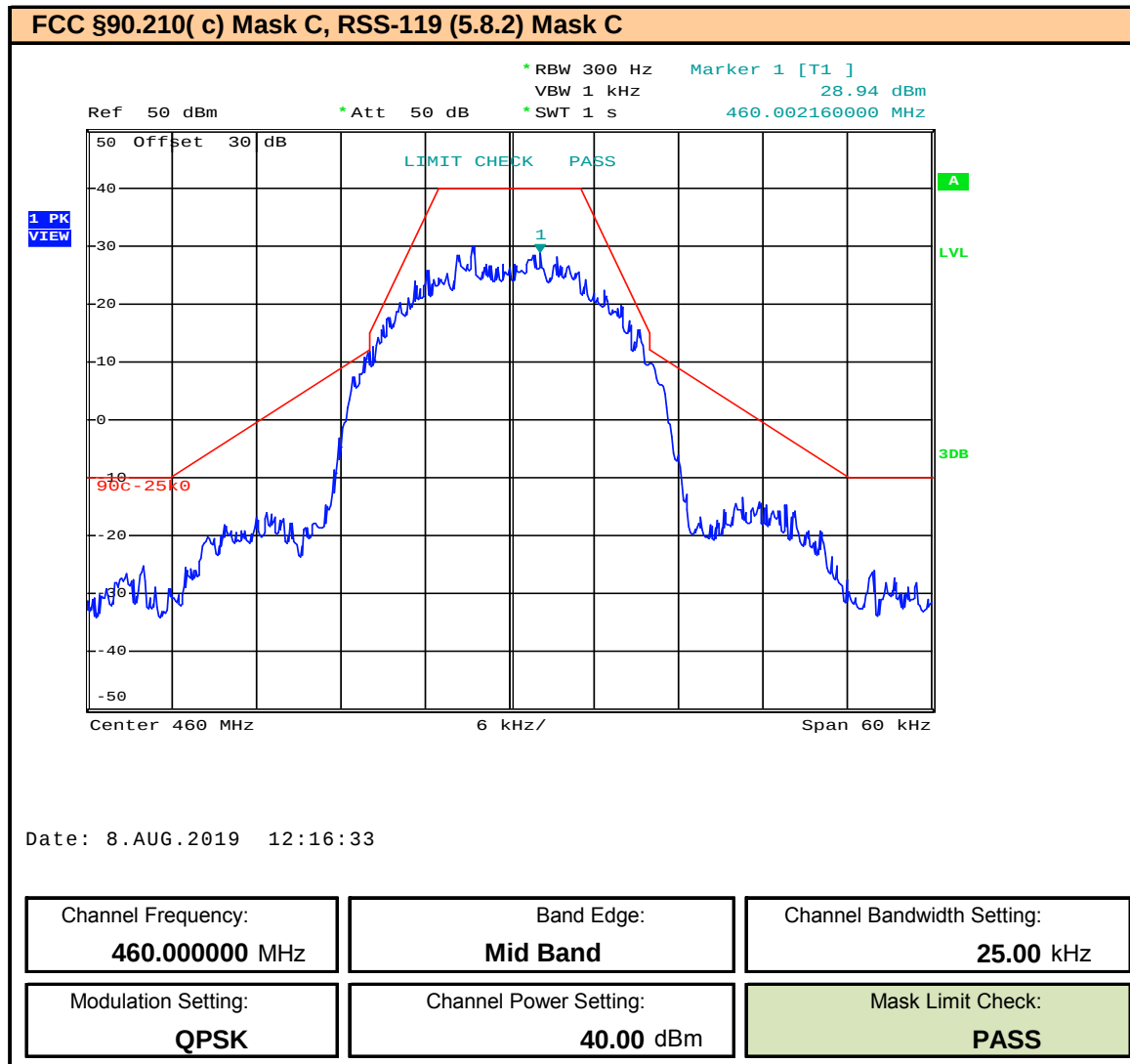
Plot 9.62 – Band Edge and Emissions Mask – 25kHz BW – QPSK – 460MHz
