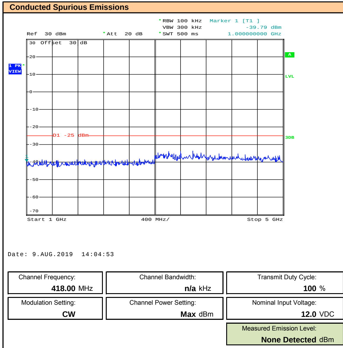
Plot 10.6 – Conducted Spurious Emission, 1 – 5GHz, Channel: 418MHz
