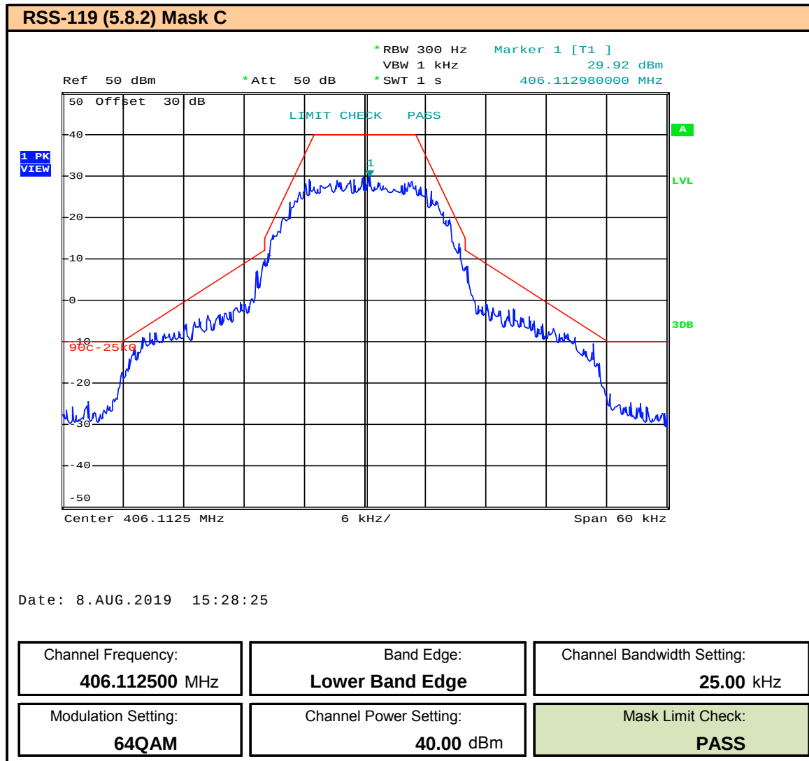
Plot 9.76 – Band Edge and Emissions Mask – 25kHz BW – 64QAM – 406.1125MHz, ISED
