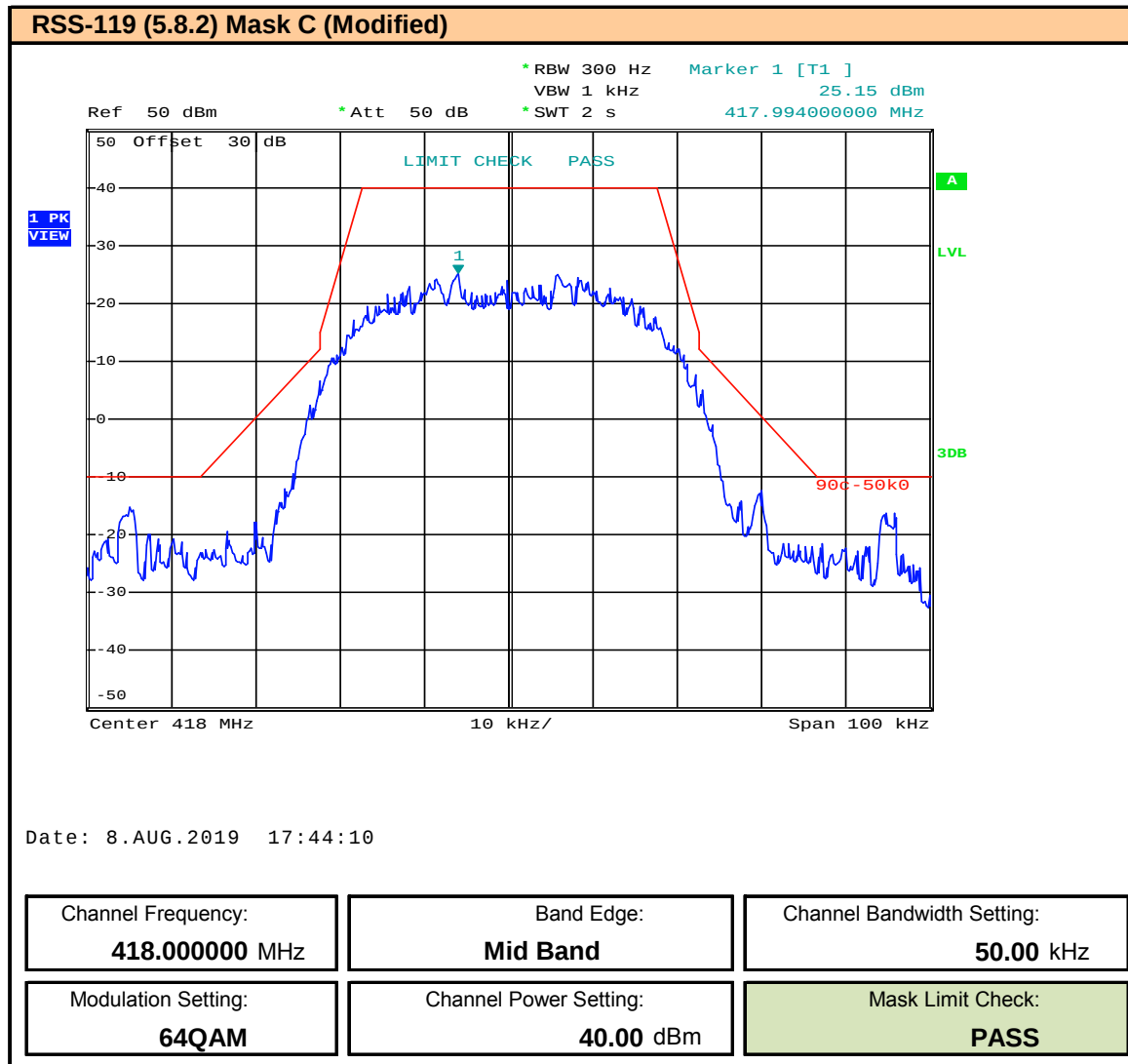
Plot 9.112 – Band Edge and Emissions Mask – 50kHz BW – 64QAM – 418MHz, ISED
