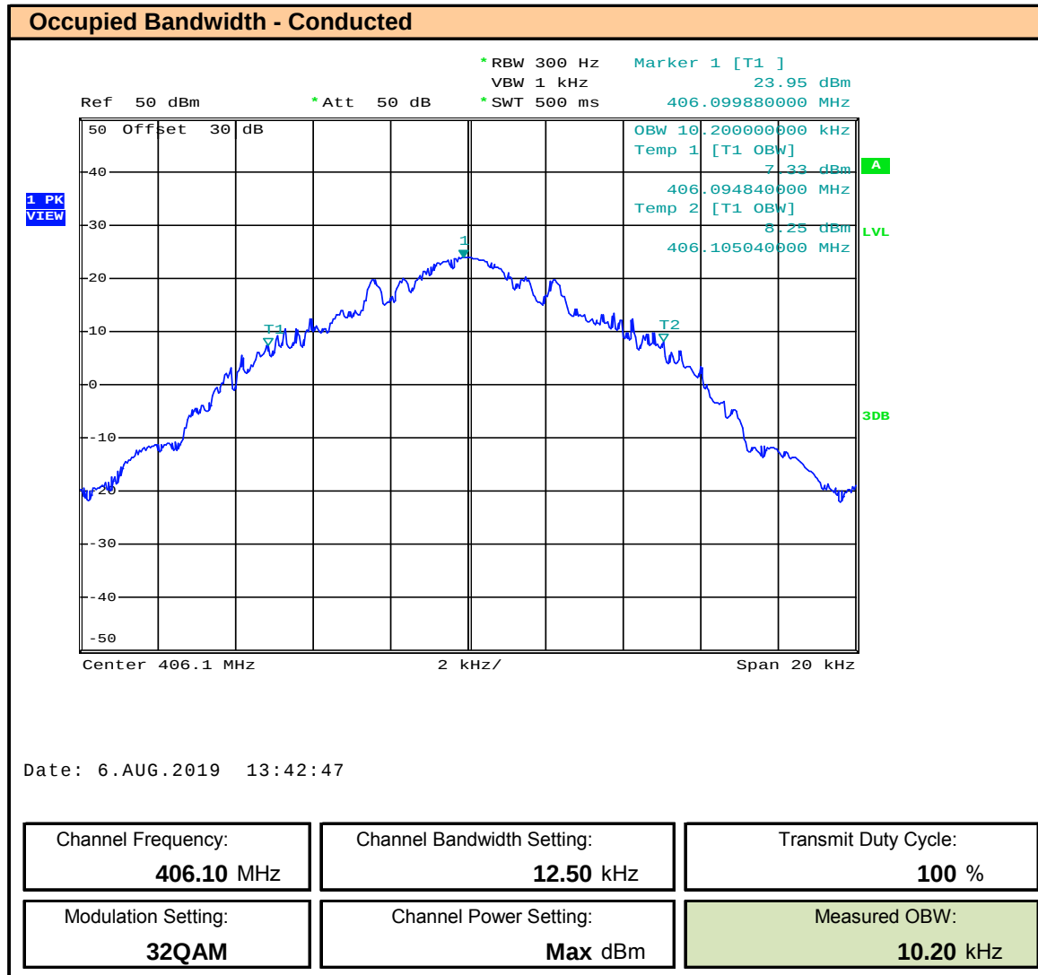
Plot 8.31 – OBW - 12.5kHz BW – 32QAM – 406.1MHz , ISED
