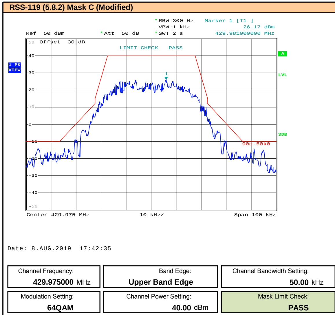
Plot 9.113 – Band Edge and Emissions Mask – 50kHz BW – 64QAM – 429.975MHz, ISED
