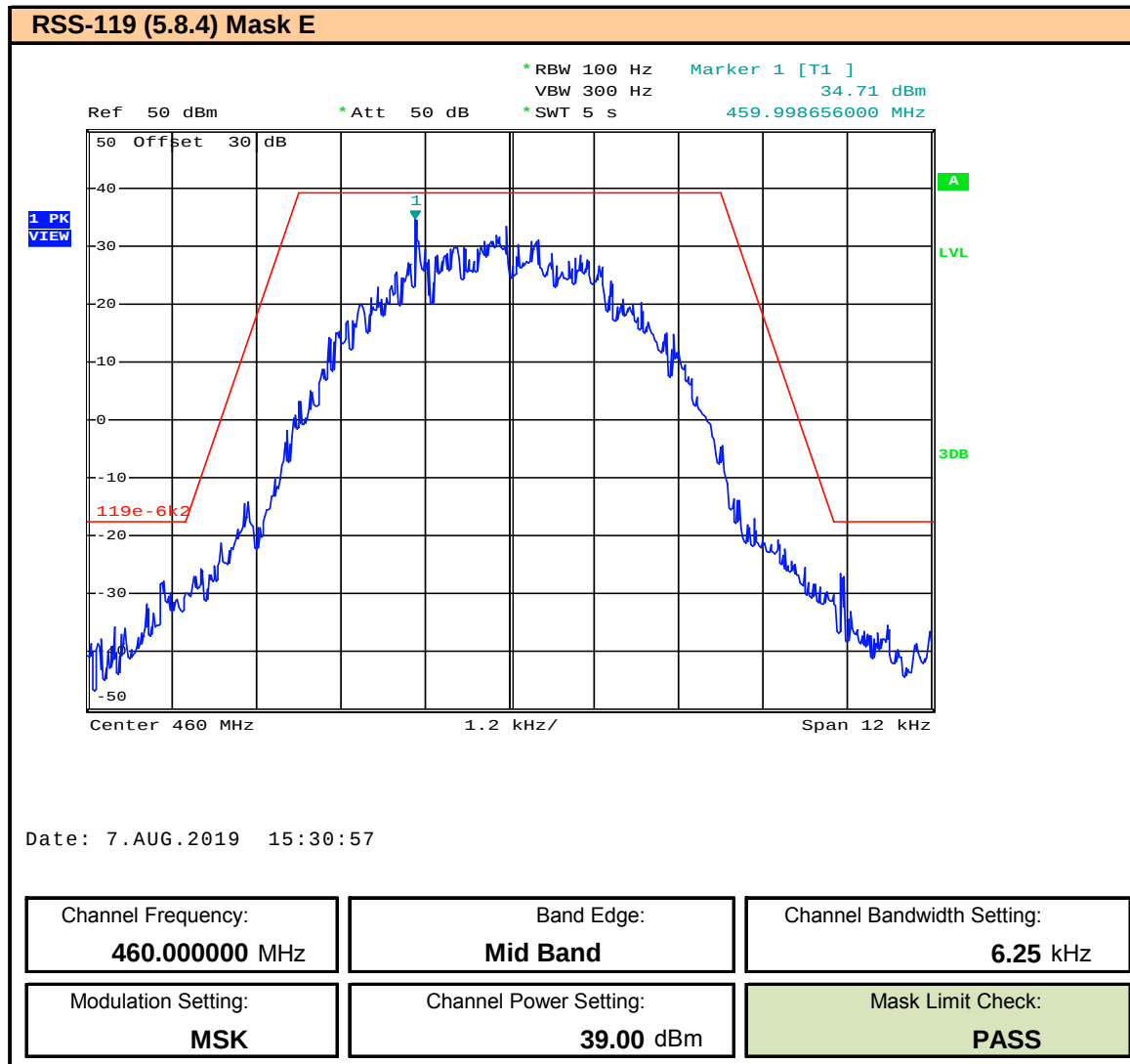
Plot 9.6 – Band Edge and Emissions Mask – 6.25kHz BW – MSK – 460MHz, ISED
