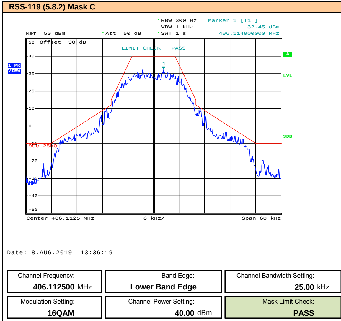
Plot 9.64 – Band Edge and Emissions Mask – 25kHz BW – 16QAM – 406.1125MHz, ISED
