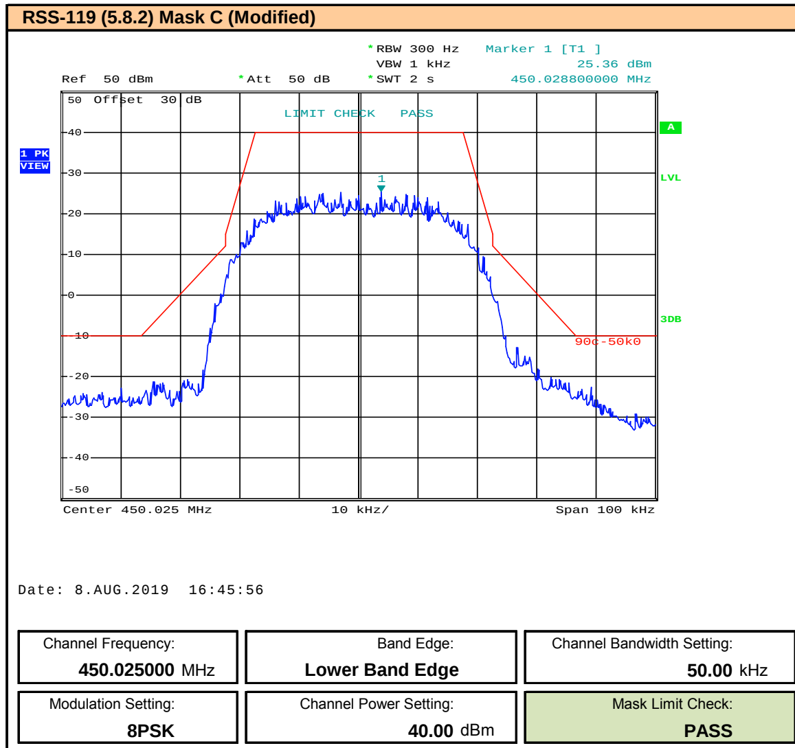
Plot 9.90 – Band Edge and Emissions Mask – 50kHz BW – 8PSK – 450.025MHz
