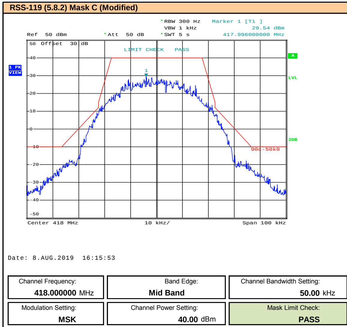
Plot 9.83 – Band Edge and Emissions Mask – 50kHz BW – MSK – 418MHz, ISED
