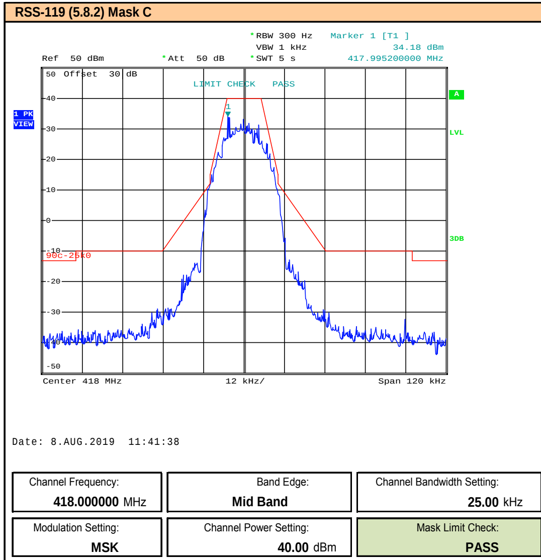
Plot 9.47 – Band Edge and Emissions Mask – 25kHz BW – MSK – 418MHz, ISED
