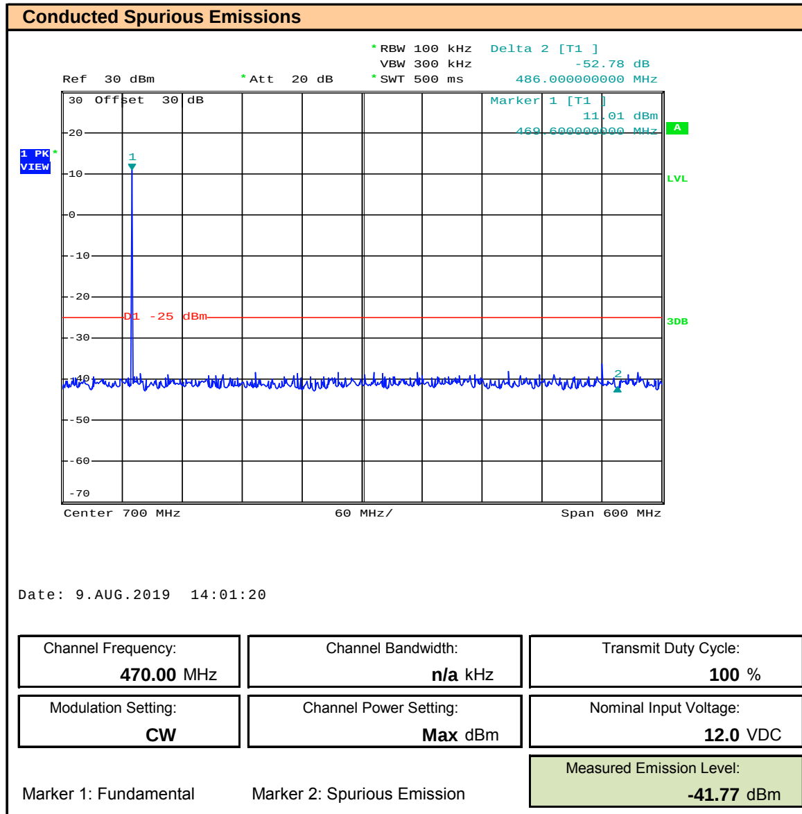
Plot 10.17 – Conducted Spurious Emission, 400MHz – 1000MHz, Channel: 470MHz
