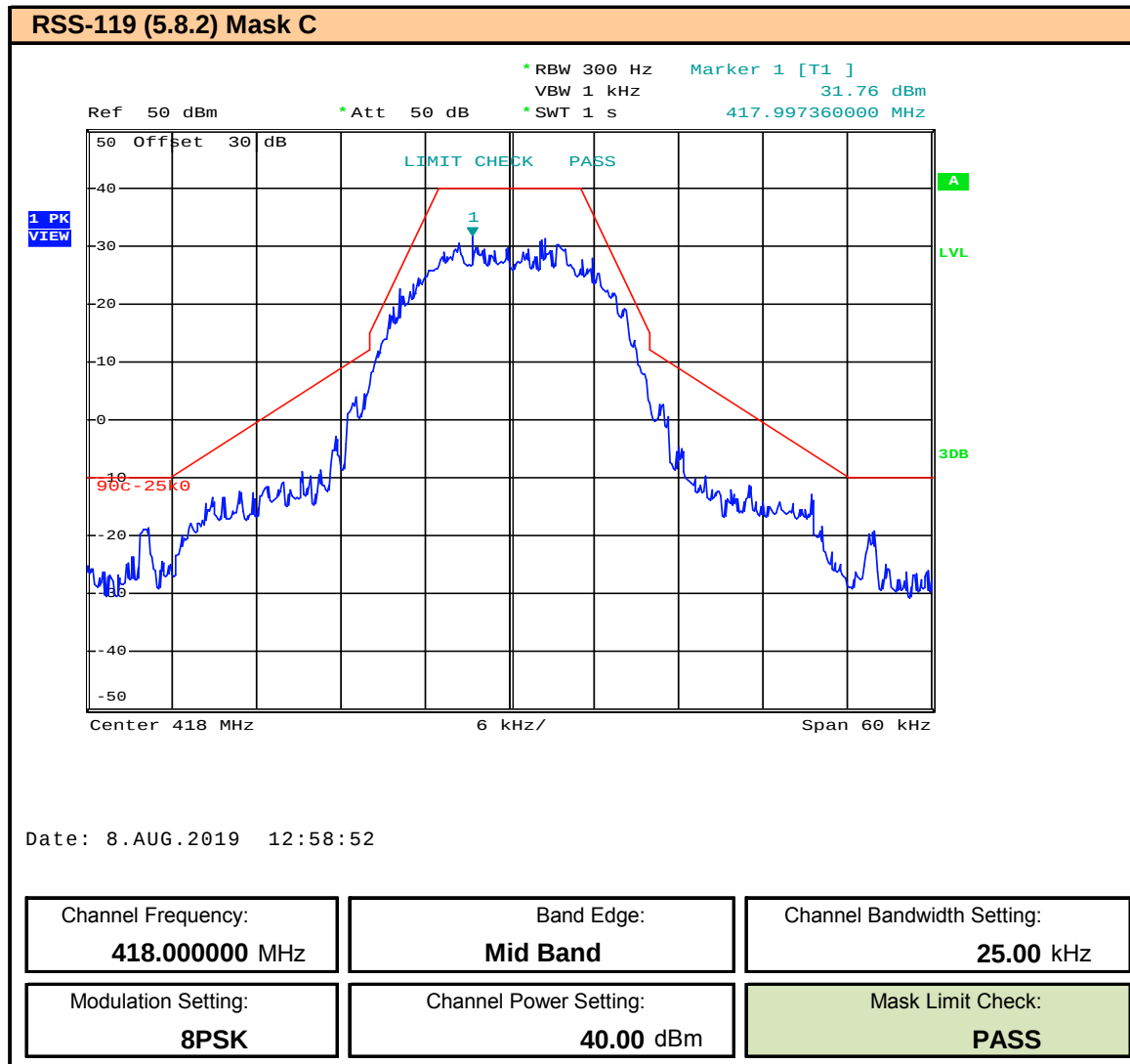
Plot 9.53 – Band Edge and Emissions Mask – 25kHz BW – 8PSK – 418MHz, ISED
