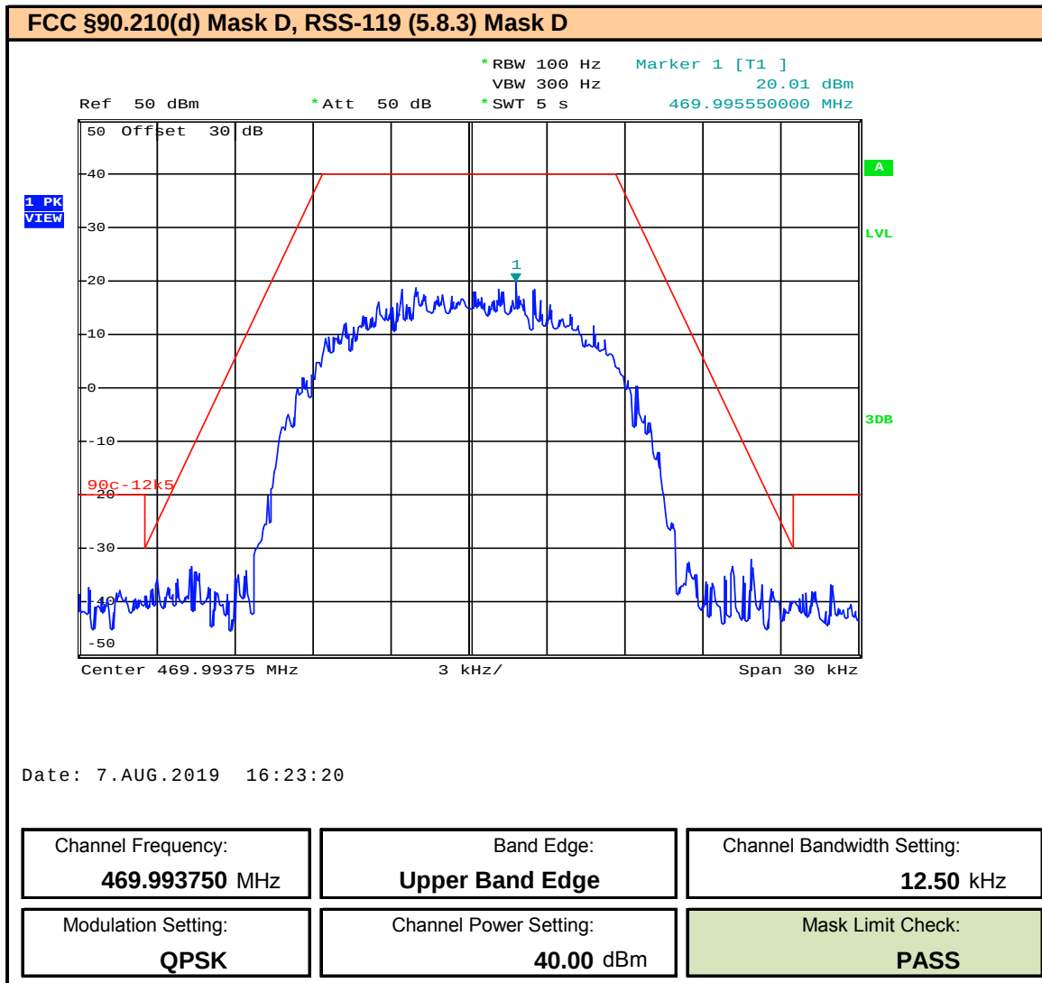
Plot 9.27 – Band Edge and Emissions Mask – 12.5kHz BW – QPSK – 469.99375MHz
