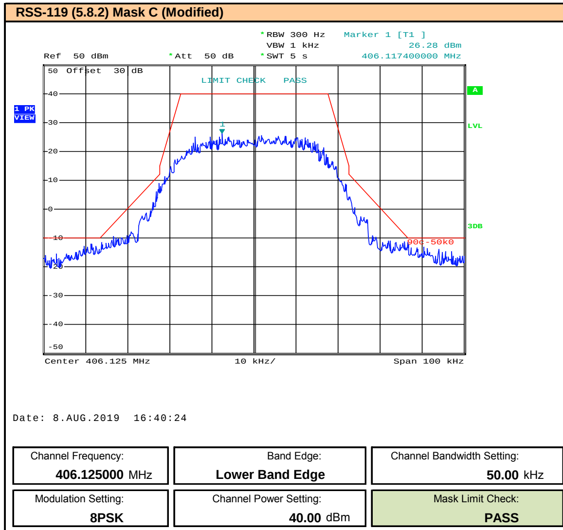
Plot 9.87 – Band Edge and Emissions Mask – 50kHz BW – 8PSK – 406.125MHz, ISED
