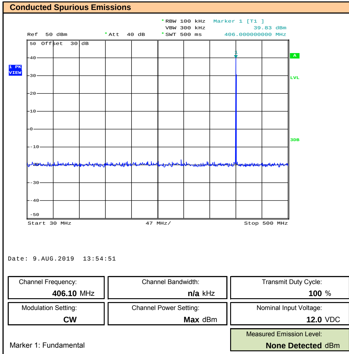
Plot 10.1 – Conducted Spurious Emission, 30MHz – 500MHz, Channel: 406.1MHz
