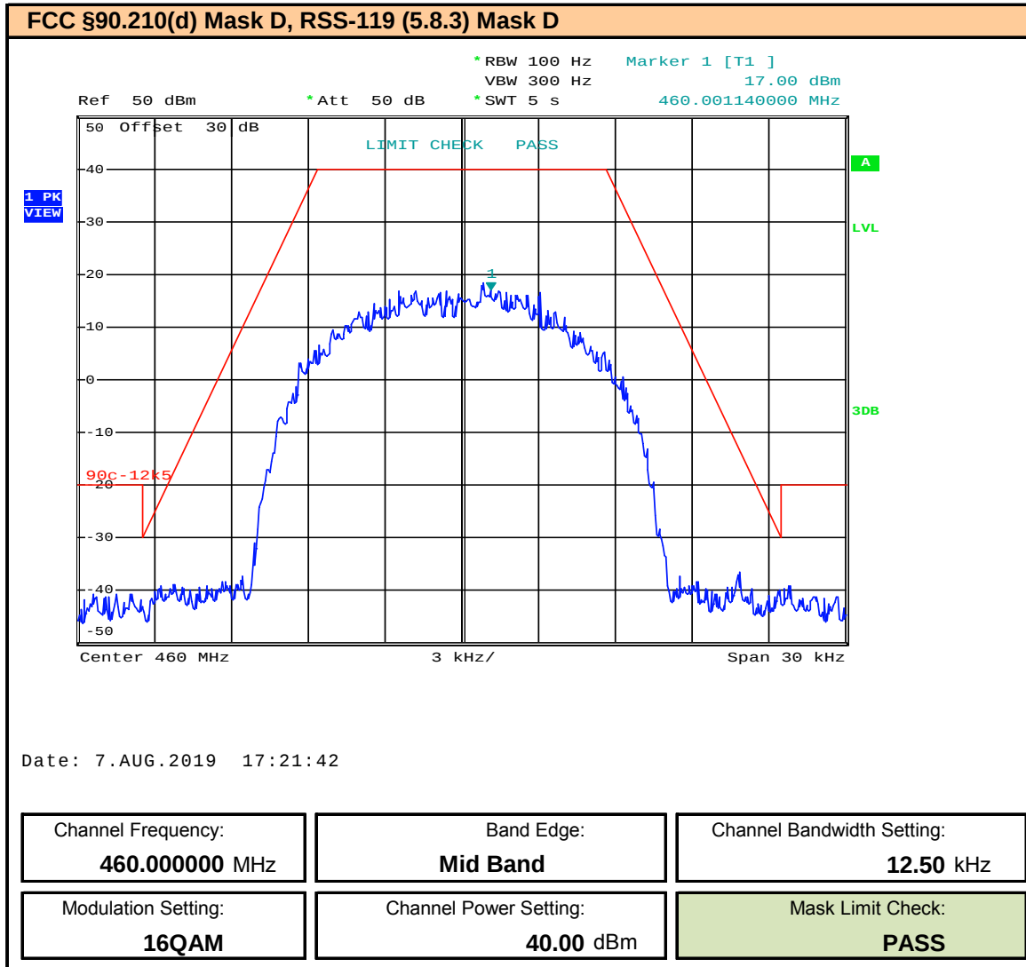
Plot 9.32 – Band Edge and Emissions Mask – 12.5kHz BW – 16QAM – 460MHz
