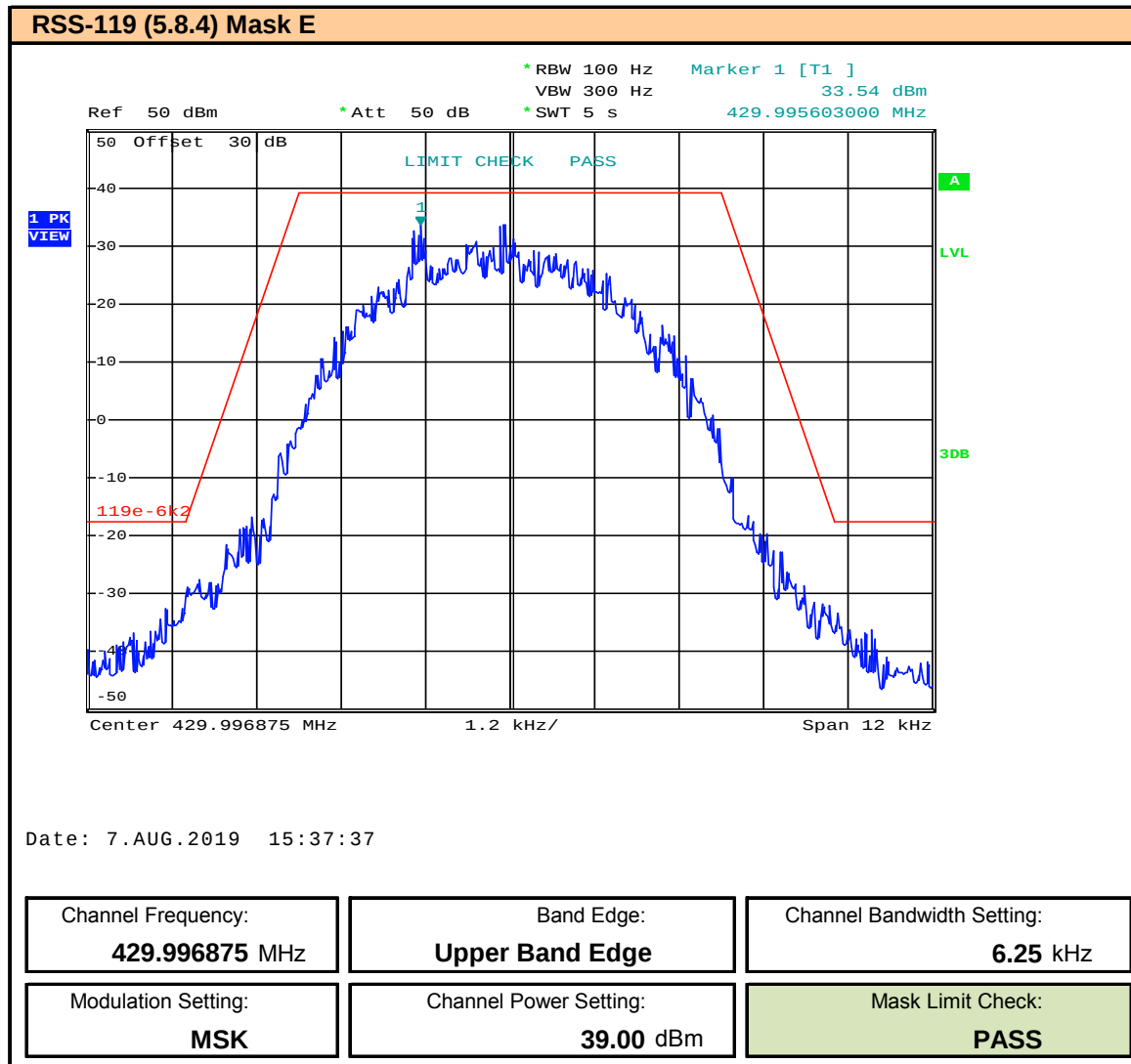
Plot 9.3 – Band Edge and Emissions Mask – 6.25kHz BW – MSK – 429.996875MHz, ISED
