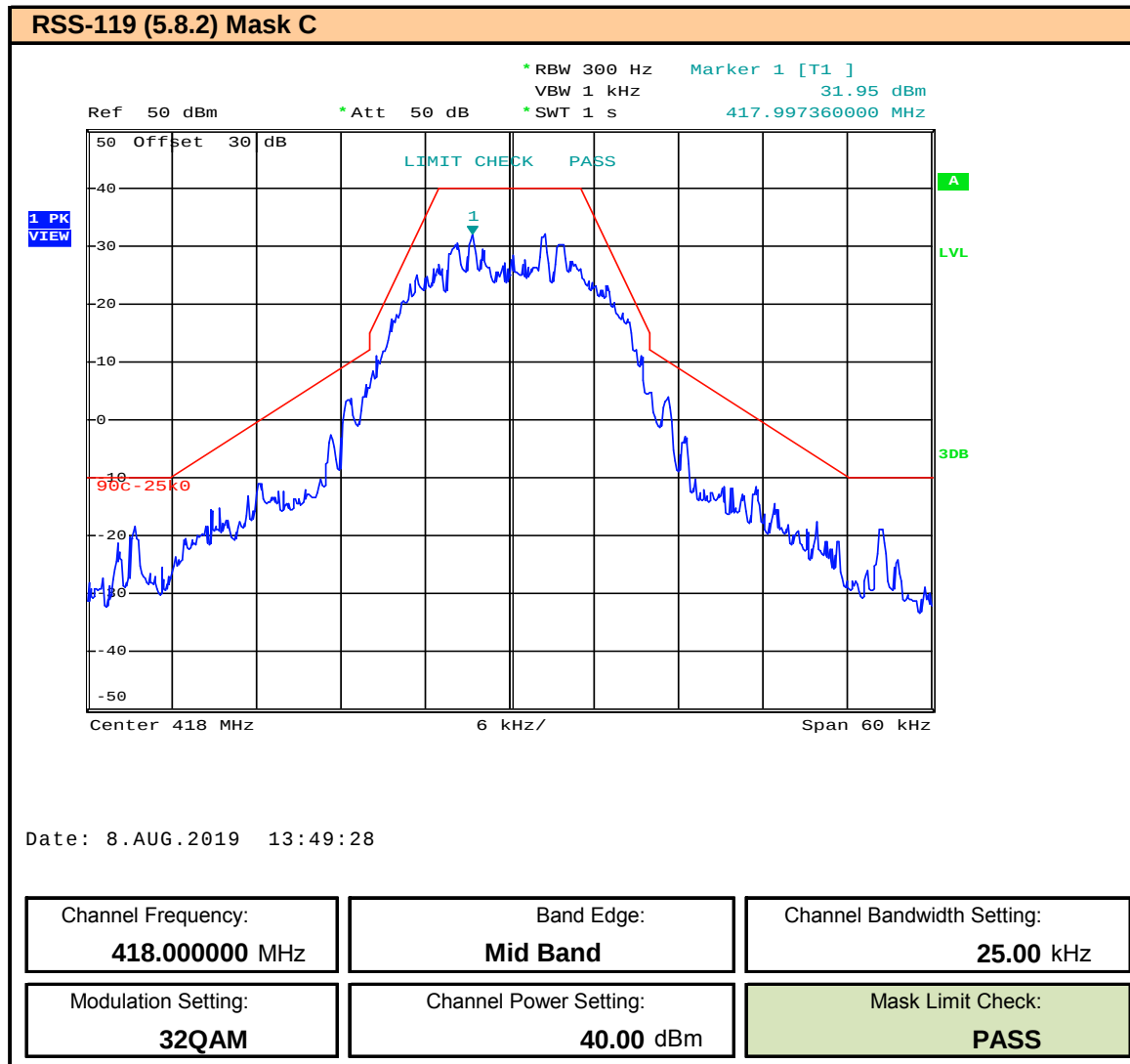
Plot 9.71 – Band Edge and Emissions Mask – 25kHz BW – 32QAM – 418MHz, ISED
