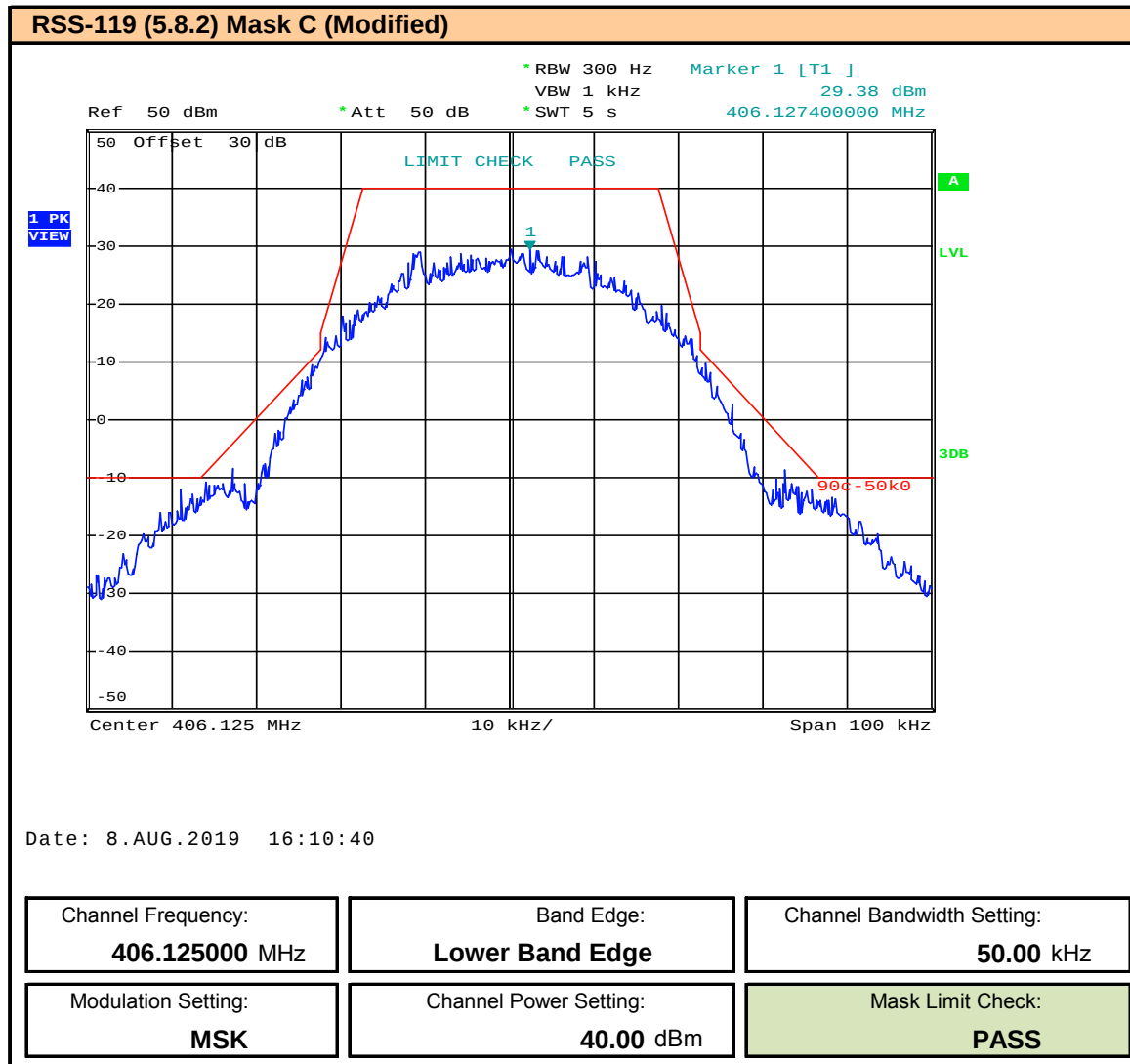
Plot 9.82 – Band Edge and Emissions Mask – 50kHz BW – MSK – 406.125MHz, ISED
