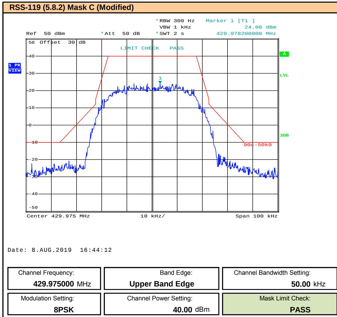
Plot 9.89 – Band Edge and Emissions Mask – 50kHz BW – 8PSK – 429.975MHz, ISED
