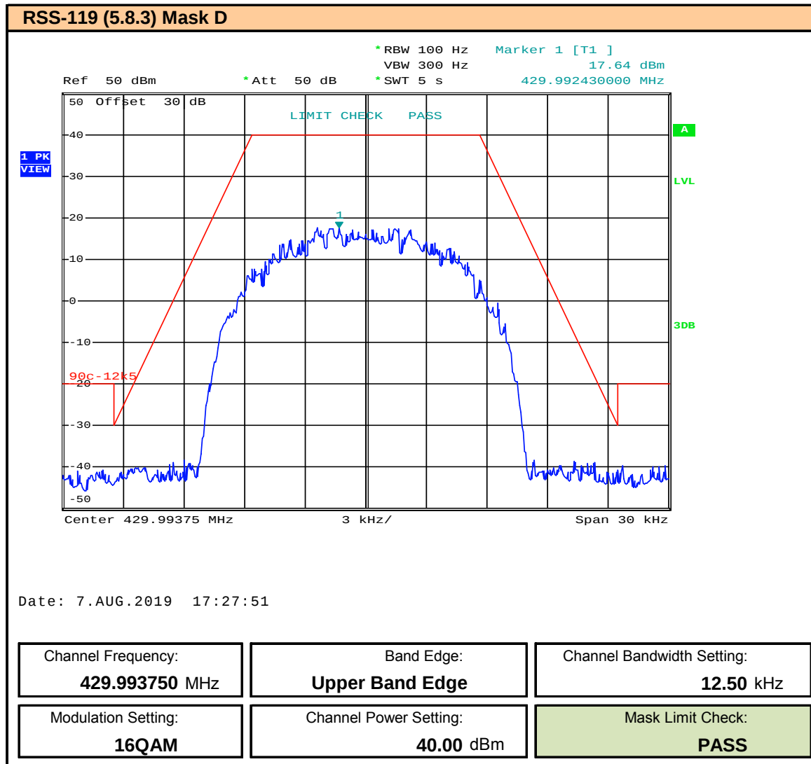
Plot 9.30 – Band Edge and Emissions Mask – 12.5kHz BW – 16QAM – 429.99375MHz, ISED
