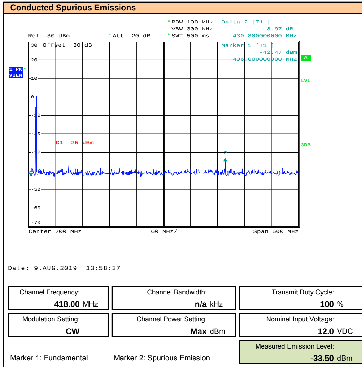
Plot 10.5 – Conducted Spurious Emission, 400MHz – 1000MHz, Channel: 418MHz
