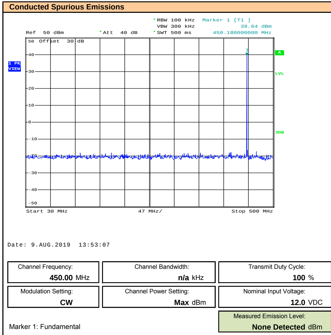
Plot 10.10 – Conducted Spurious Emission, 30MHz – 500MHz, Channel: 450MHz
