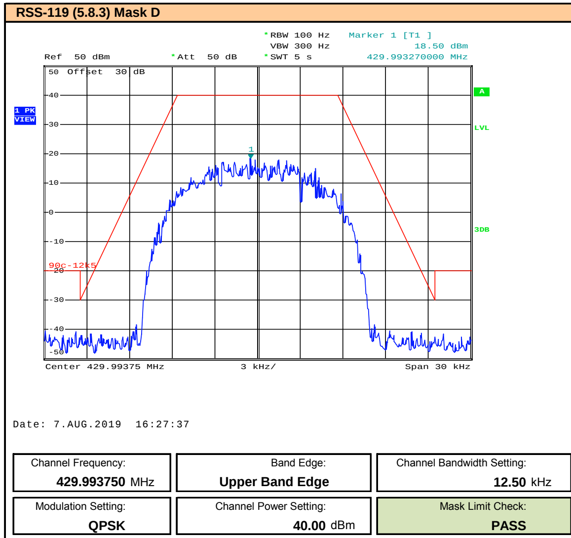
Plot 9.24 – Band Edge and Emissions Mask – 12.5kHz BW – QPSK – 429.99375MHz, ISED
