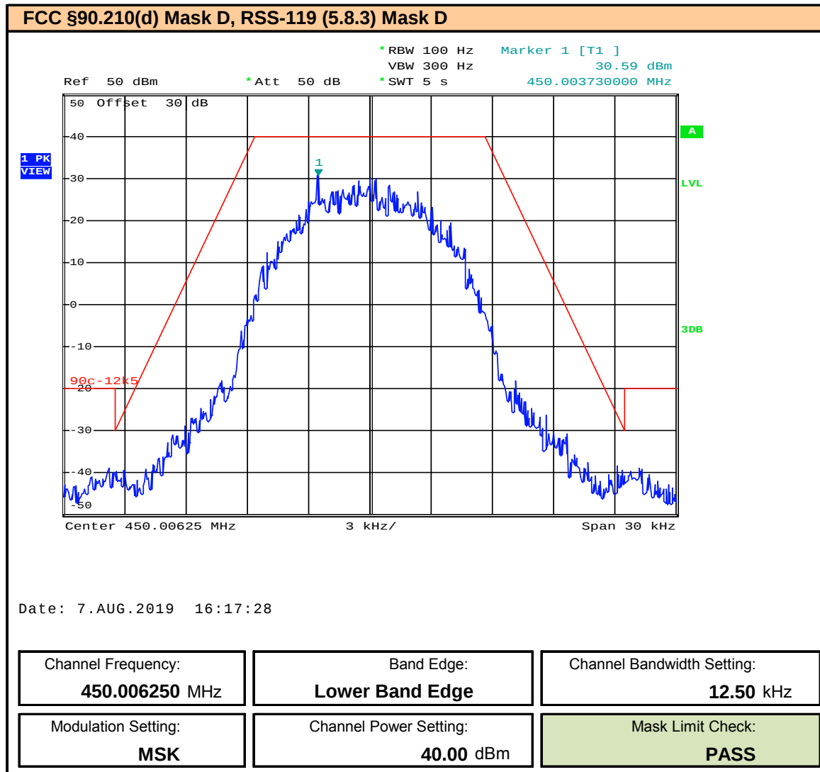
Plot 9.13 – Band Edge and Emissions Mask – 12.5kHz BW – MSK – 450.00625MHz
