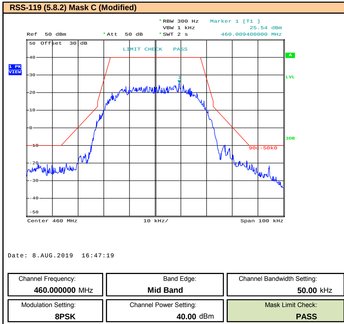
Plot 9.91 – Band Edge and Emissions Mask – 50kHz BW – 8PSK – 460MHz
