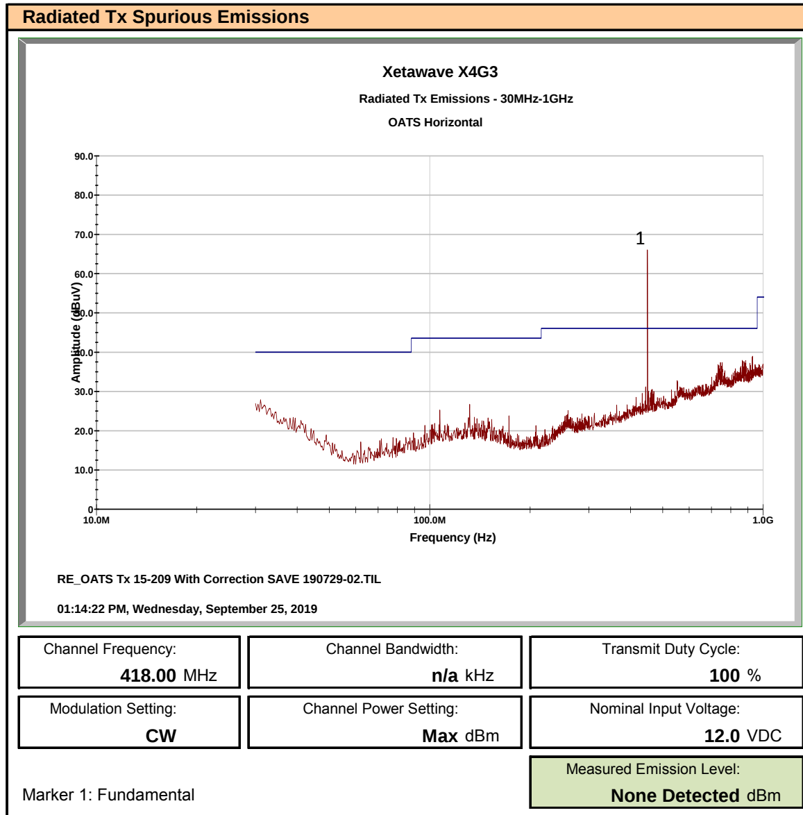
Plot 11.1 – Radiates Tx Spurious Emissions – OATS - Horizontal
