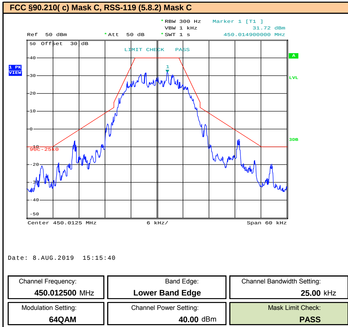
Plot 9.79 – Band Edge and Emissions Mask – 25kHz BW – 64QAM – 450.0125MHz
