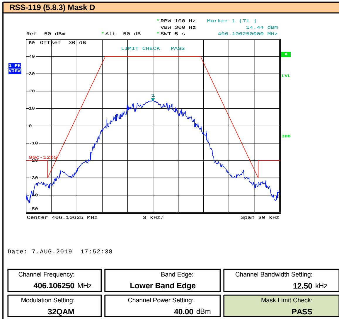
Plot 9.34 – Band Edge and Emissions Mask – 12.5kHz BW – 32QAM – 406.10625MHz, ISED
