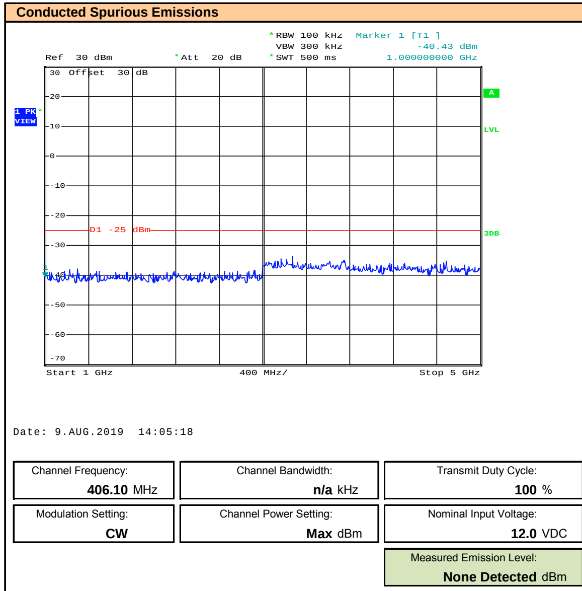
Plot 10.3 – Conducted Spurious Emission, 1 – 5GHz, Channel: 406.1MHz
