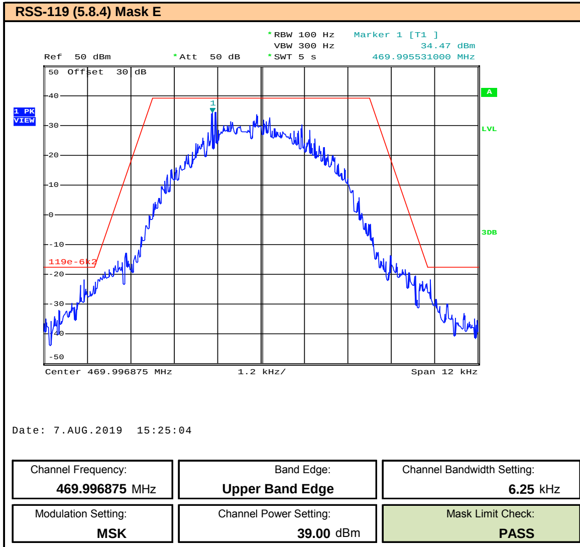
Plot 9.8 – Band Edge and Emissions Mask – 6.25kHz BW – MSK – 469.996875MHz, ISED
