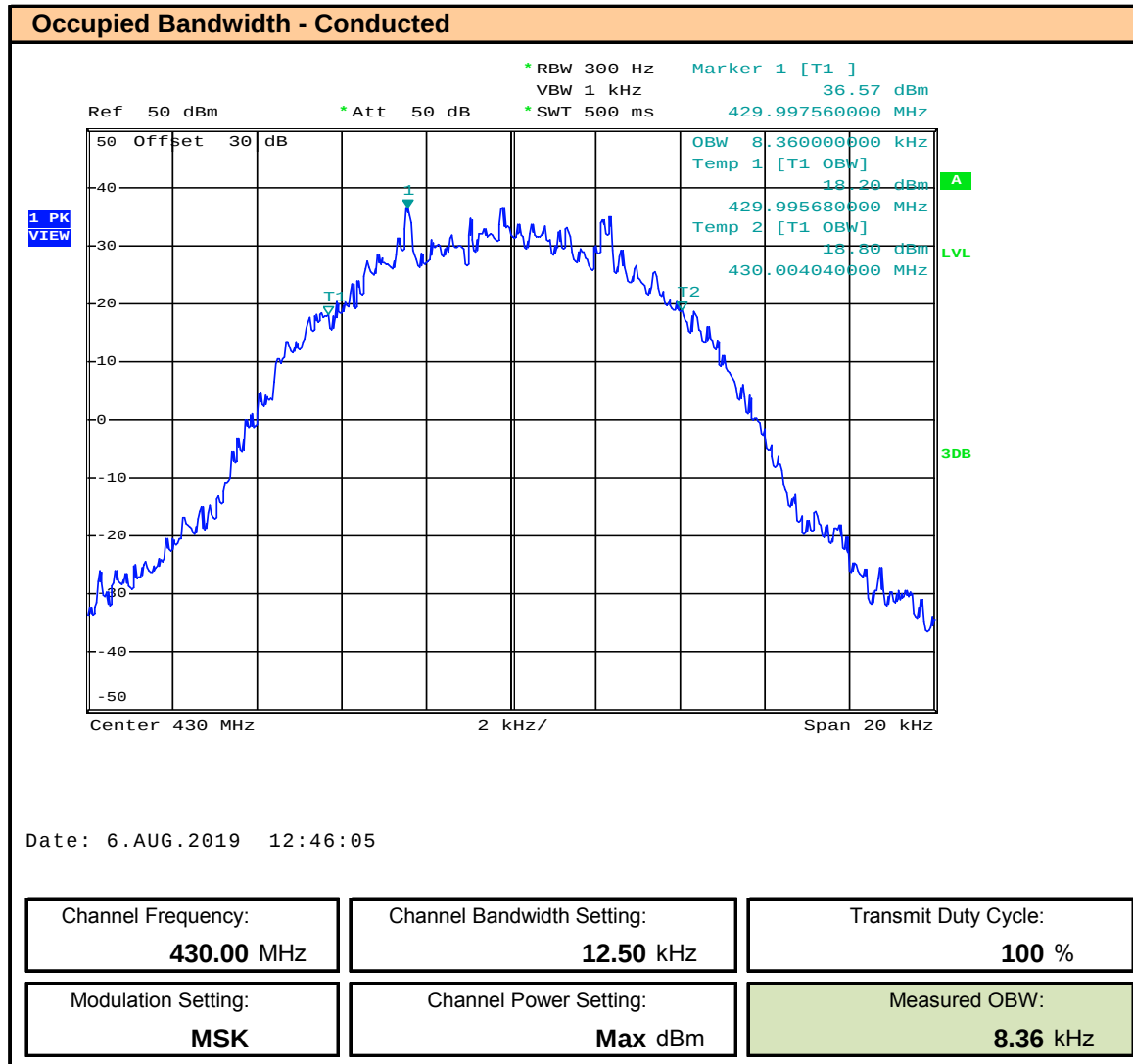
Plot 8.9 – OBW - 12.5kHz BW – MSK – 430MHz , ISED
