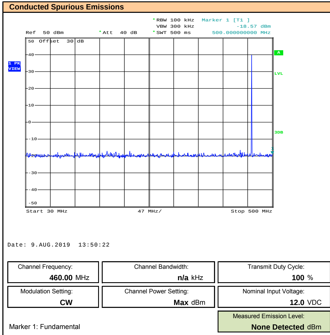
Plot 10.13 – Conducted Spurious Emission, 30MHz – 500MHz, Channel: 460MHz
