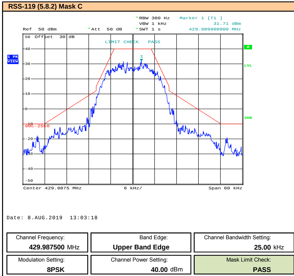
Plot 9.54 – Band Edge and Emissions Mask – 25kHz BW – 8PSK – 429.9875MHz, ISED
