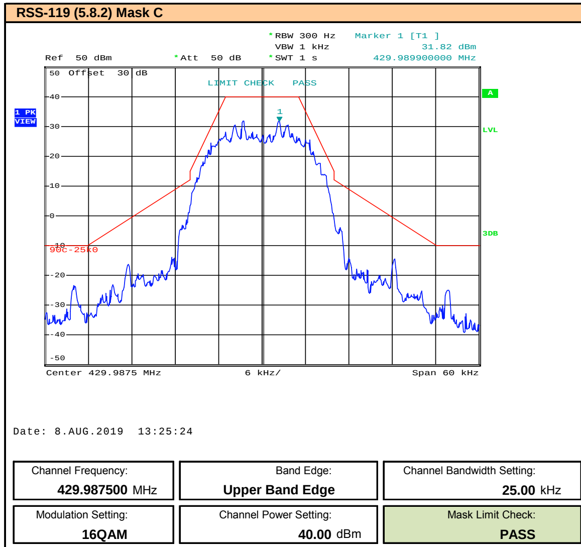
Plot 9.66 – Band Edge and Emissions Mask – 25kHz BW – 16QAM – 429.9875MHz, ISED
