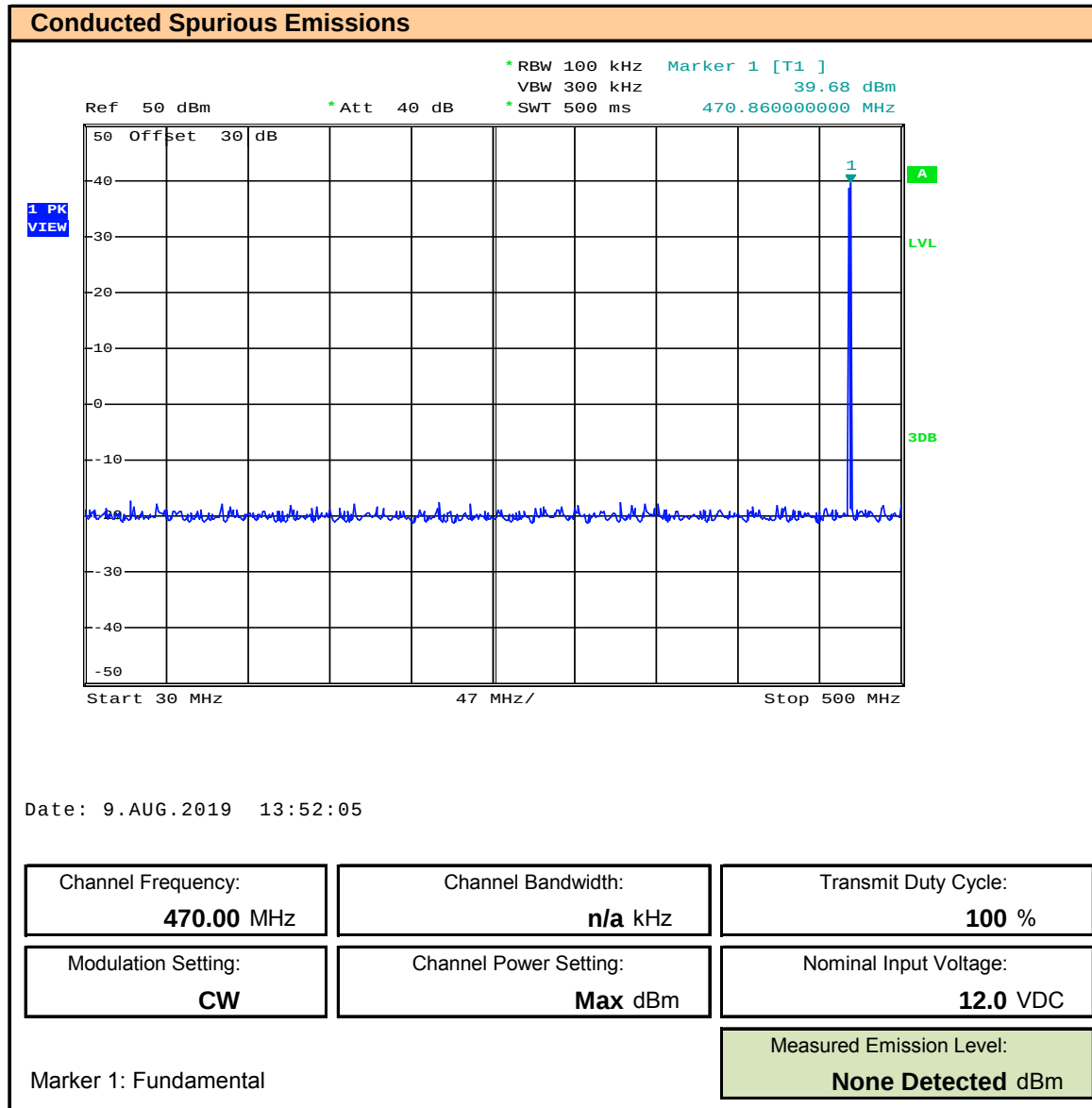
Plot 10.16 – Conducted Spurious Emission, 30MHz – 500MHz, Channel: 470MHz
