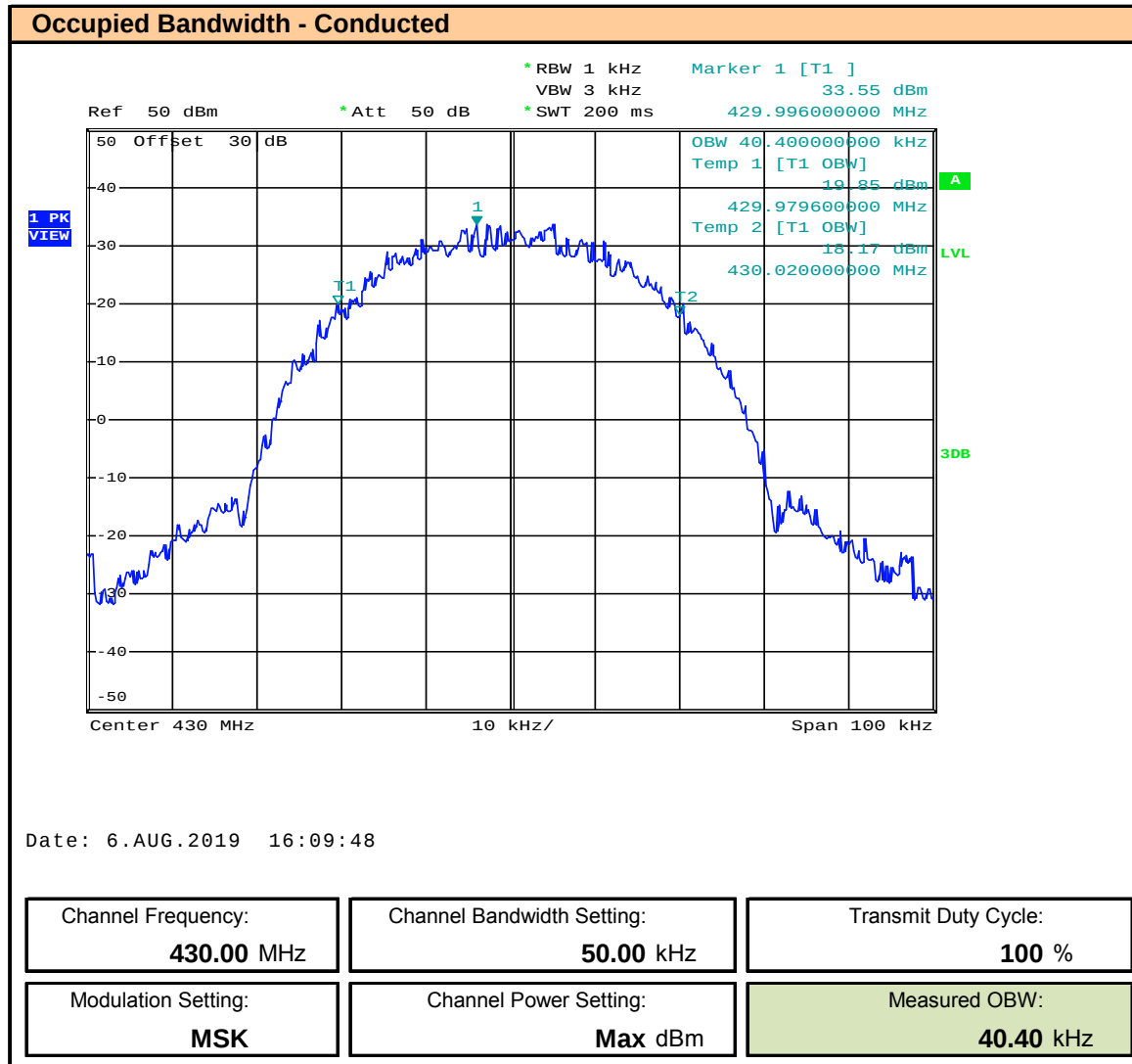
Plot 8.81 – OBW - 50kHz BW – MSK – 430MHz , ISED
