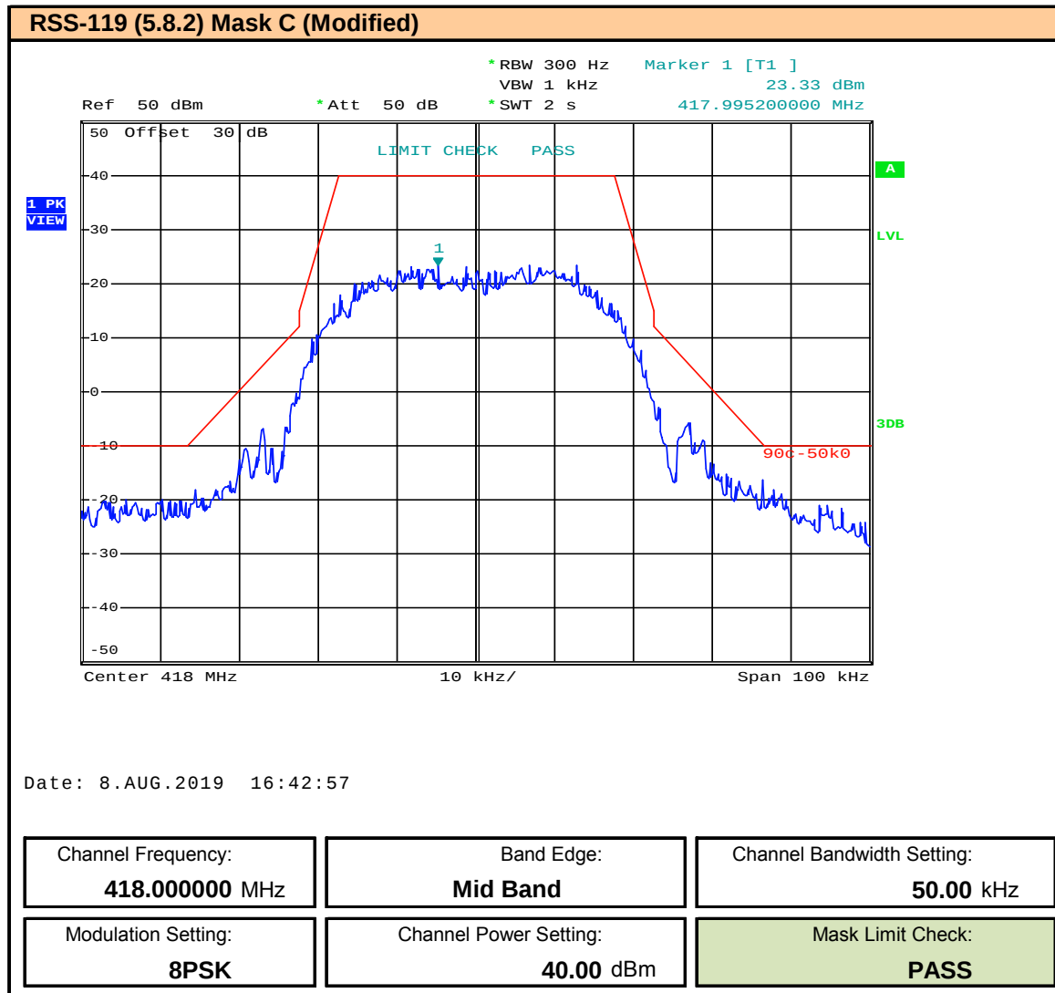
Plot 9.88 – Band Edge and Emissions Mask – 50kHz BW – 8PSK – 418MHz, ISED
