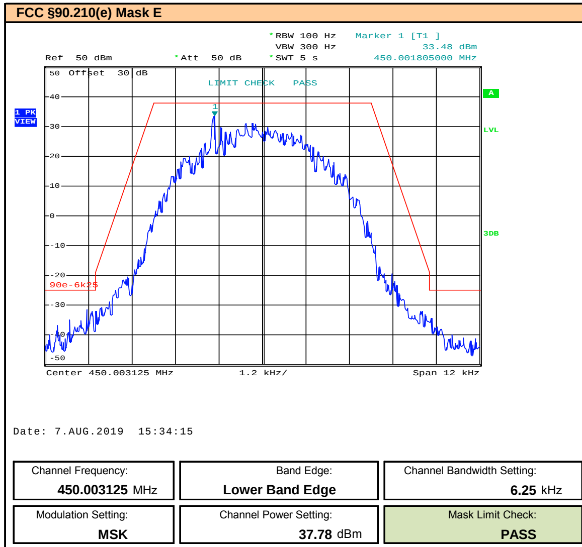
Plot 9.5 – Band Edge and Emissions Mask – 6.25kHz BW – MSK – 450.003125MHz, FCC
