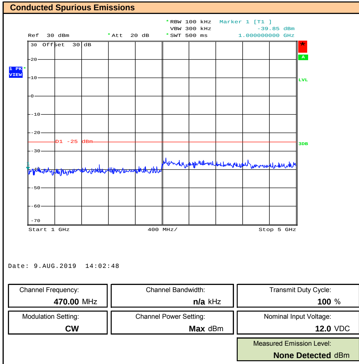
Plot 10.18 – Conducted Spurious Emission, 1 – 5GHz, Channel: 470MHz
