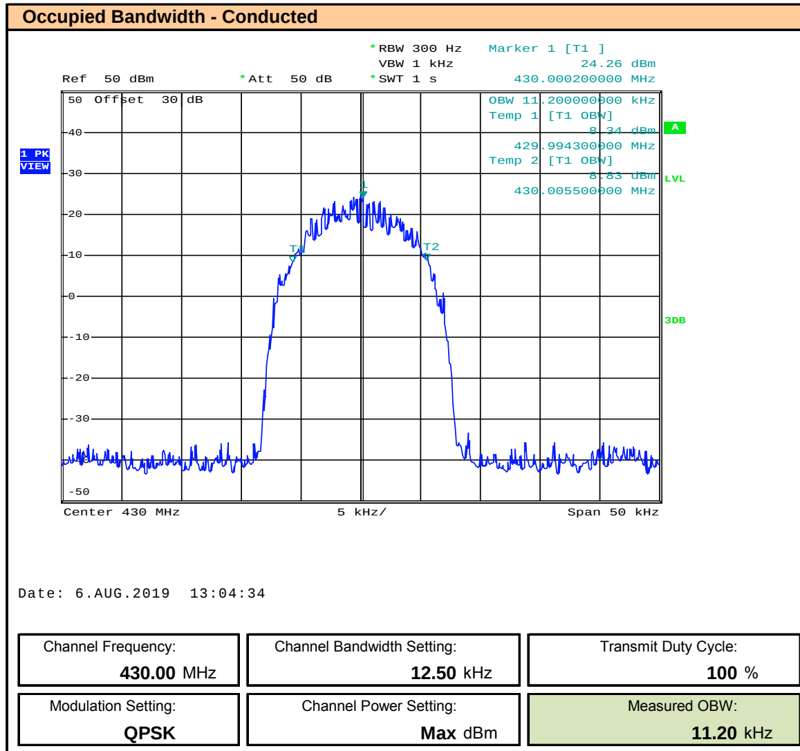
Plot 8.21 – OBW - 12.5kHz BW – QPSK – 430MHz , ISED
