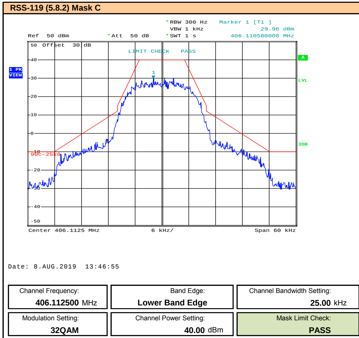
Plot 9.70 – Band Edge and Emissions Mask – 25kHz BW – 32QAM – 406.1125MHz, ISED
