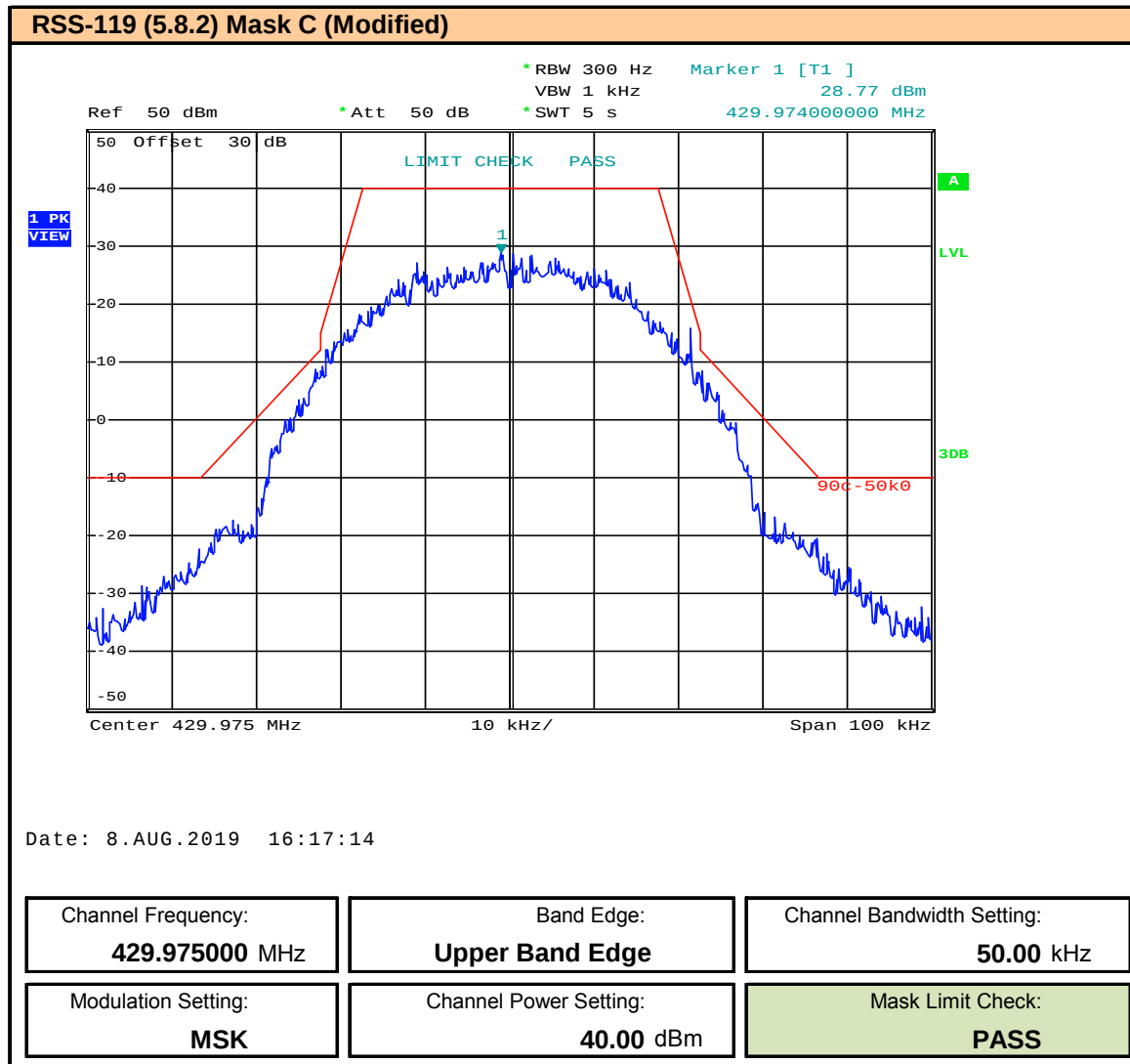
Plot 9.84 – Band Edge and Emissions Mask – 50kHz BW – MSK – 429.975MHz, ISED
