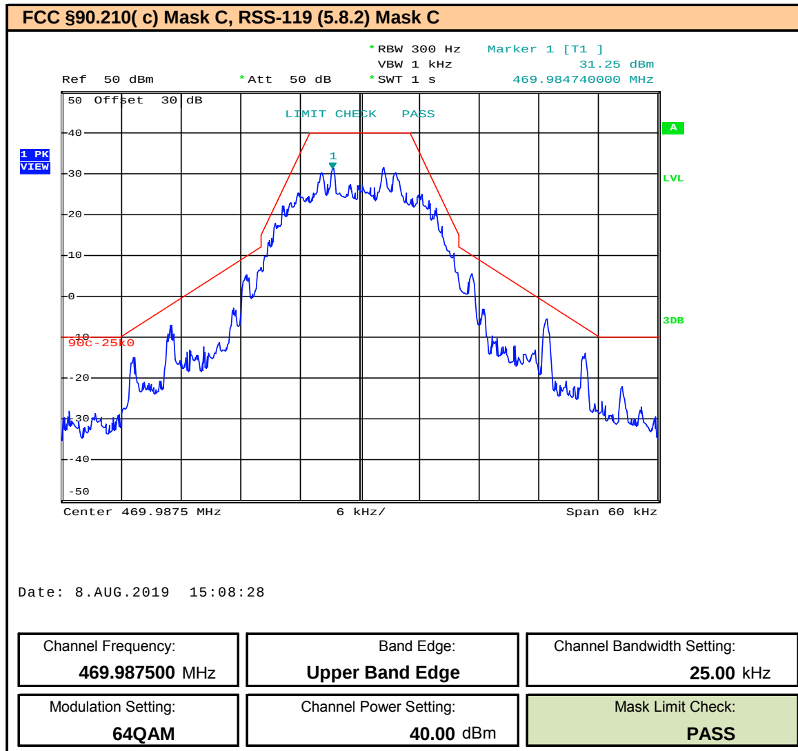
Plot 9.81 – Band Edge and Emissions Mask – 25kHz BW – 64QAM – 469.9875MHz
