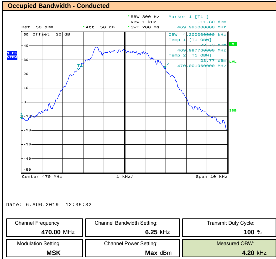
Plot 8.6 – OBW - 6.25kHz BW – MSK - 470MHz
