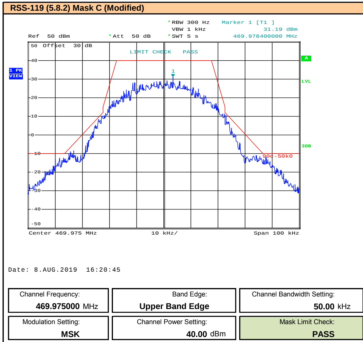
Plot 9.86 – Band Edge and Emissions Mask – 50kHz BW – MSK – 469.975MHz
