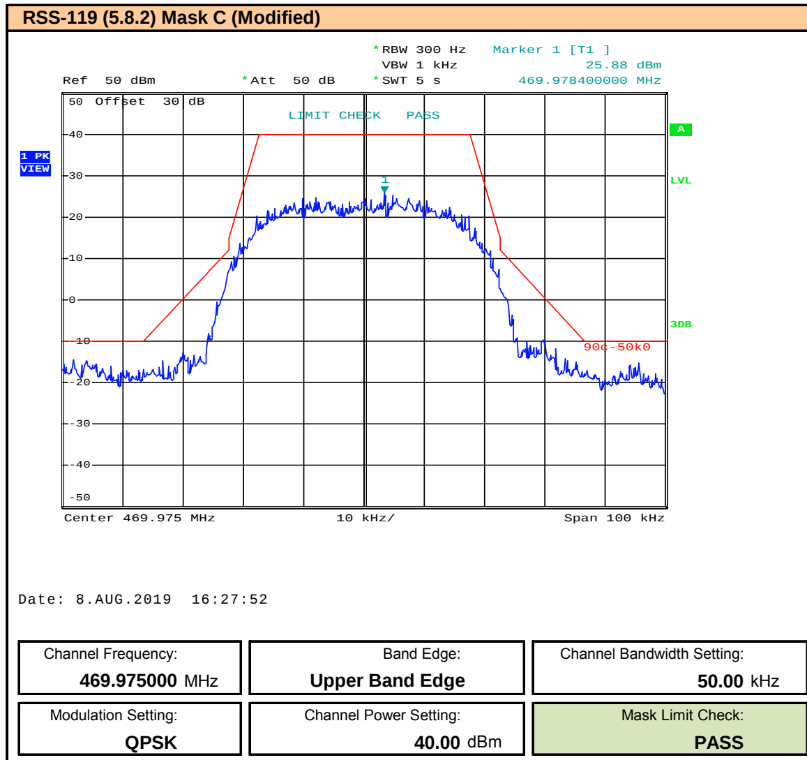
Plot 9.98 – Band Edge and Emissions Mask – 50kHz BW – QPSK – 469.975MHz
