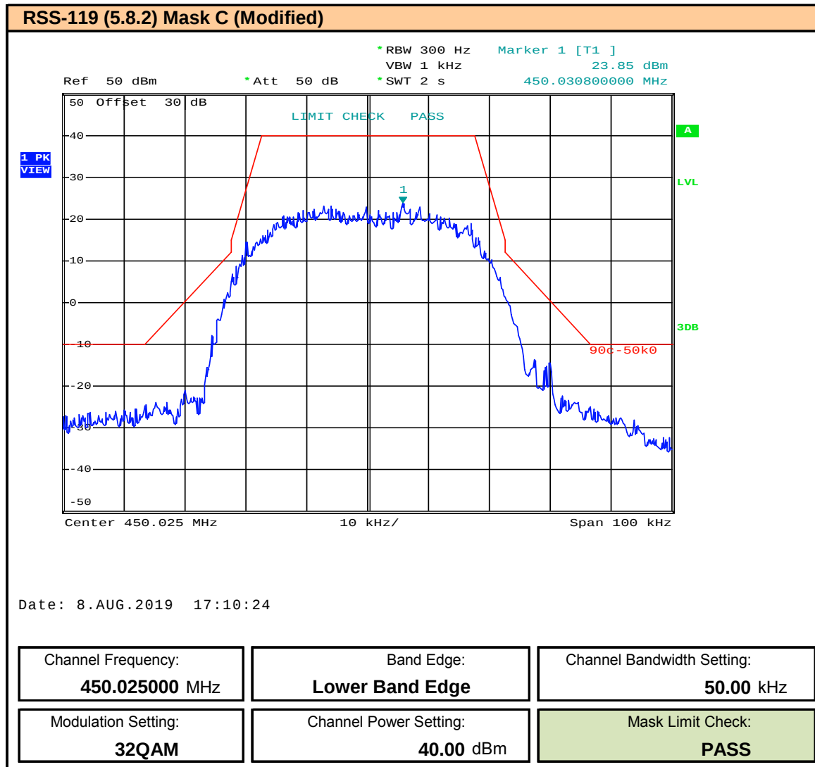
Plot 9.108 – Band Edge and Emissions Mask – 50kHz BW – 32QAM – 450.025MHz
