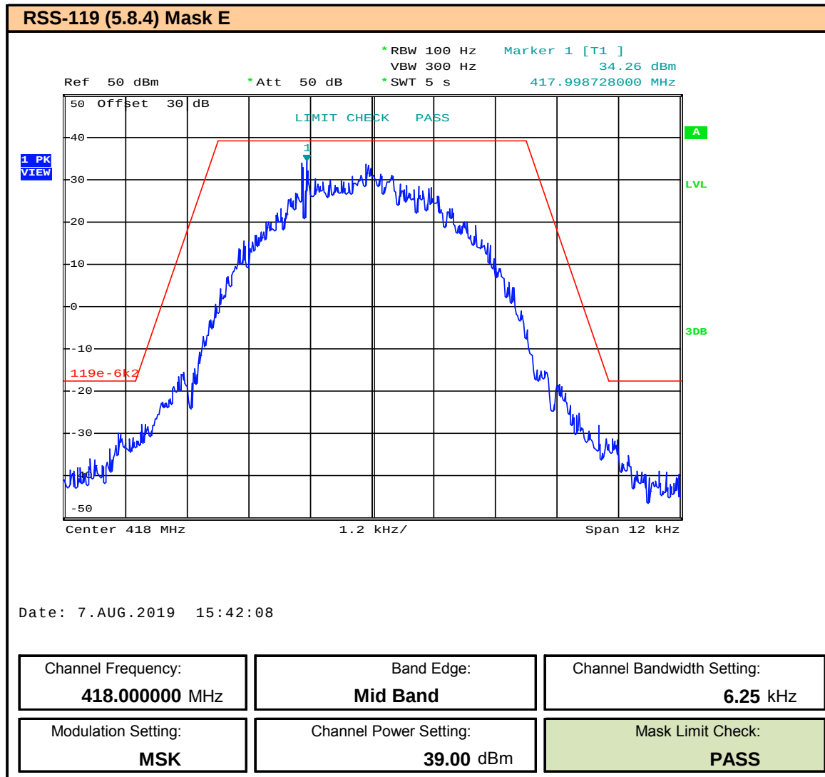
Plot 9.2 – Band Edge and Emissions Mask – 6.25kHz BW – MSK – 418MHz, ISED
