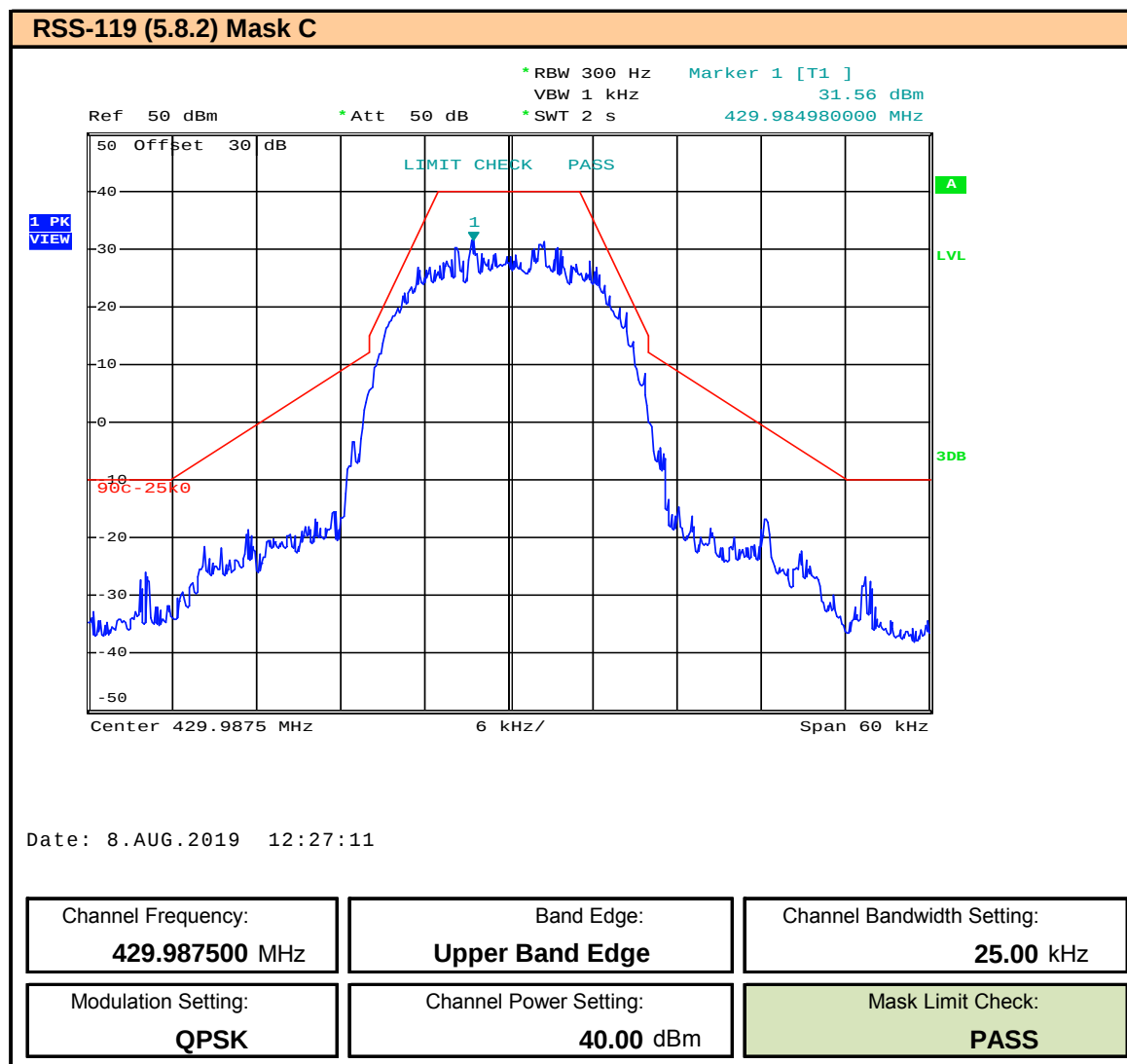
Plot 9.60 – Band Edge and Emissions Mask – 25kHz BW – QPSK – 429.9875MHz, ISED
