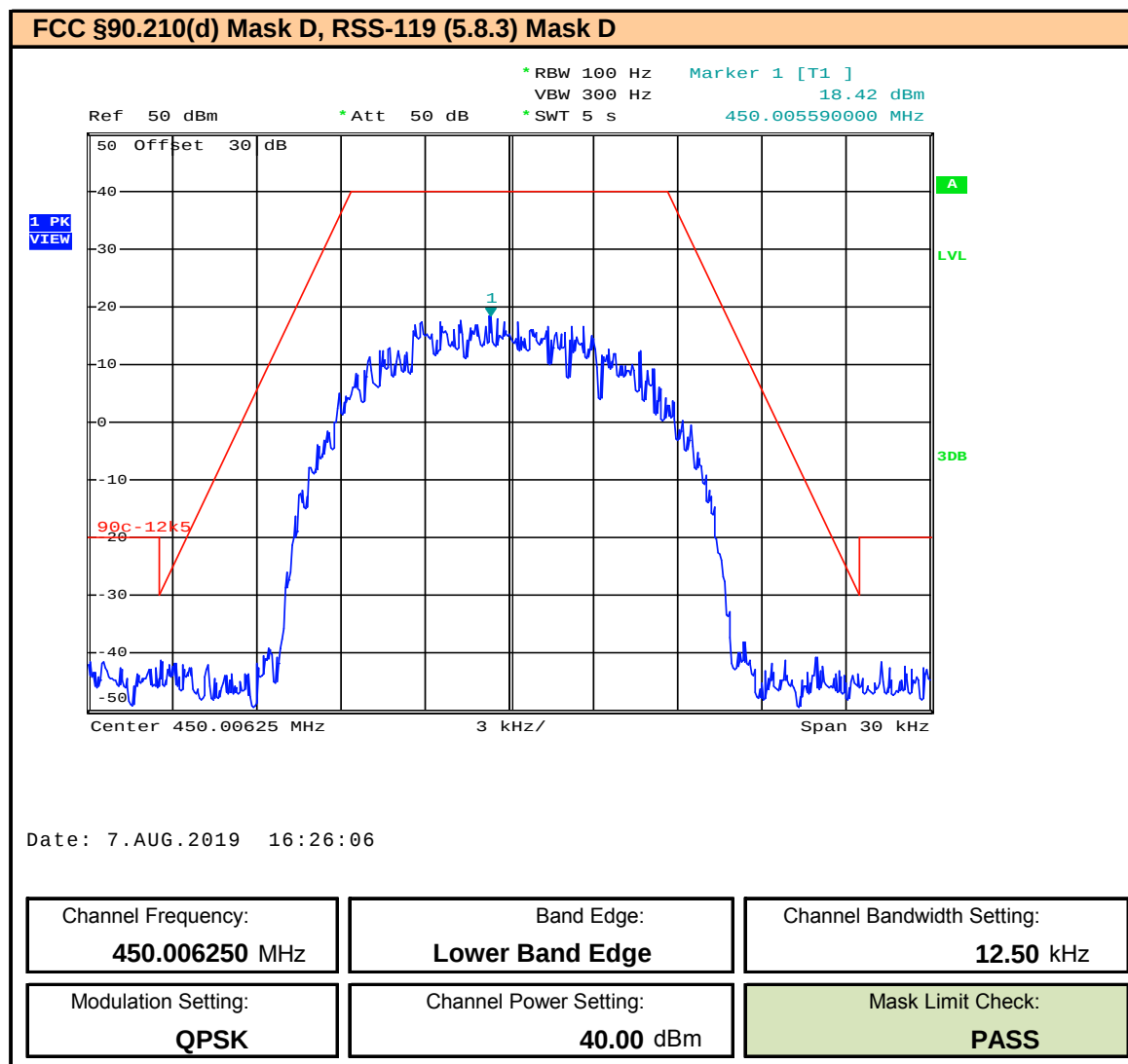
Plot 9.25 – Band Edge and Emissions Mask – 12.5kHz BW – QPSK – 450.00625MHz
