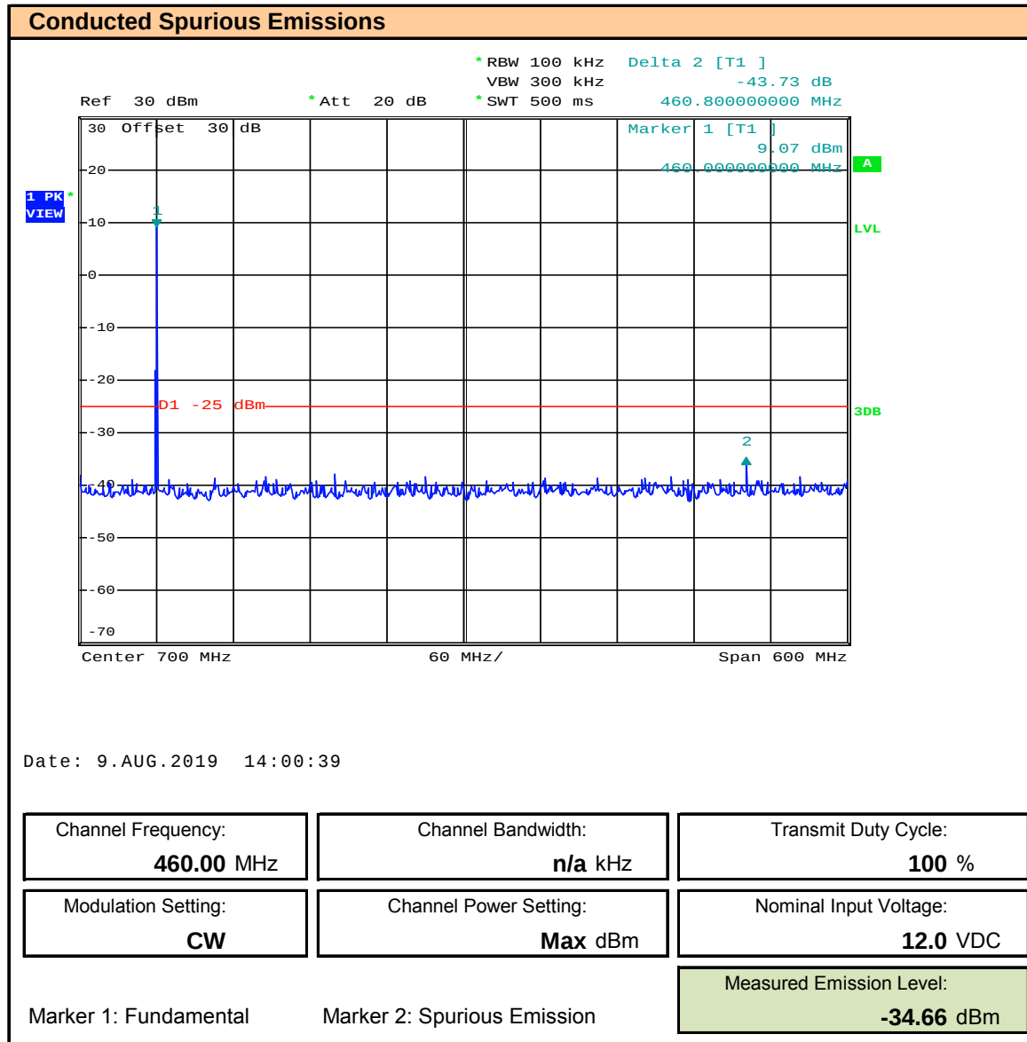
Plot 10.14 – Conducted Spurious Emission, 400MHz – 1000MHz, Channel: 460MHz
