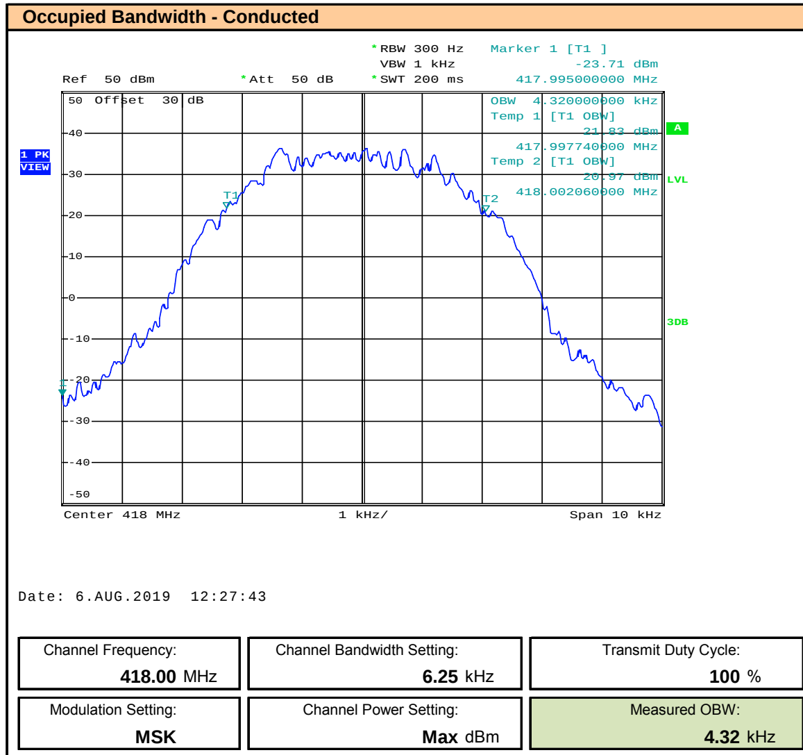
Plot 8.2 – OBW - 6.25kHz BW – MSK - 418MHz , ISED
