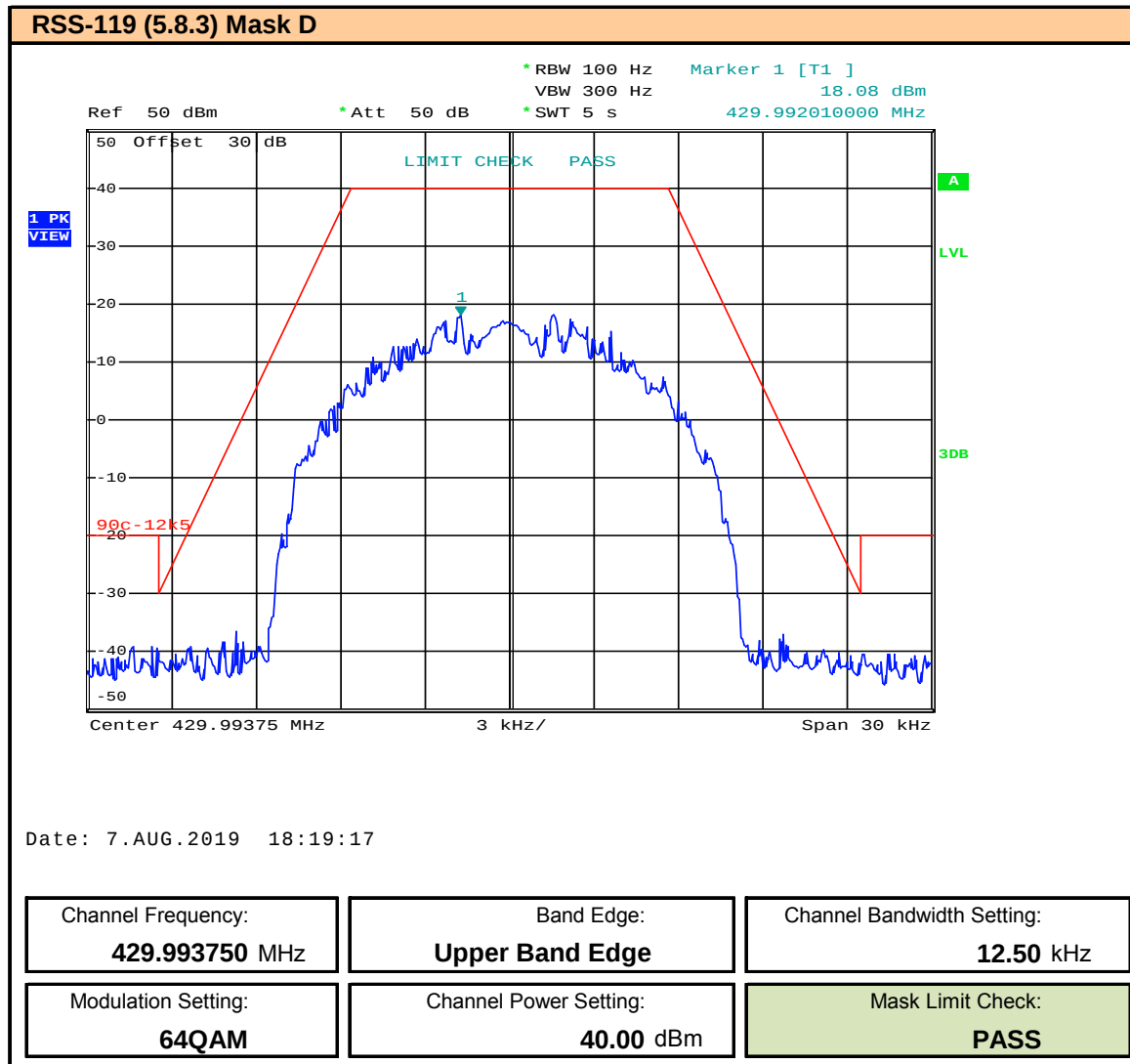
Plot 9.42 – Band Edge and Emissions Mask – 12.5kHz BW – 64QAM – 429.99375MHz, ISED
