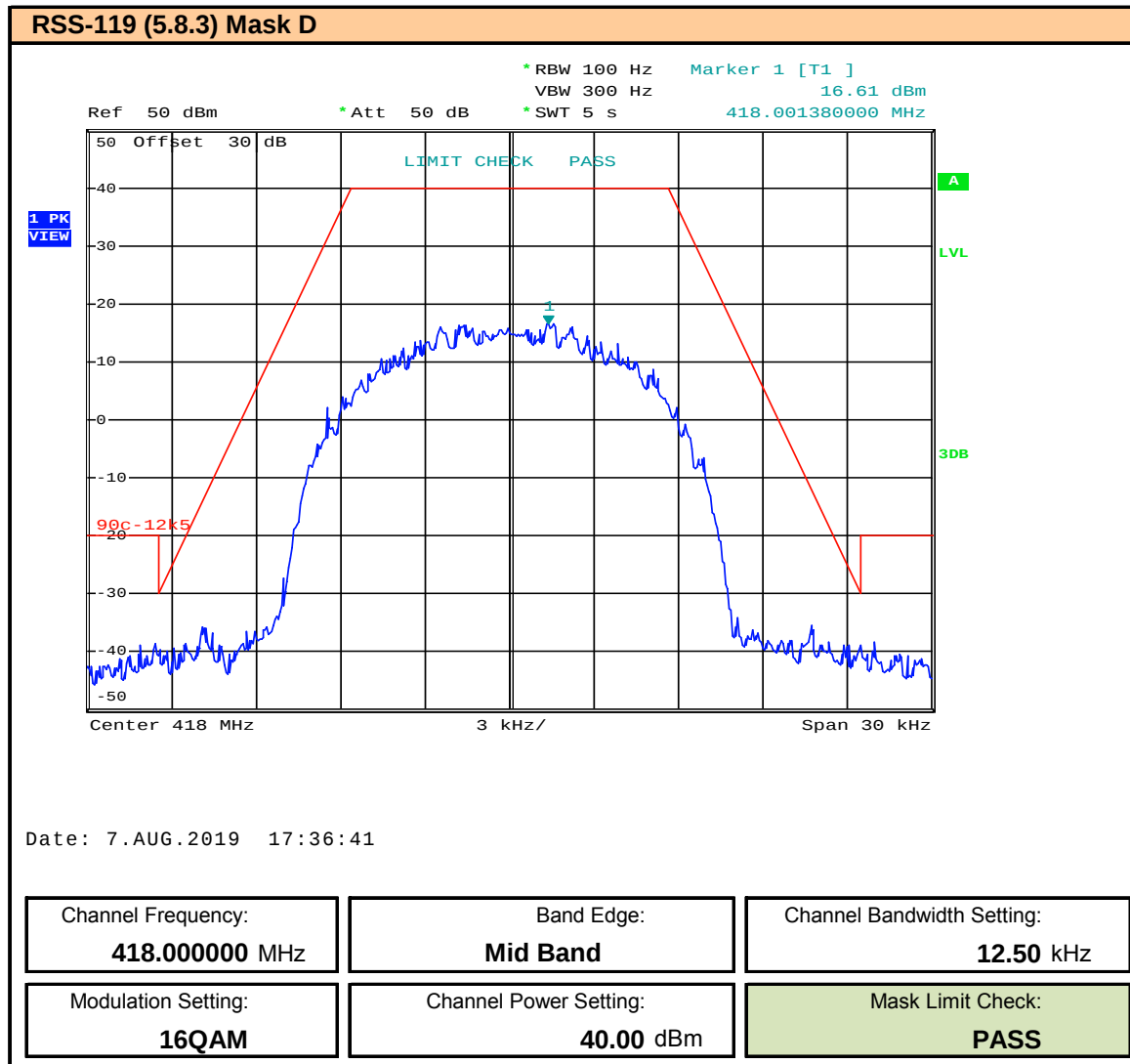
Plot 9.29 – Band Edge and Emissions Mask – 12.5kHz BW – 16QAM – 418MHz, ISED
