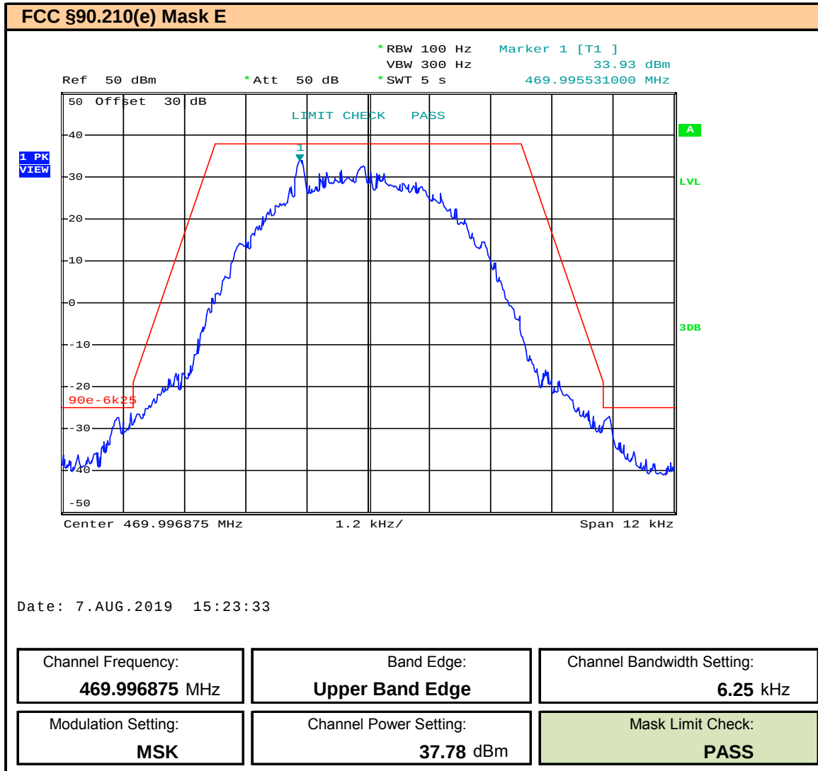
Plot 9.9 – Band Edge and Emissions Mask – 6.25kHz BW – MSK – 469.996875MHz, FCC
