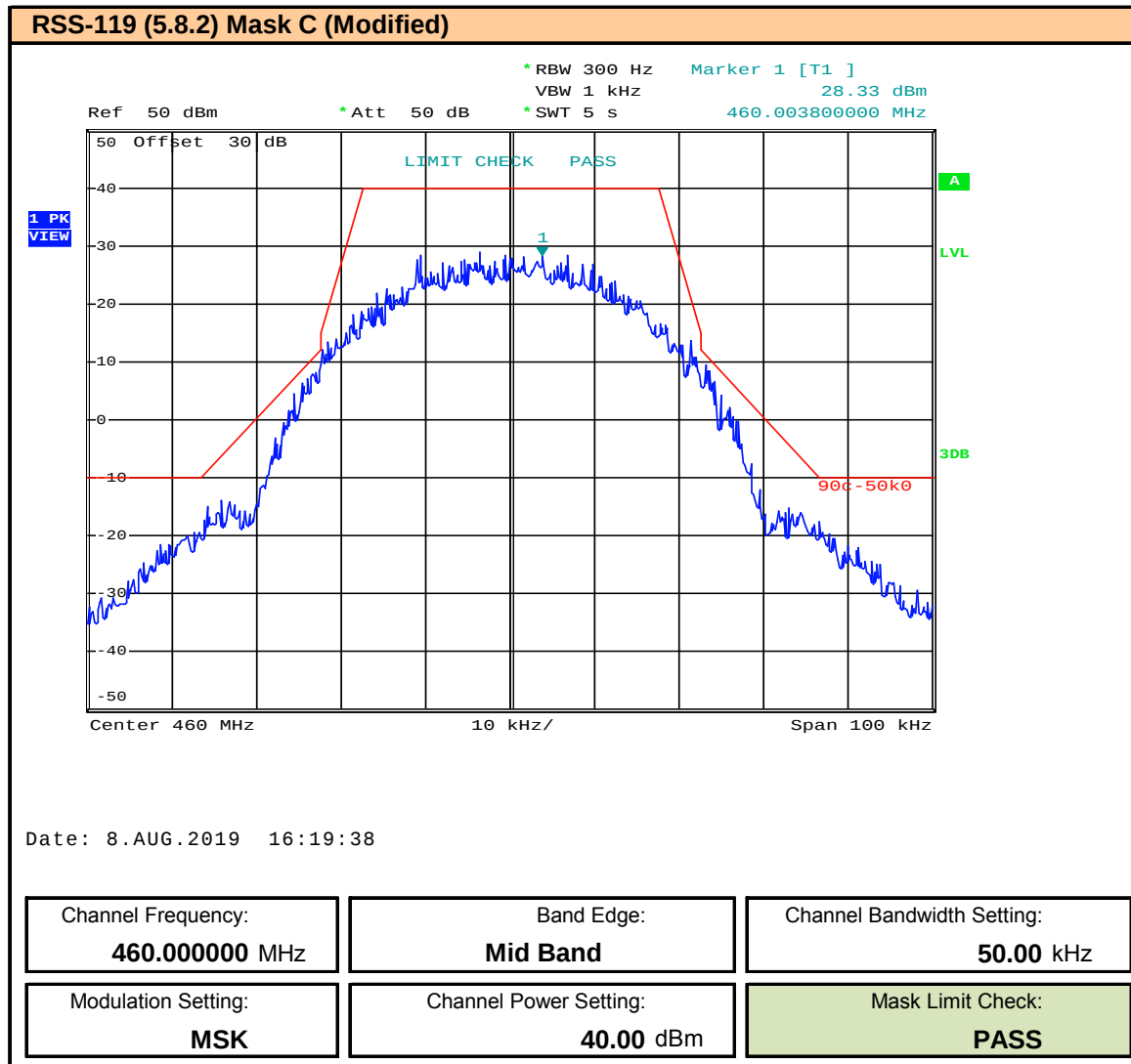
Plot 9.86 – Band Edge and Emissions Mask – 50kHz BW – MSK – 460MHz
