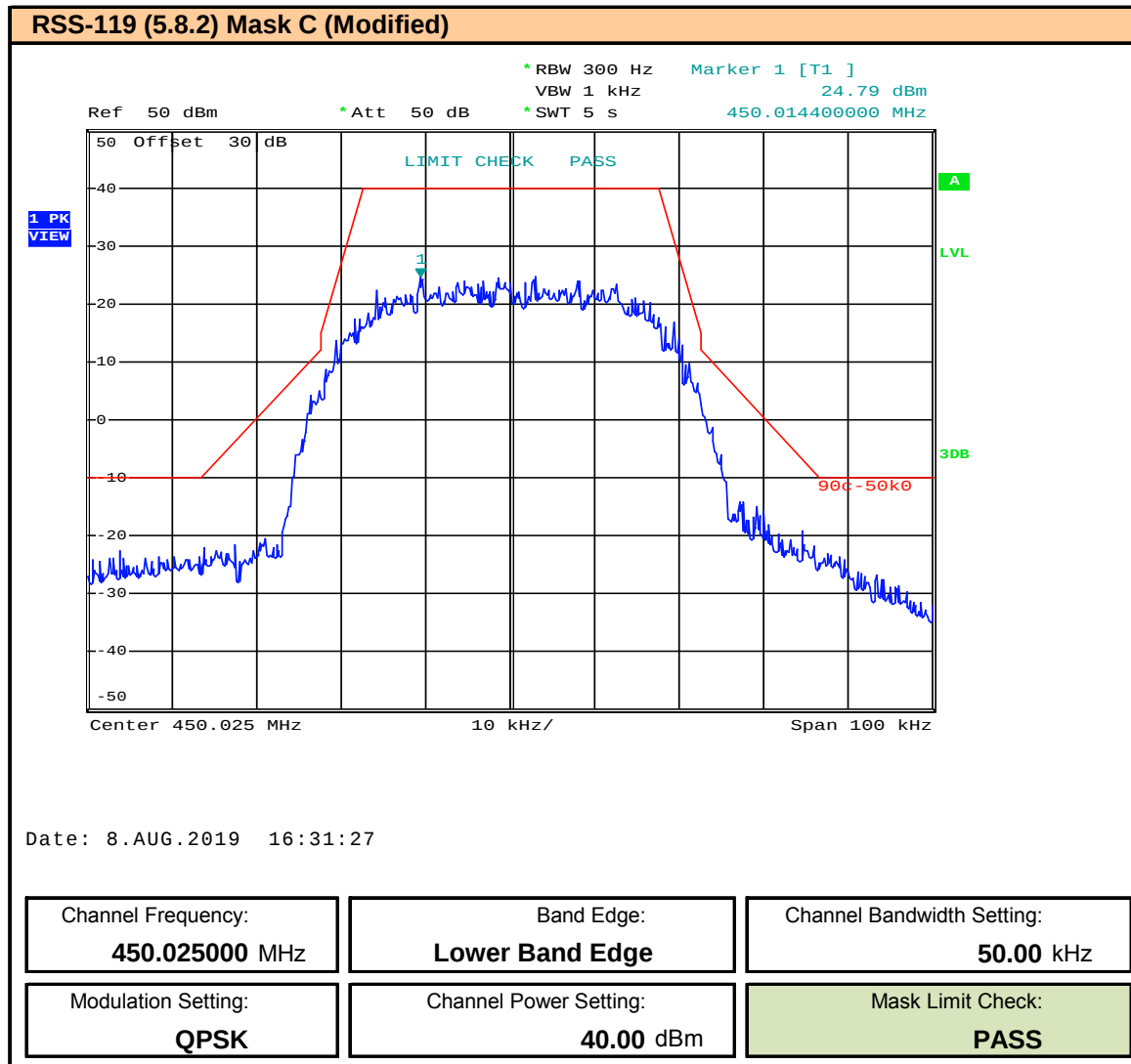
Plot 9.96 – Band Edge and Emissions Mask – 50kHz BW – QPSK – 450.025MHz
