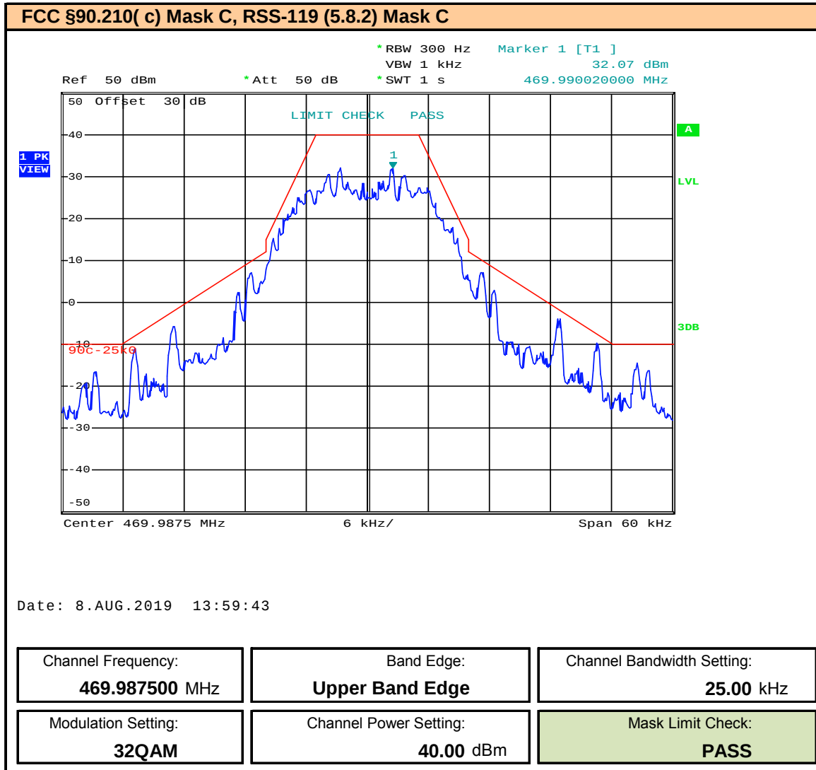
Plot 9.75 – Band Edge and Emissions Mask – 25kHz BW – 32QAM – 469.9875MHz
