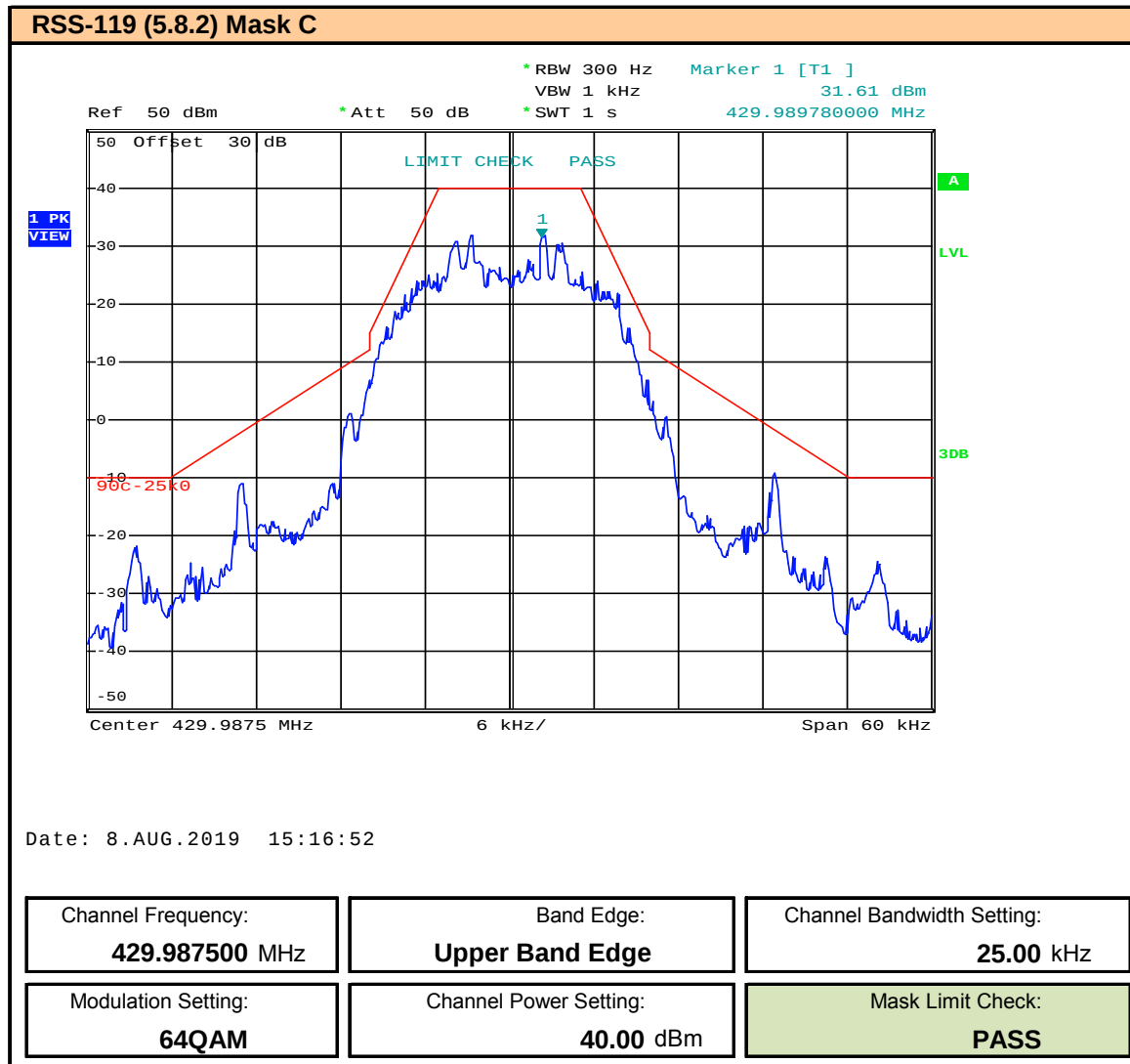
Plot 9.78 – Band Edge and Emissions Mask – 25kHz BW – 64QAM – 429.9875MHz, ISED
