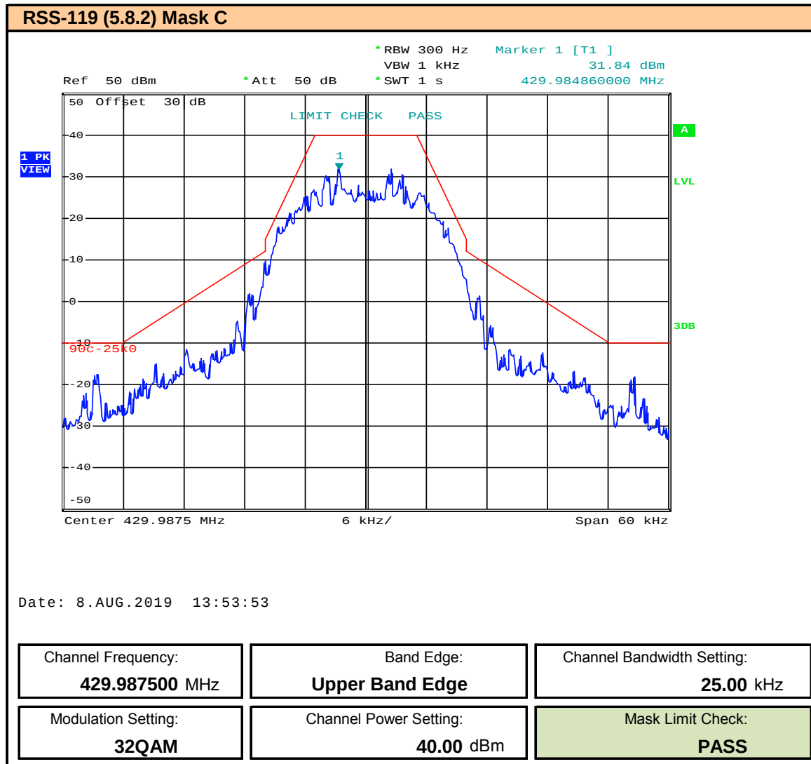
Plot 9.72 – Band Edge and Emissions Mask – 25kHz BW – 32QAM – 429.9875MHz, ISED
