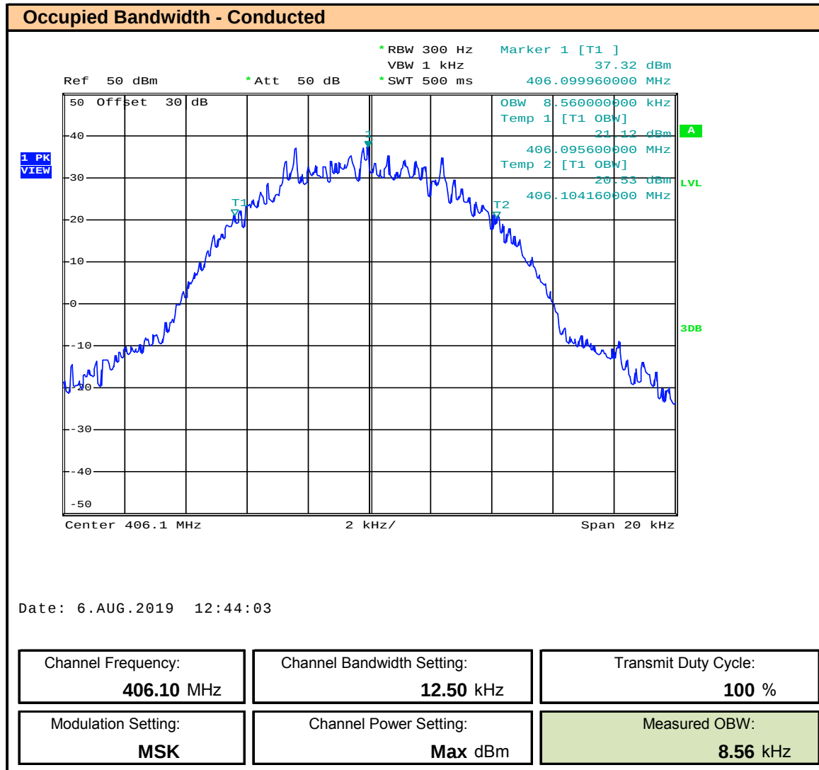
Plot 8.7 – OBW - 12.5kHz BW – MSK – 406.1MHz , ISED
