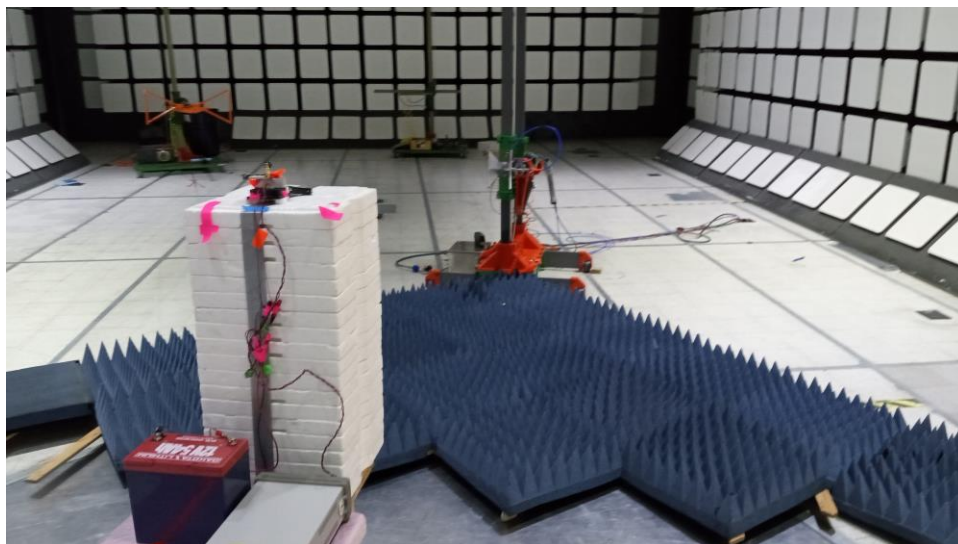
1 – 18 GHz Test Setup
