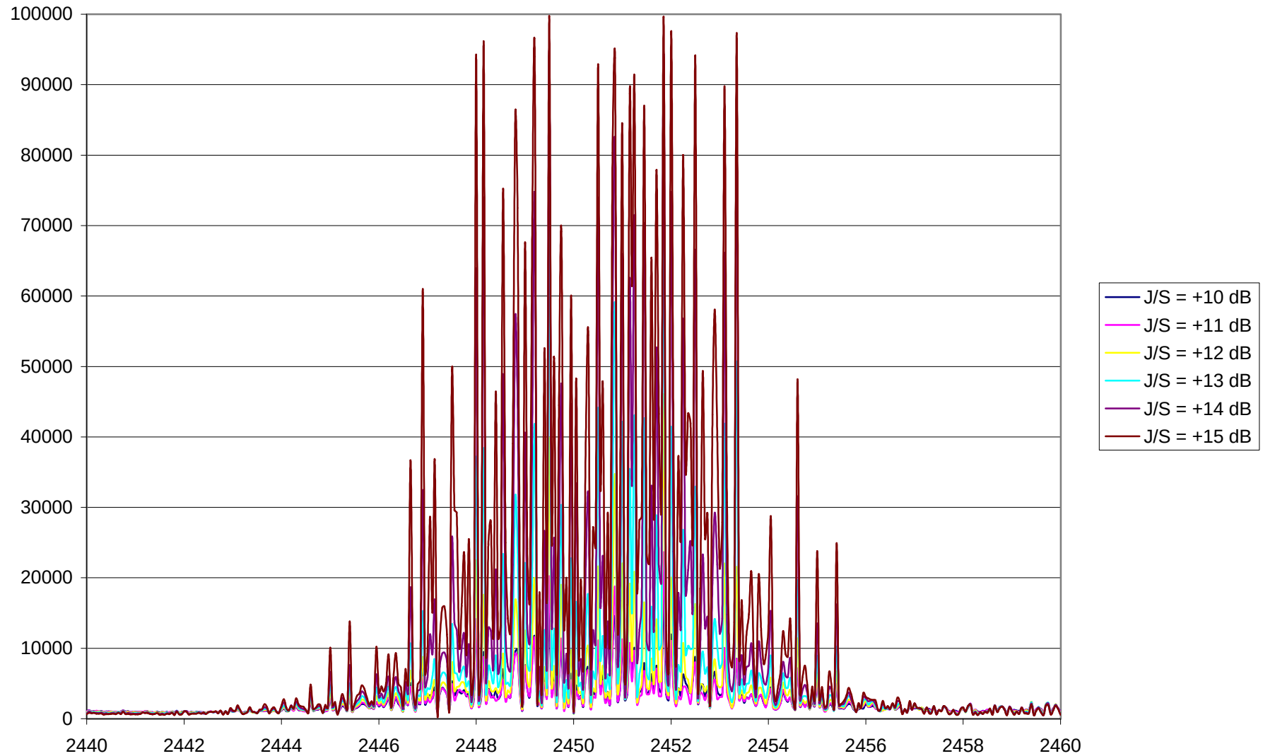
SAM019 Receiver BER - Errors per 100,000 bits (Combined DSSS Input & Jammer Input)
