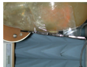
Fig. 9 Head SAR Test Setup
