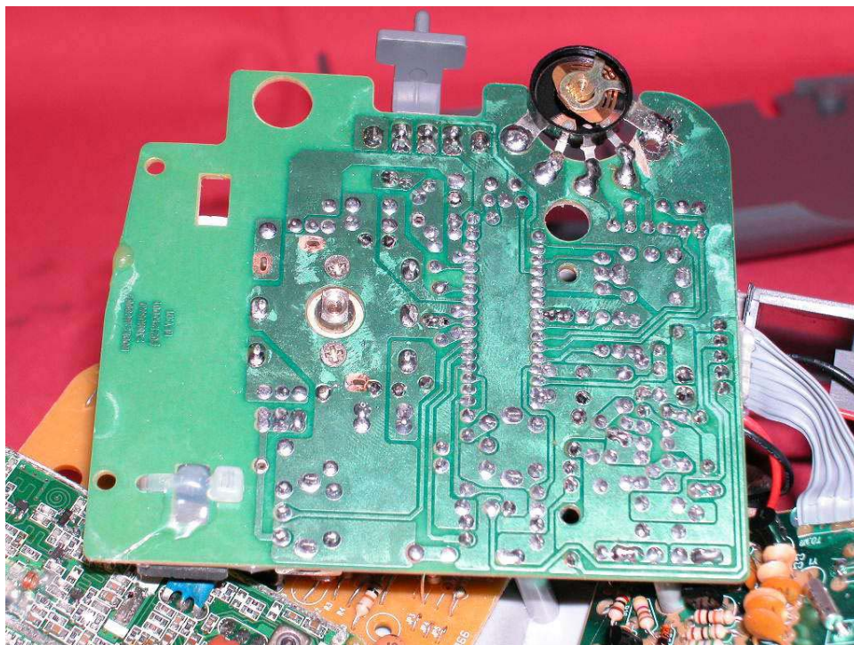
Radio Clock PCB solder side (view 2)
