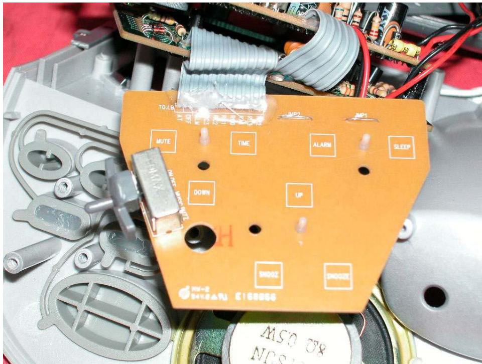
Base PCB keypad rear side
