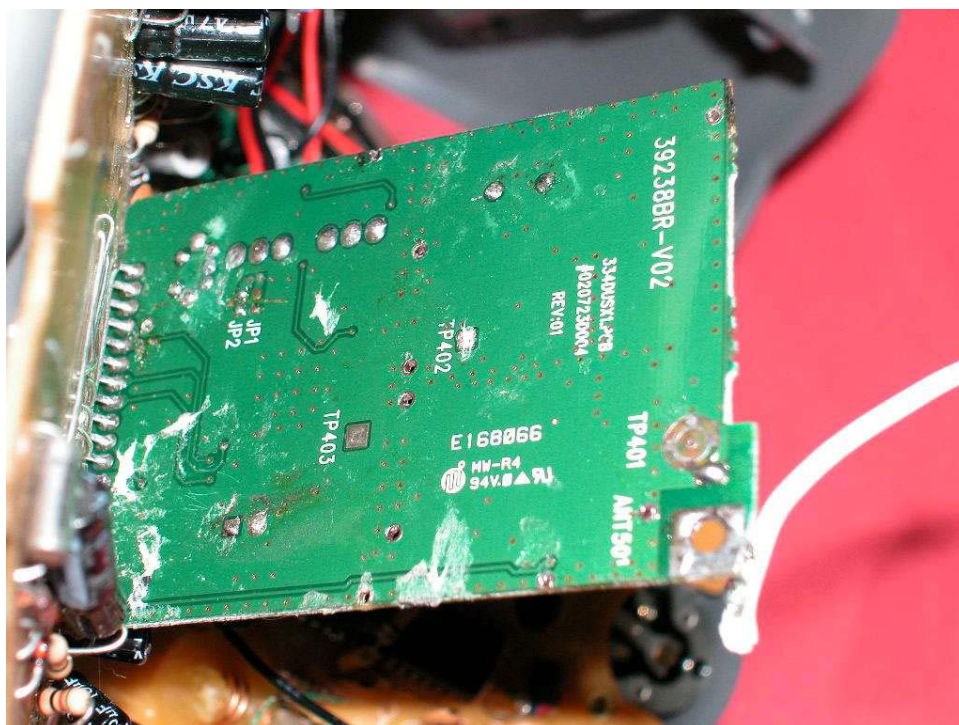
Base Oscillator PCB solder side (view 2)
