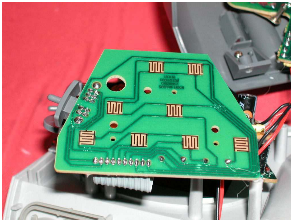
Base PCB keypad front side
