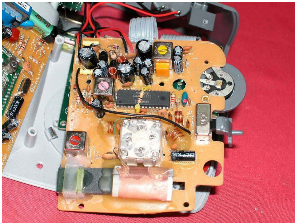
Radio Clock PCB comp side
