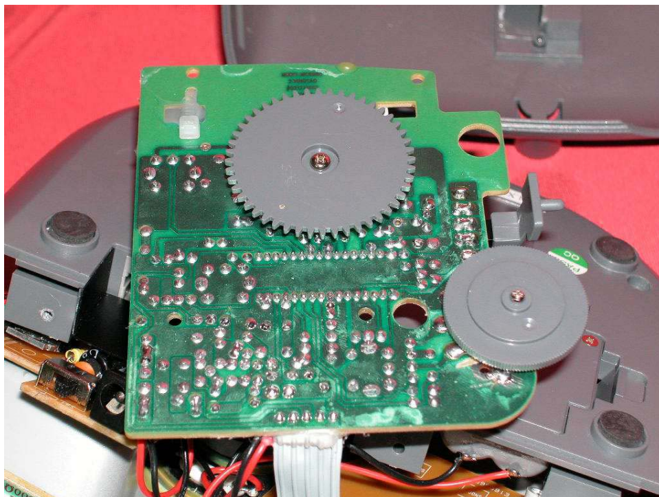
Radio Clock PCB solder side (view 1)
