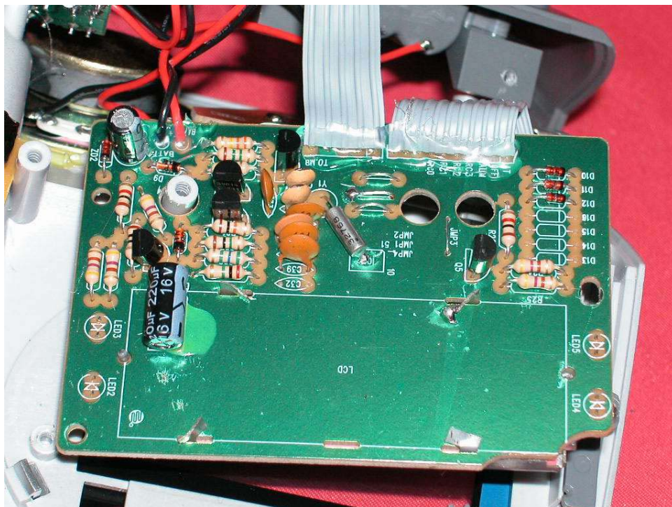
Base LCD display comp side
