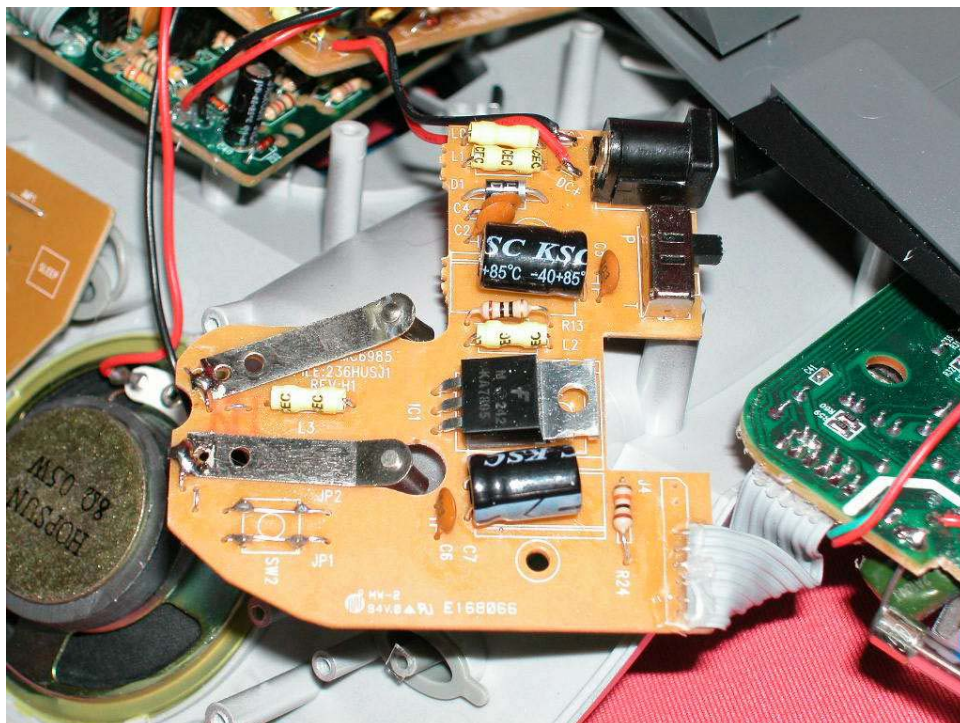
Jack board PCB comp side
