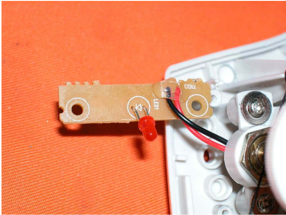
Base PCB LED front side
