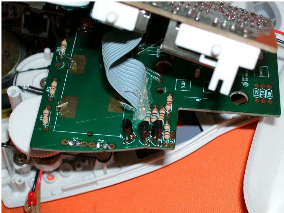
LCD display solder side (View 2)
