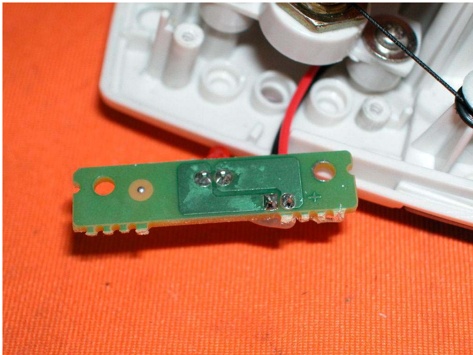
Base PCB LED rear side
