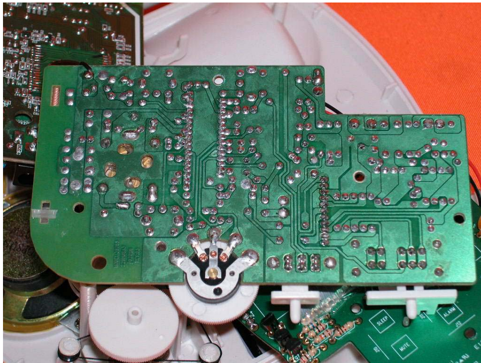
Radio Clock PCB solder side
