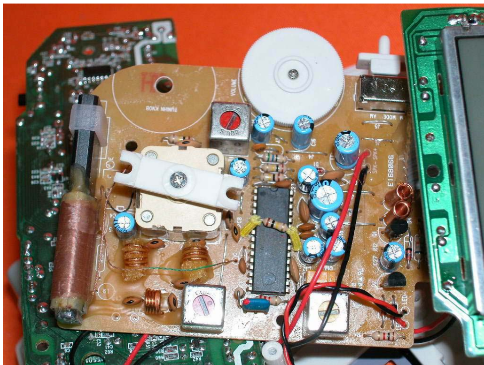
Radio Clock PCB comp side (View 1)
