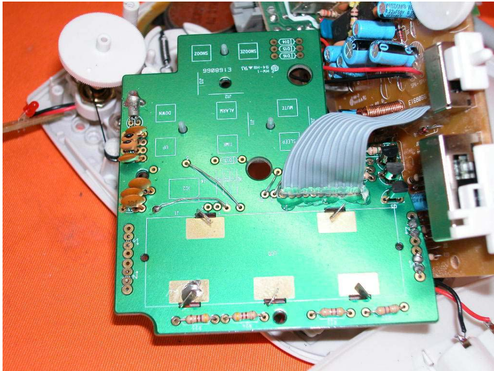
LCD display solder side (View 1)
