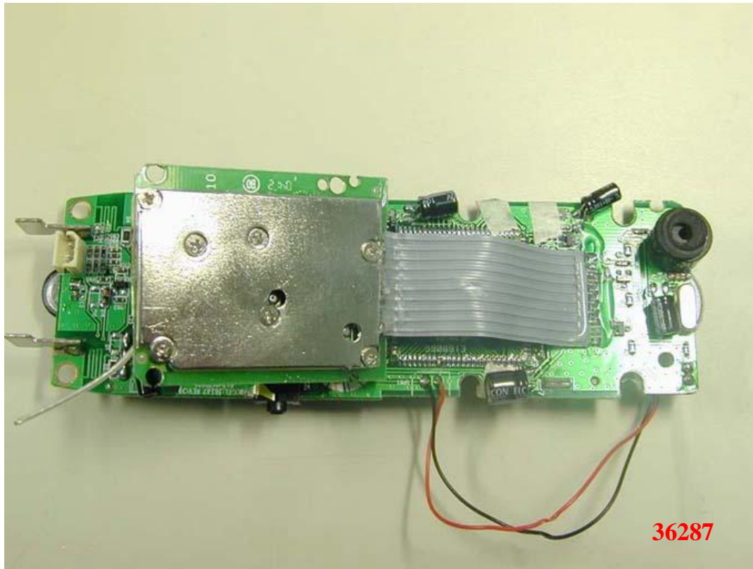
Photo 4: Internal photo of EUT (Handset)
