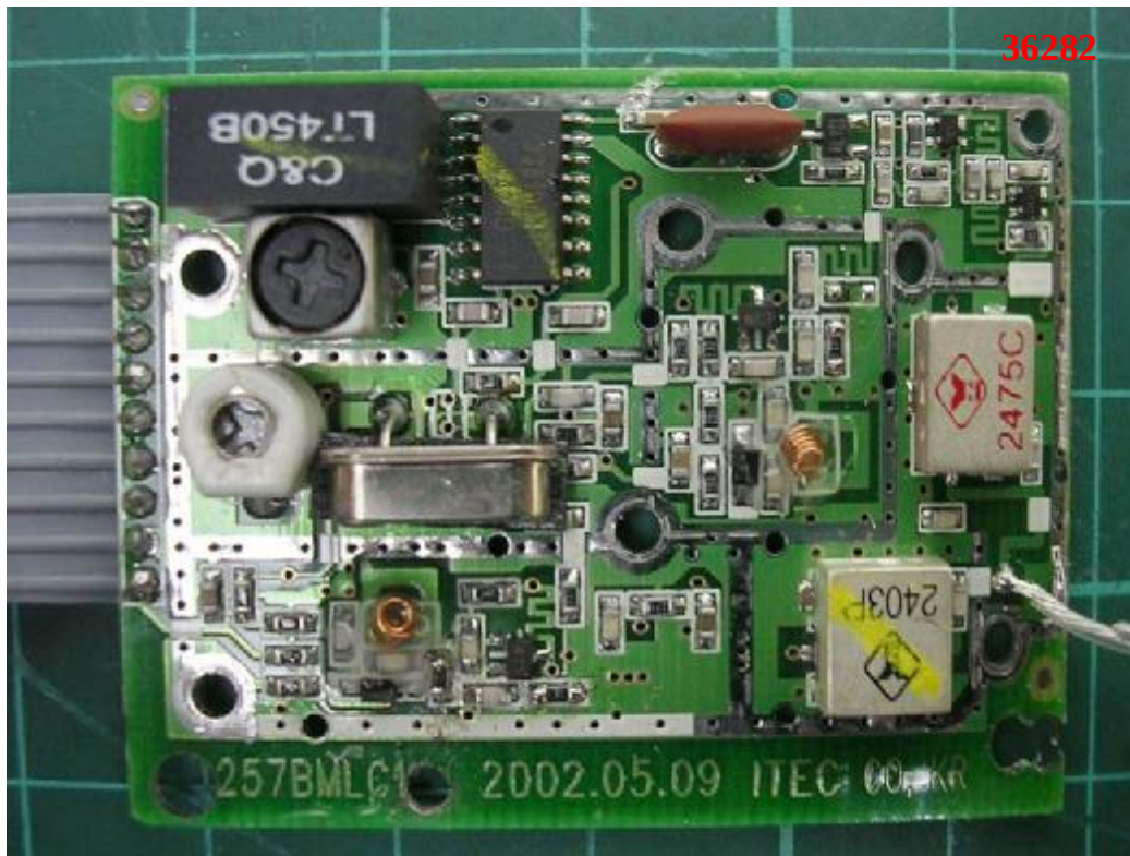
Photo 12: Internal photo of EUT
