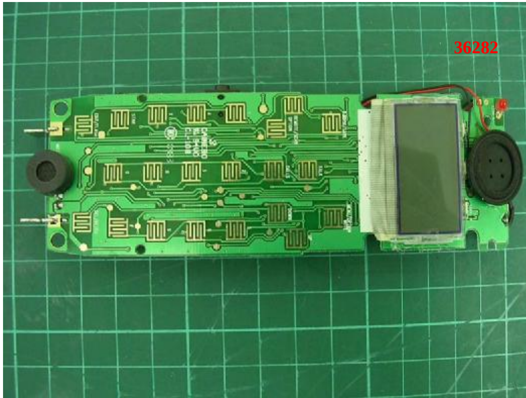
Photo 1: Internal photo of EUT
