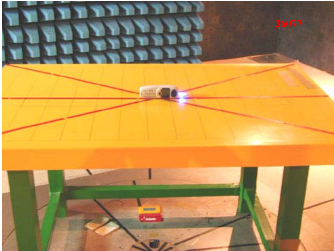
Photo 3: Radiated Emission Test Set-up photo (Handset)
