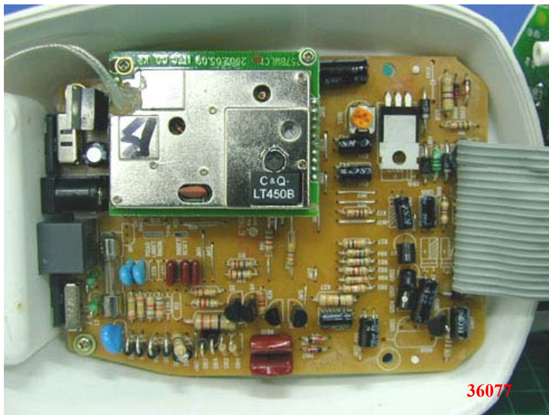
Photo 1: Internal photo of EUT (Base)
