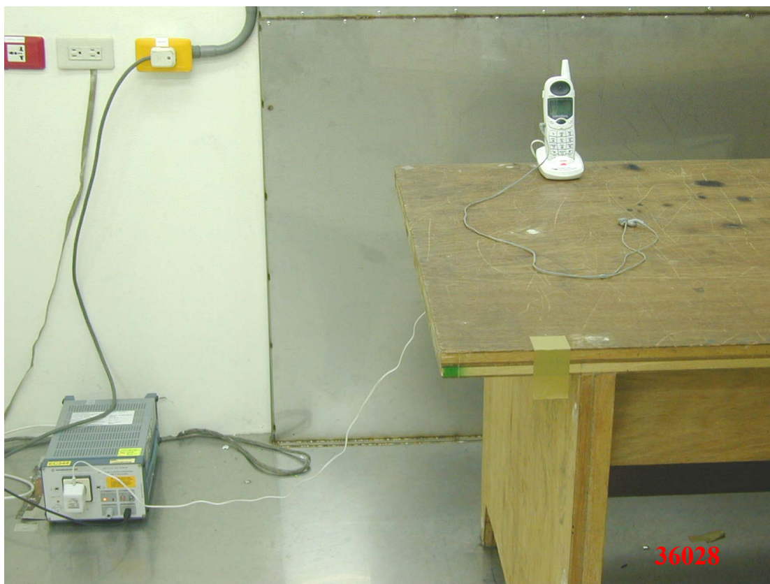
Photo 3: Conducted Emission Test Set-up photo (Handset with Charge)
